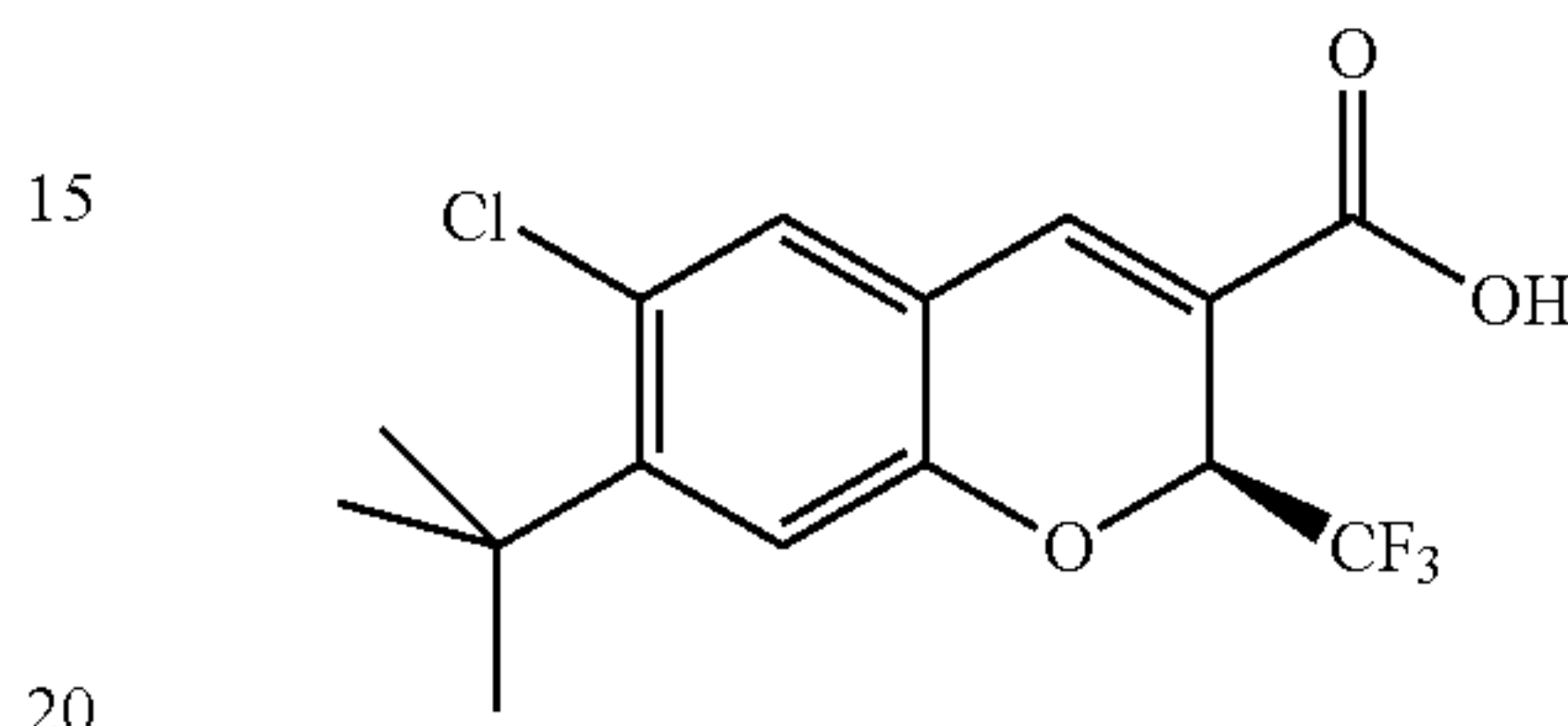
((S)-6-Chloro-7-(1,1-dimethylethyl)-2-(trifluoromethyl)-2H-1-benzopyran-3-carboxylic acid
