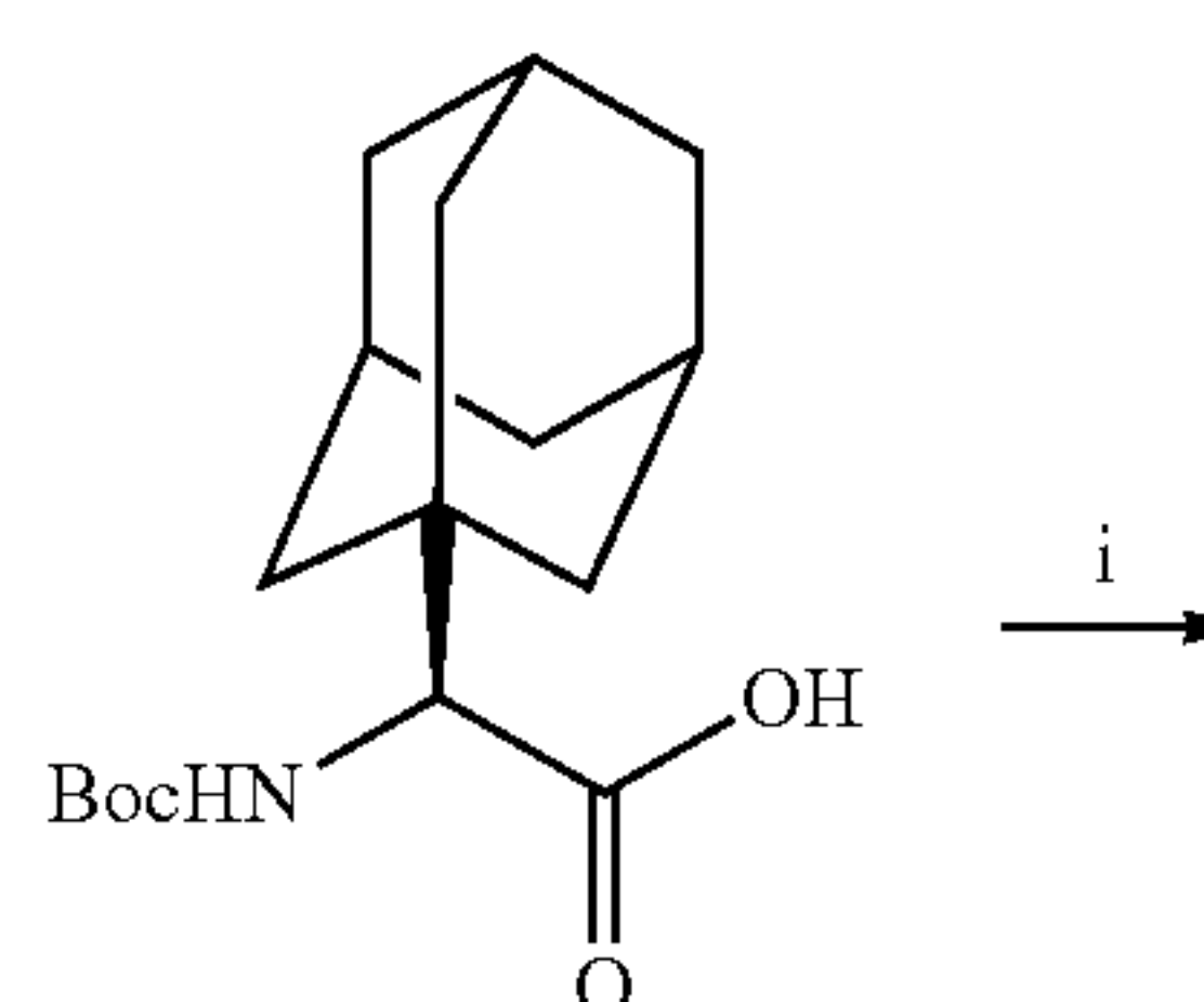
Scheme 2. Synthetic method for ARI-5544 a
