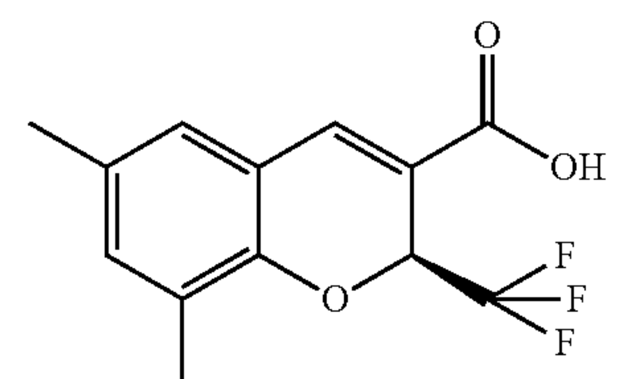
(SS)-6-Chloro-1,2-dihydro-2-(trifluoromethyl)-3-quinolinecarboxylic acid
