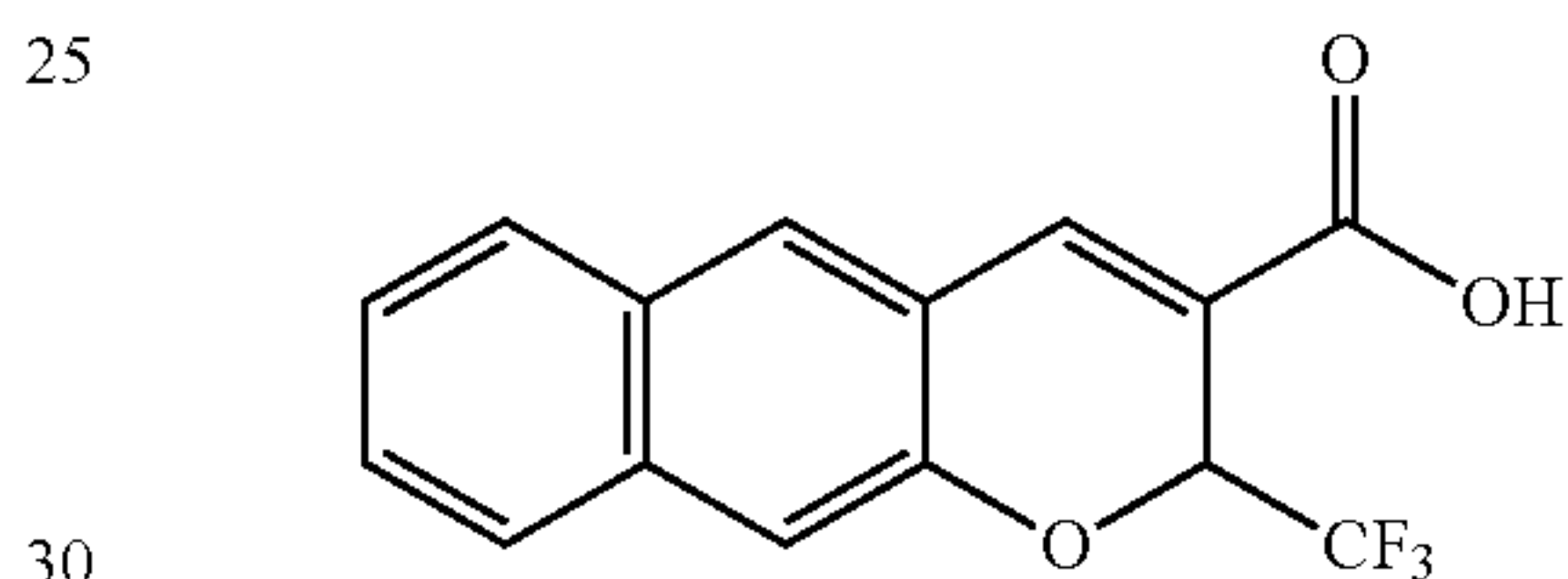
2-Trifluoromethyl-2H-naphtho[2,3-b]pyran-3-carboxylic acid
