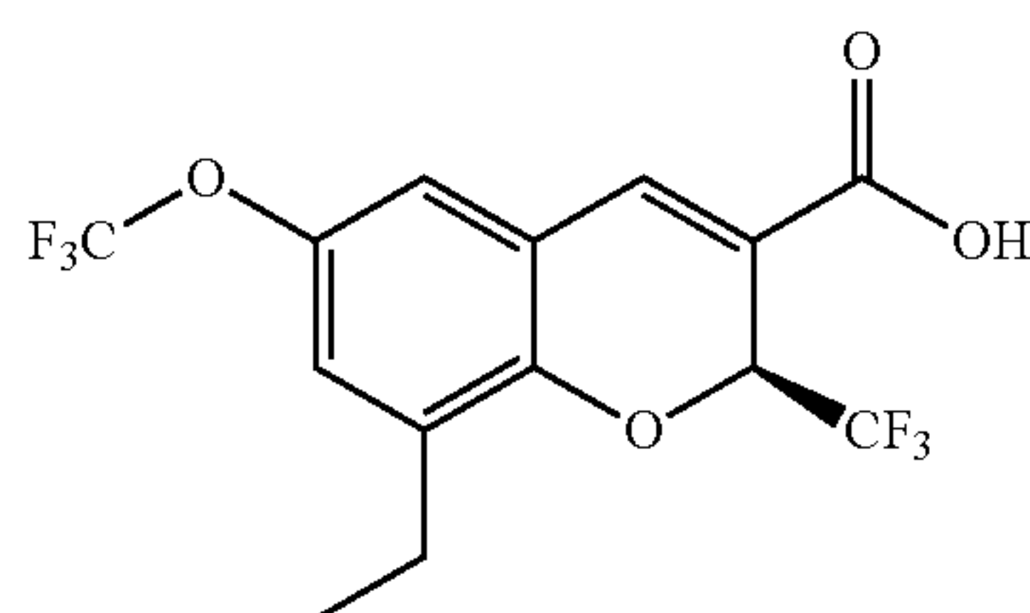
(2S)-8-ethyl-6-(trifluoromethoxy)-2-(trifluoromethyl)-2H-chromene-3-carboxylic acid
