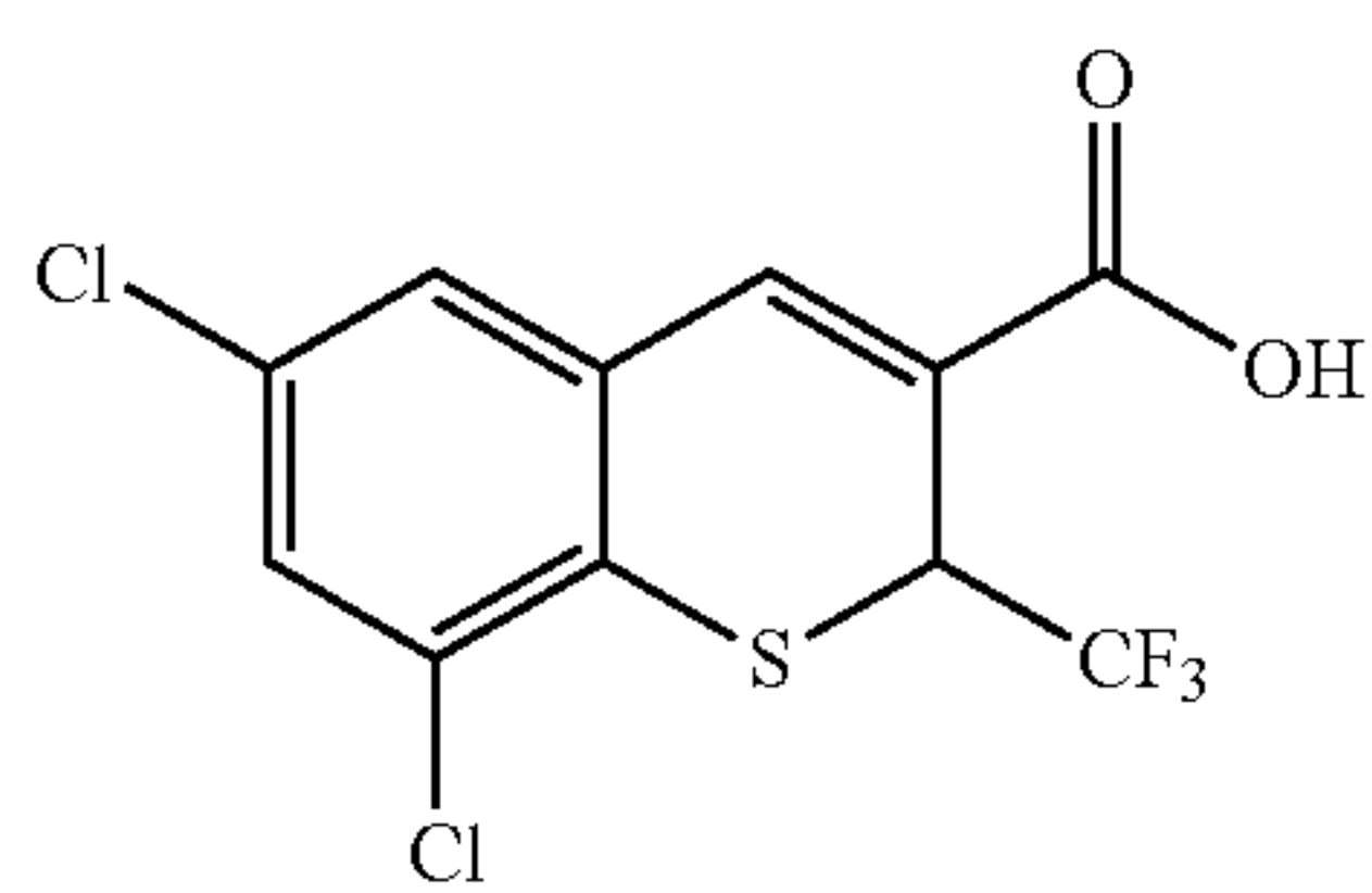
6,8-Dichloro-2-trifluoromethyl-2H-1-benzothiopyran-3-carboxylic acid
