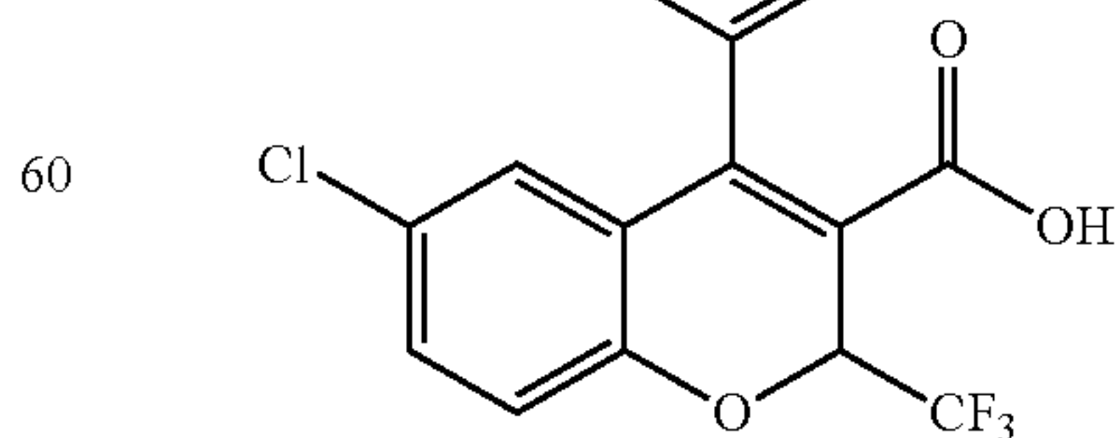
6-Chloro-2-(trifluoromethyl)-4-phenyl-2H-1-benzopyran-3-carboxylic acid
