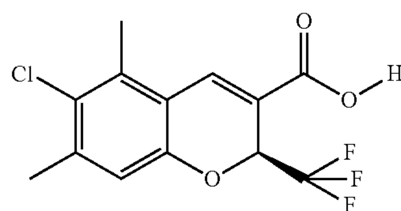
(2S)-6-chloro-5,7-dimethyl-2-(trifluoromethyl)-2H-chromene-3-carboxylic acid
