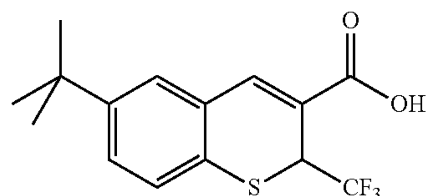
6-(1,1-Dimethylethyl)-2-(trifluoromethyl)-2H-1-benzothiopyran-3-carboxylic acid
