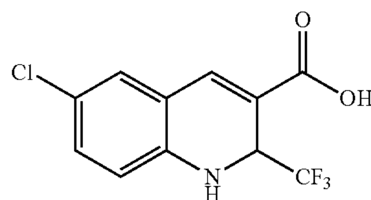
6-Chloro-2-(trifluoromethyl)-1,2-dihydro[1,8]naphthyridine-3-carboxylic acid
