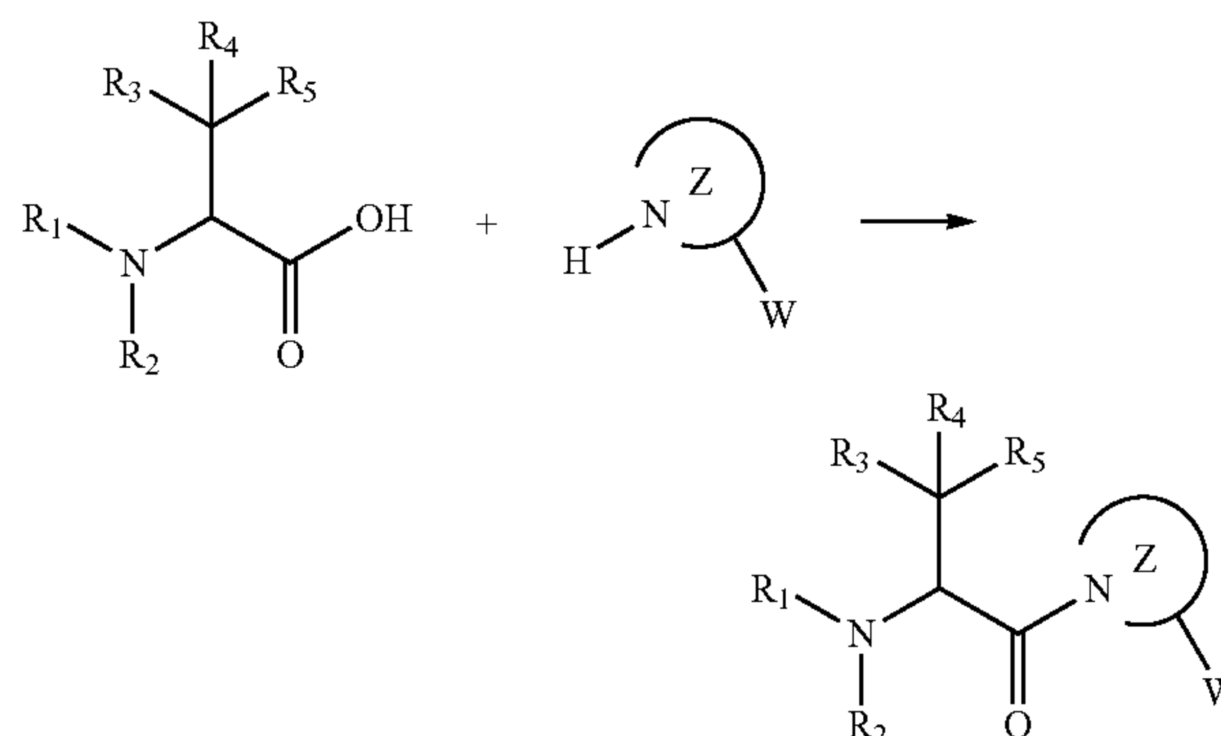
Scheme 1. General synthetic method
