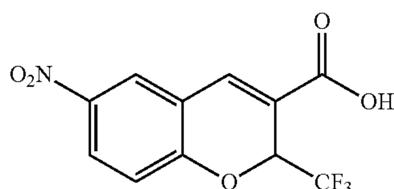
6-Nitro-2-trifluoromethyl-2H-1-benzopyran-3-carboxylic acid
