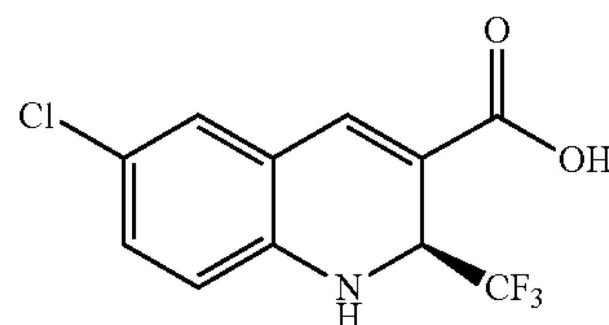
(SS)-6-Chloro-1,2-dihydro-2-(trifluoromethyl)-3-quinolinecarboxylic acid
