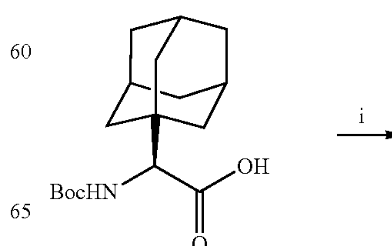
Scheme 2. Synthetic method for ARI-5544 a
