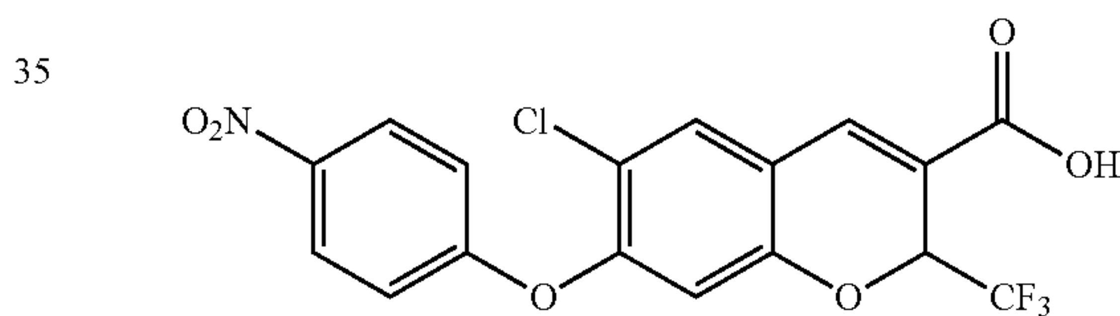
6-Chloro-7-(4-nitrophenoxy)-2-(trifluoromethyl)-2H-1-benzopyran-3-carboxylic acid
