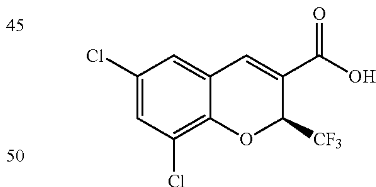
((S)-6,8-Dichloro-2-(trifluoromethyl)-2H-1-benzopyran-3-carboxylic acid
