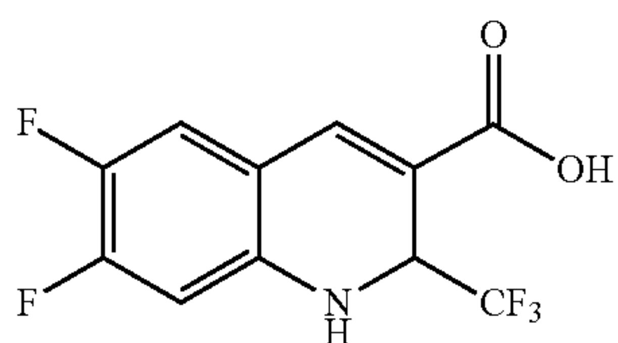
6,7-Difluoro-1,2-dihydro-2-(trifluoromethyl)-3-quinolinecarboxylic acid
