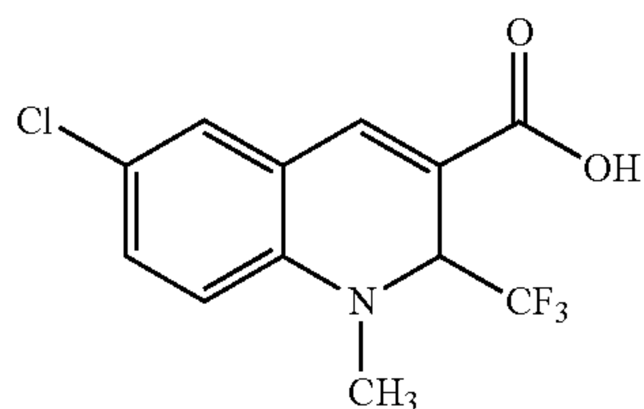
6-Chloro-1,2-dihydro-1-methyl-2-(trifluoromethyl)-3-quinolinecarboxylic acid
