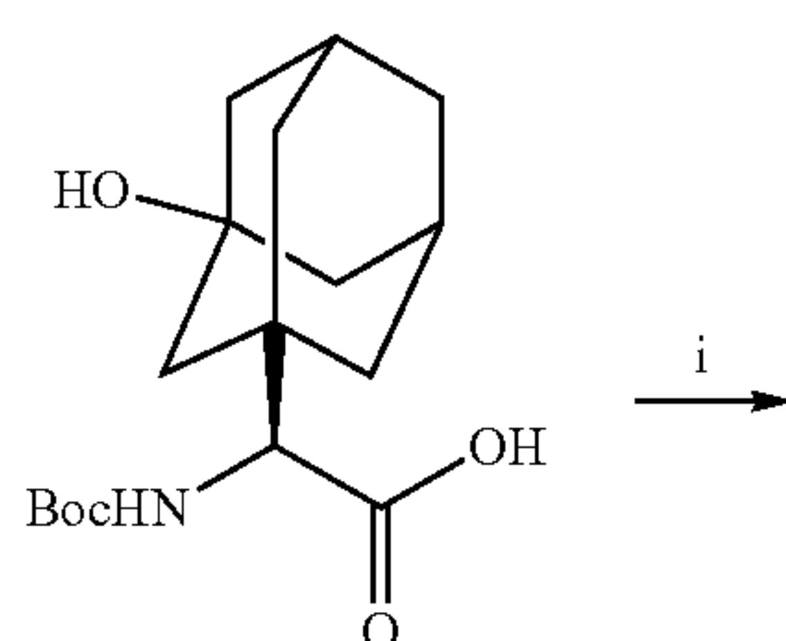
Scheme 3. Synthetic method for 3102C a
