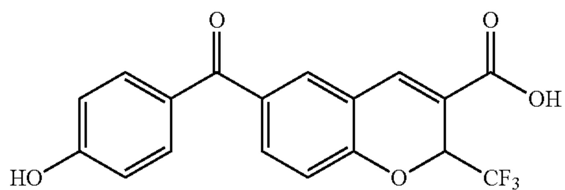
6-(4-Hydroxybenzoyl)-2-(trifluoromethyl)-2H-1-benzopyran-3-carboxylic acid
