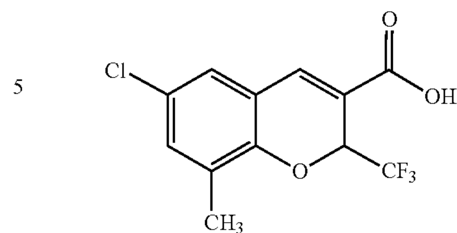
6-Chloro-8-methyl-2-trifluoromethyl-2H-1-benzopyran-3-carboxylic acid
