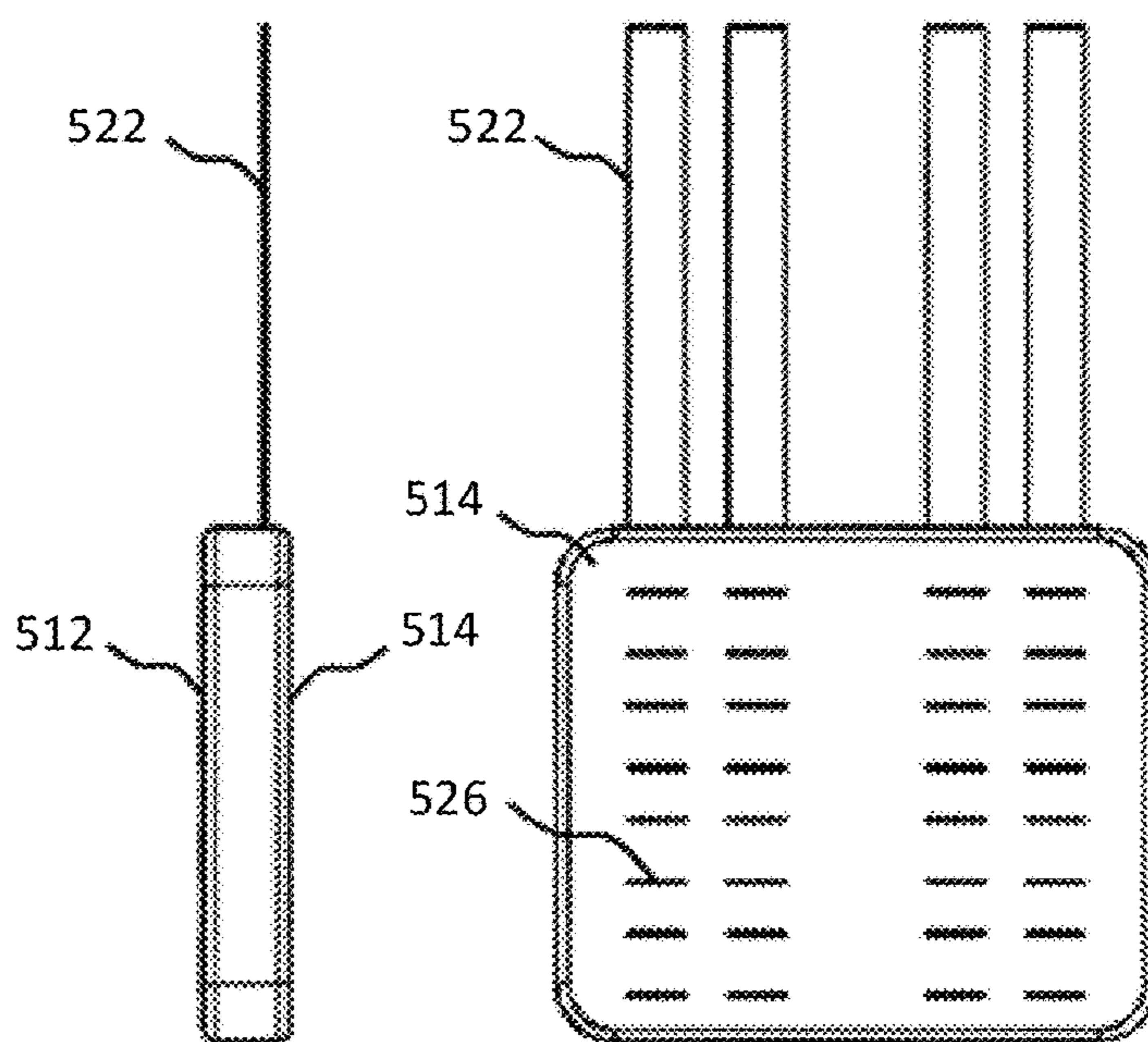
(SIDE)
