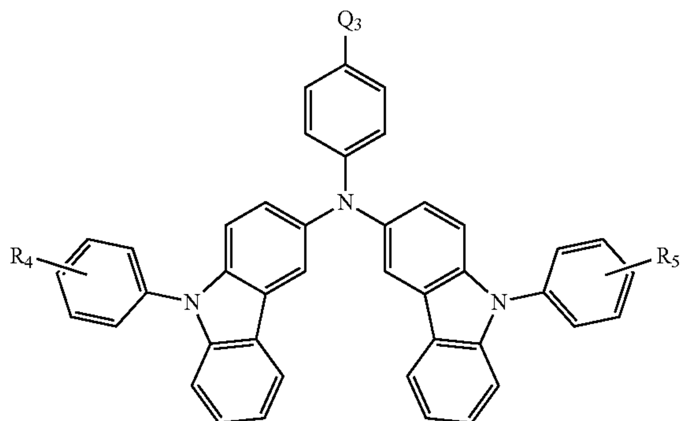
Formula 2a
