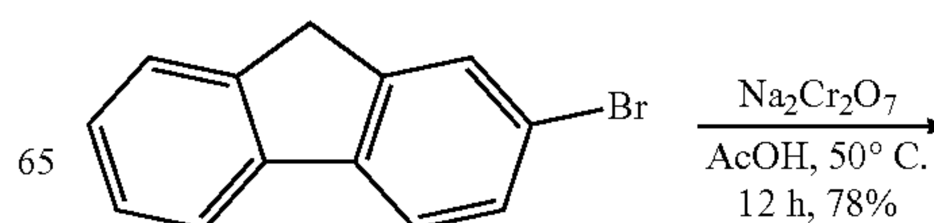
Reaction Scheme 9
