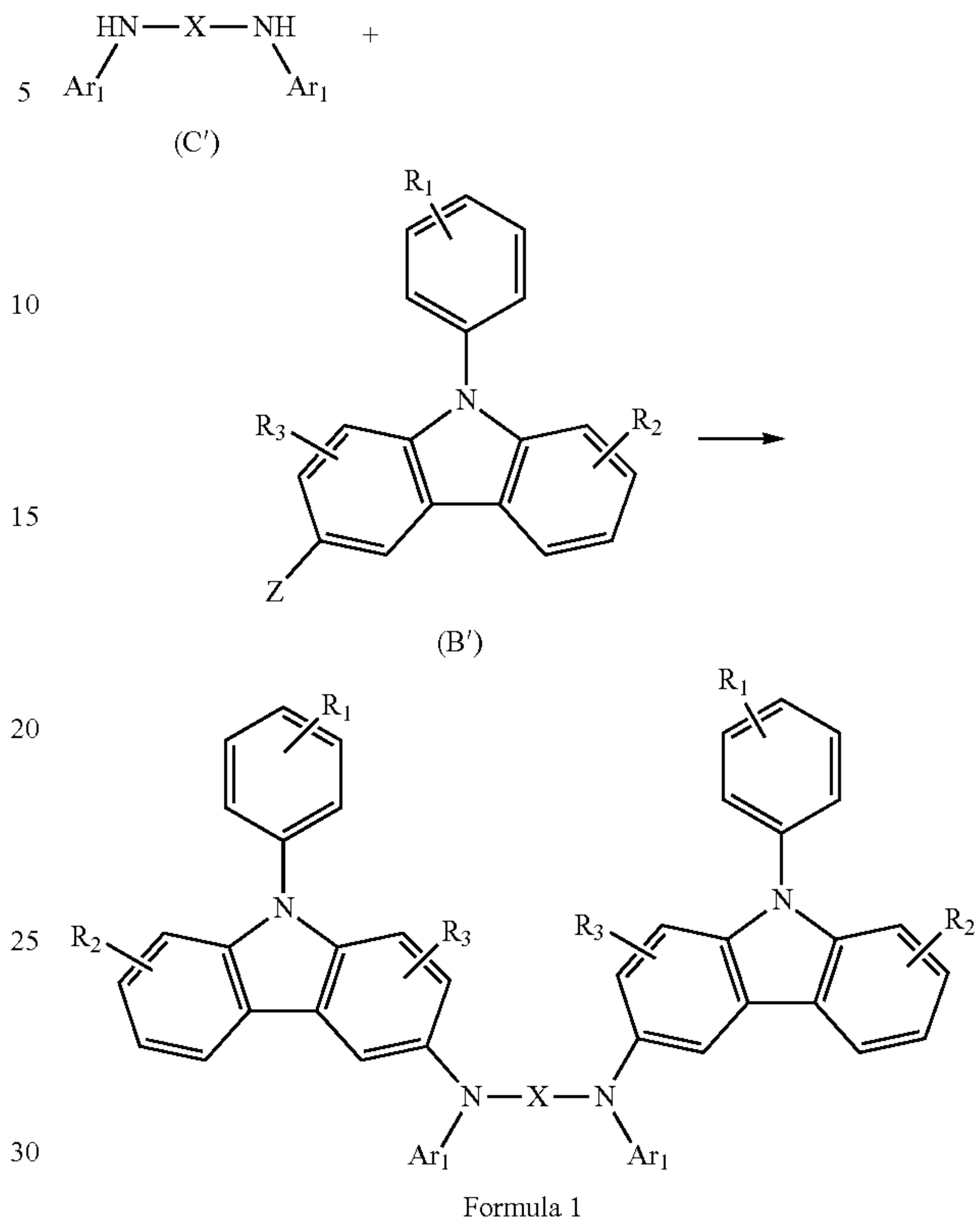
Reaction Scheme 1
