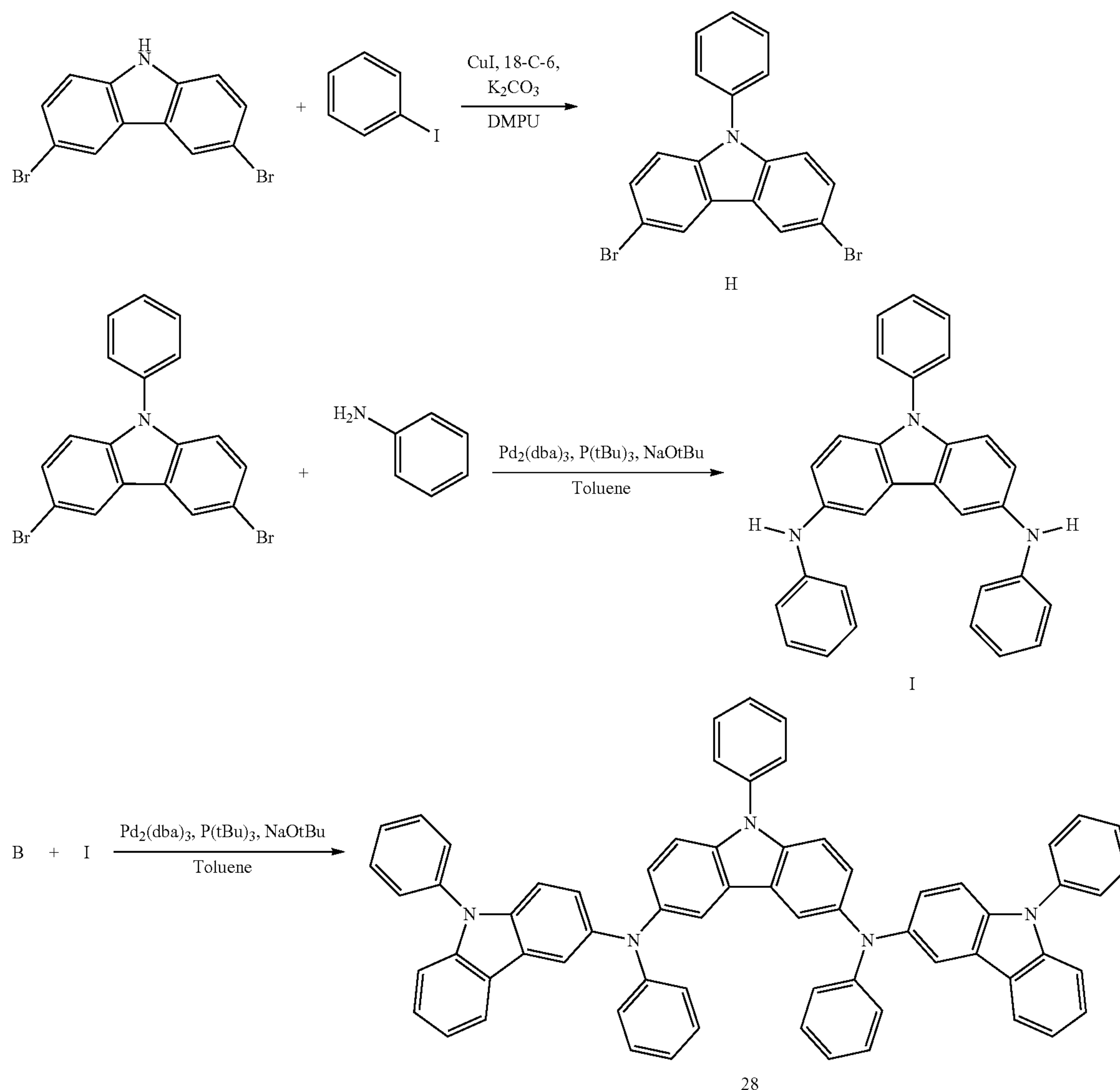
Reaction Scheme 7
