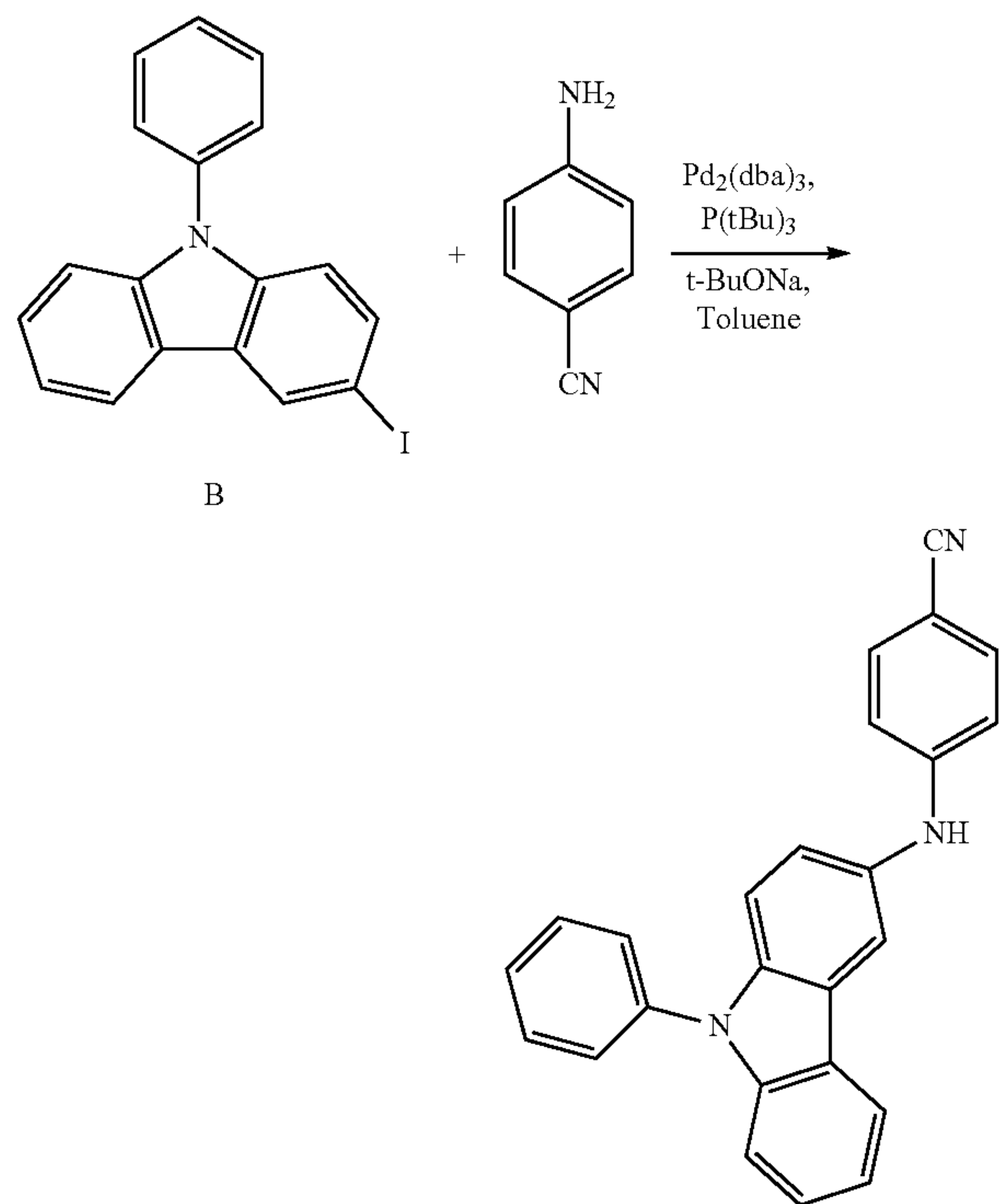
Reaction Scheme 8
