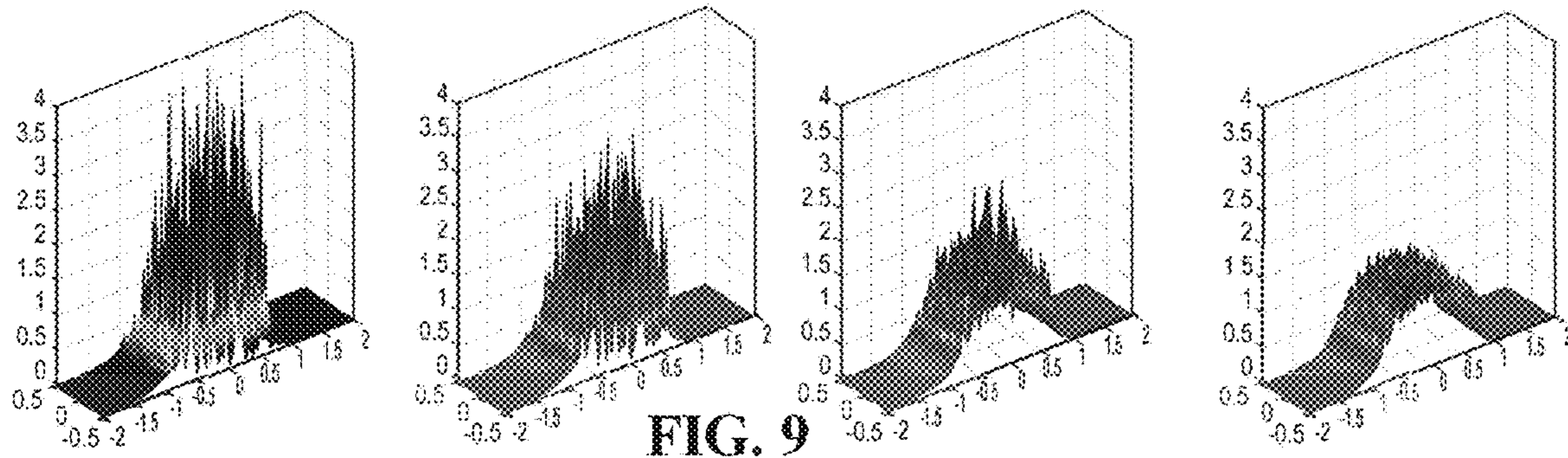
Mixed-EHL pressure profiles for progressively smoother surface roughness (scaled RMS)
