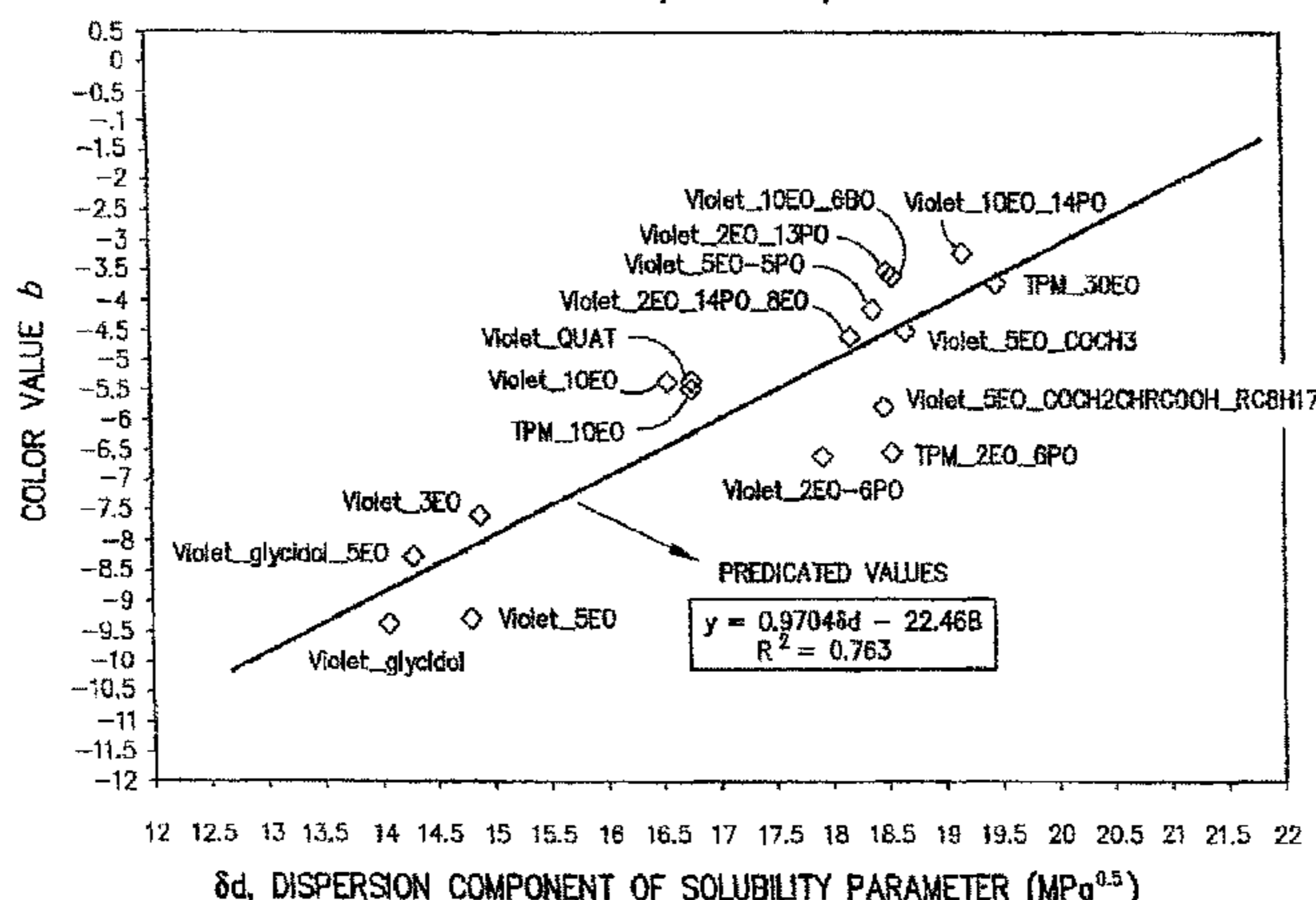
CALCULATED VERSUS MEASURED b COLOR VALUES FOR POWDERED CELLULOSE WASHED IN DETERGENT/COLORANT/WATER MIXTURE
