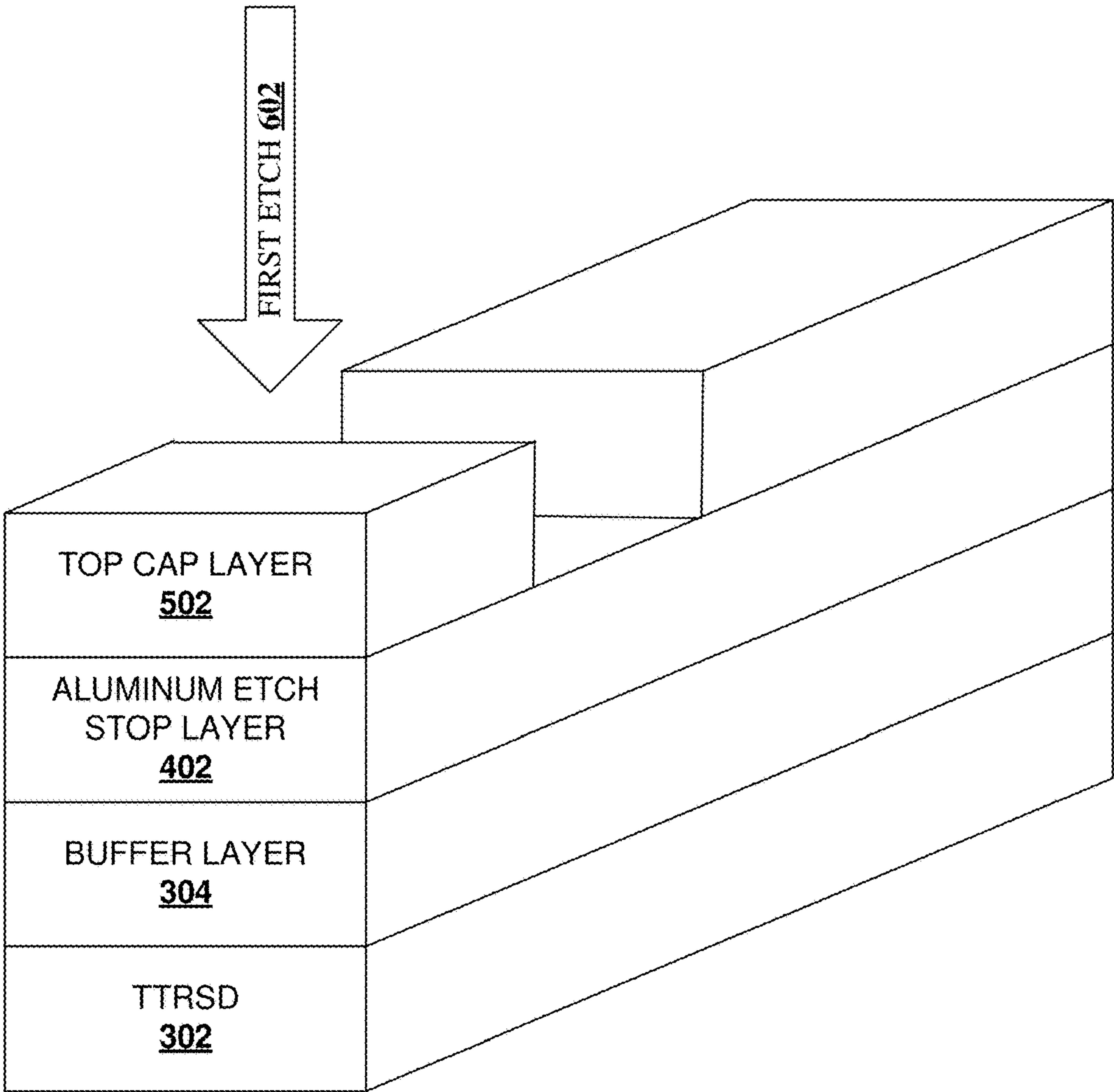
EXAMPLE 3D VIEW SHOWING FIRST ETCHING PROCEDURE
