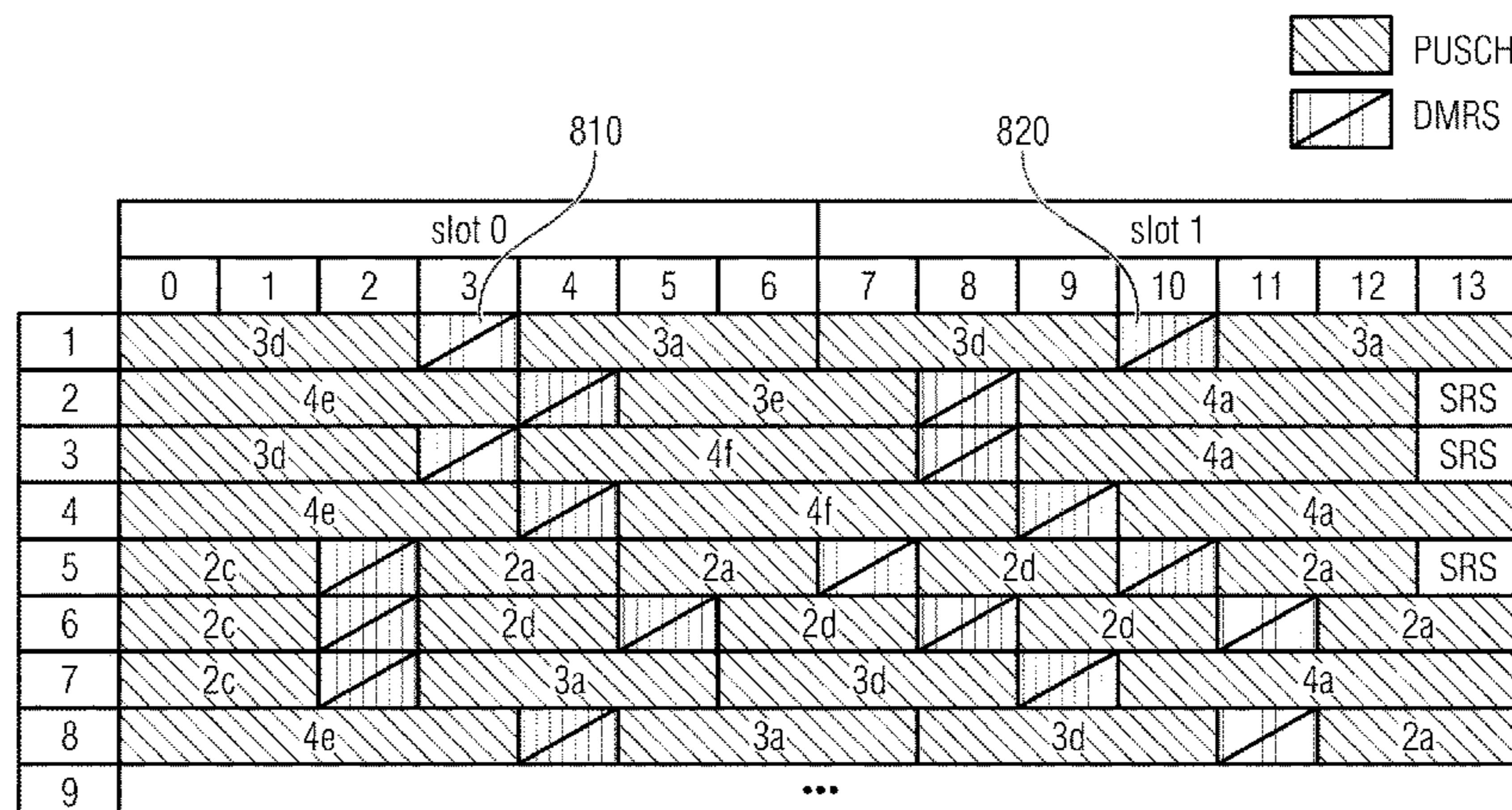
PUSCH sTTIs and corresponding DMRS slots in (Example... should contain every possible variation)
