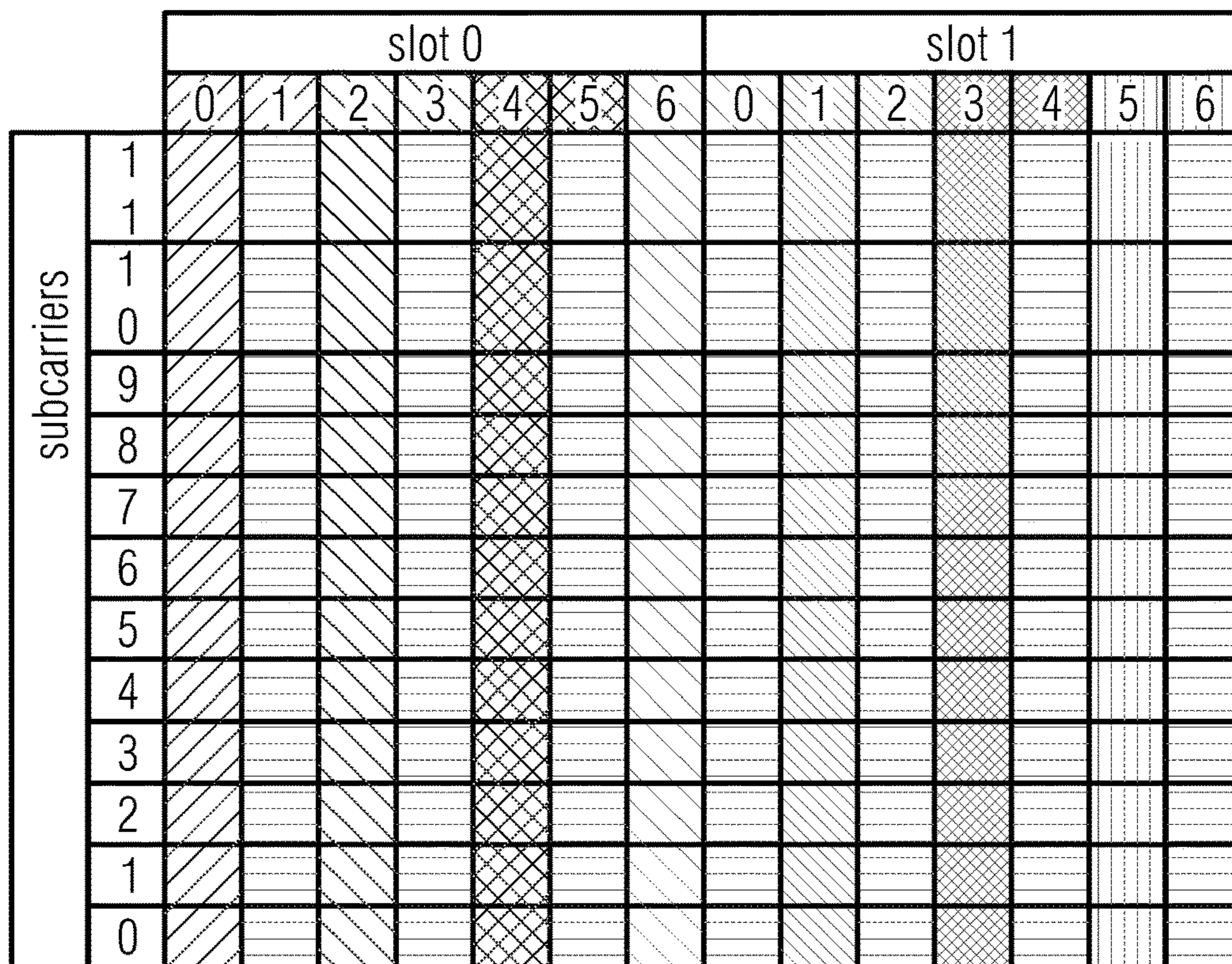
Example of an uplink subframe with sTTI length 3/4 and 2 OFDM symbols
