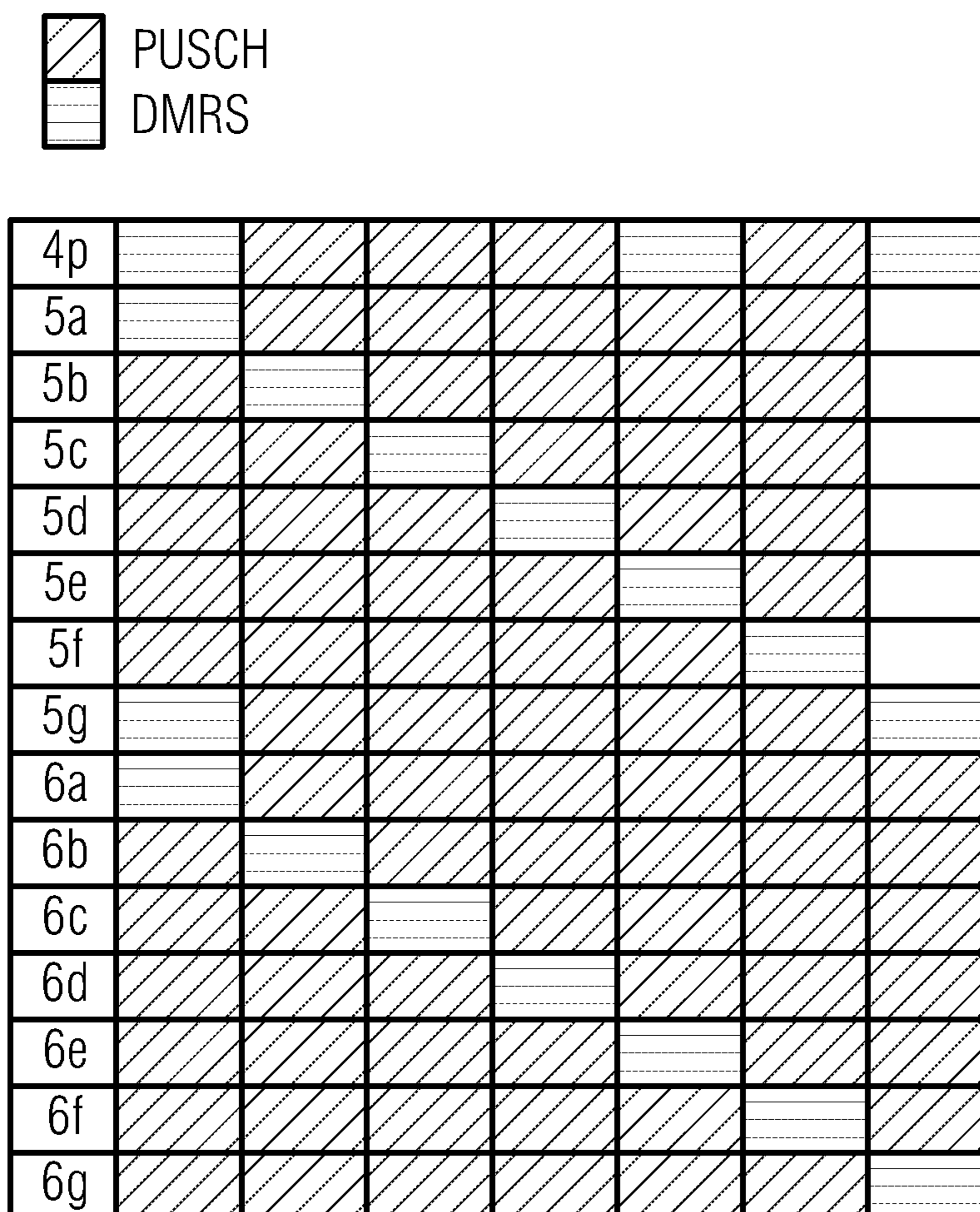
sTTI possible DMRS positions
