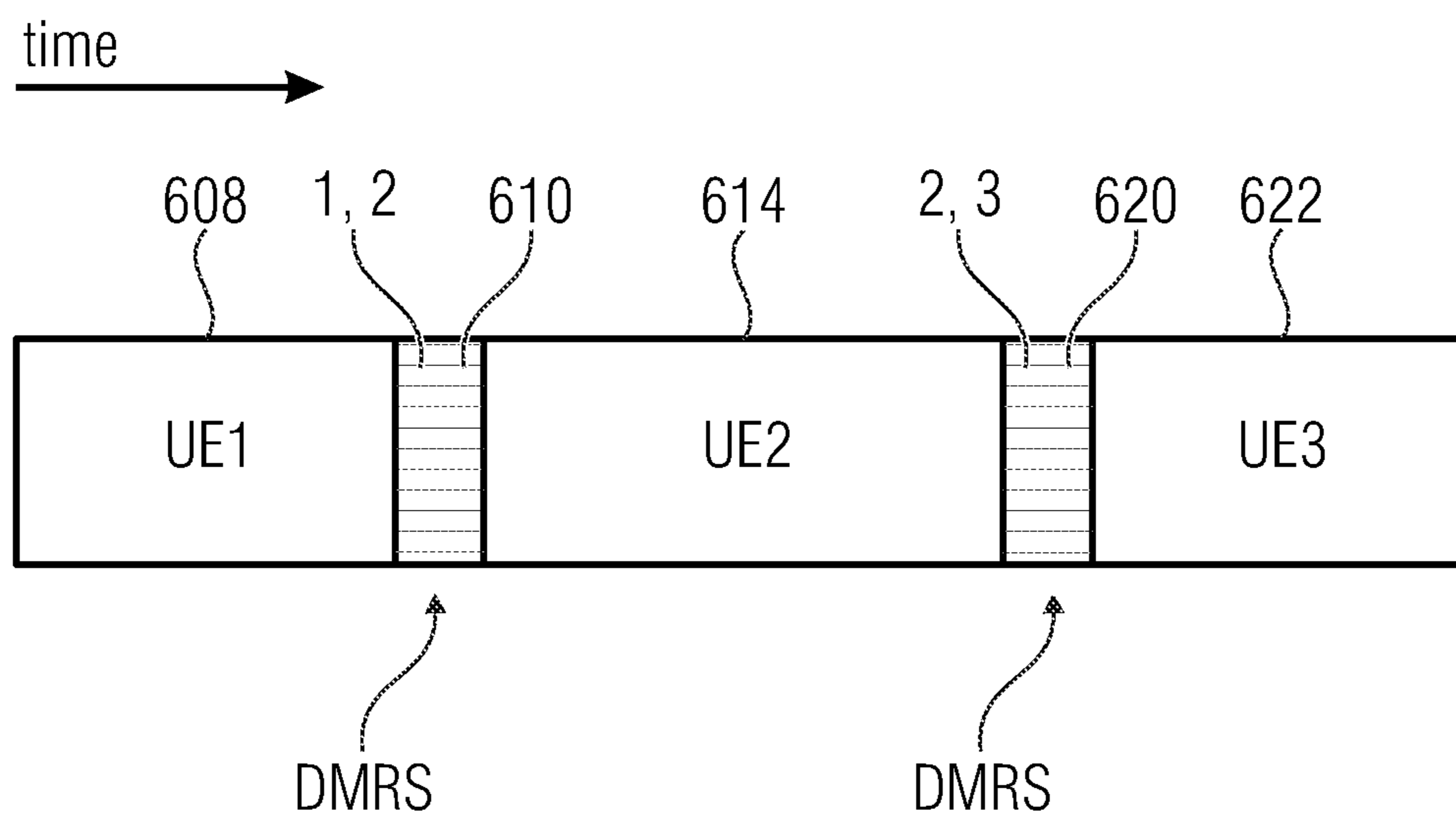
Multiplexing of UEs with different transmission lengths
