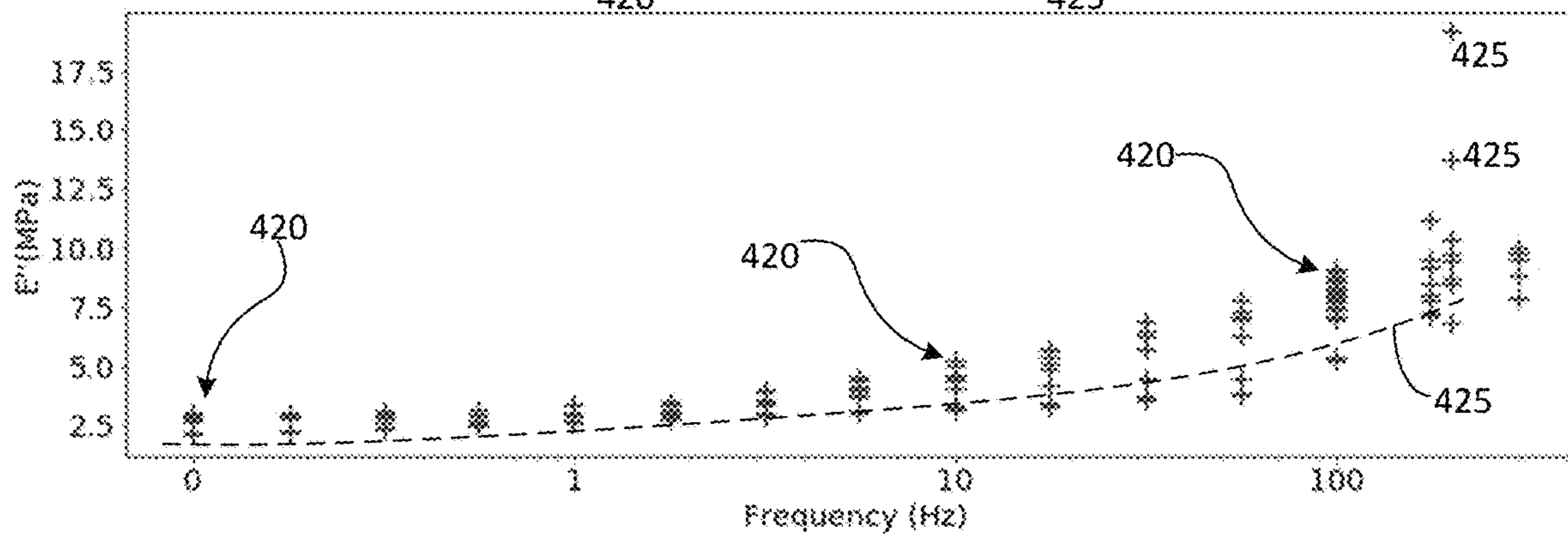
FIG. 4B 420 425 Loss Modulus (red: nDMA w/ Poisson 0.5; green: Bulk DMA)
