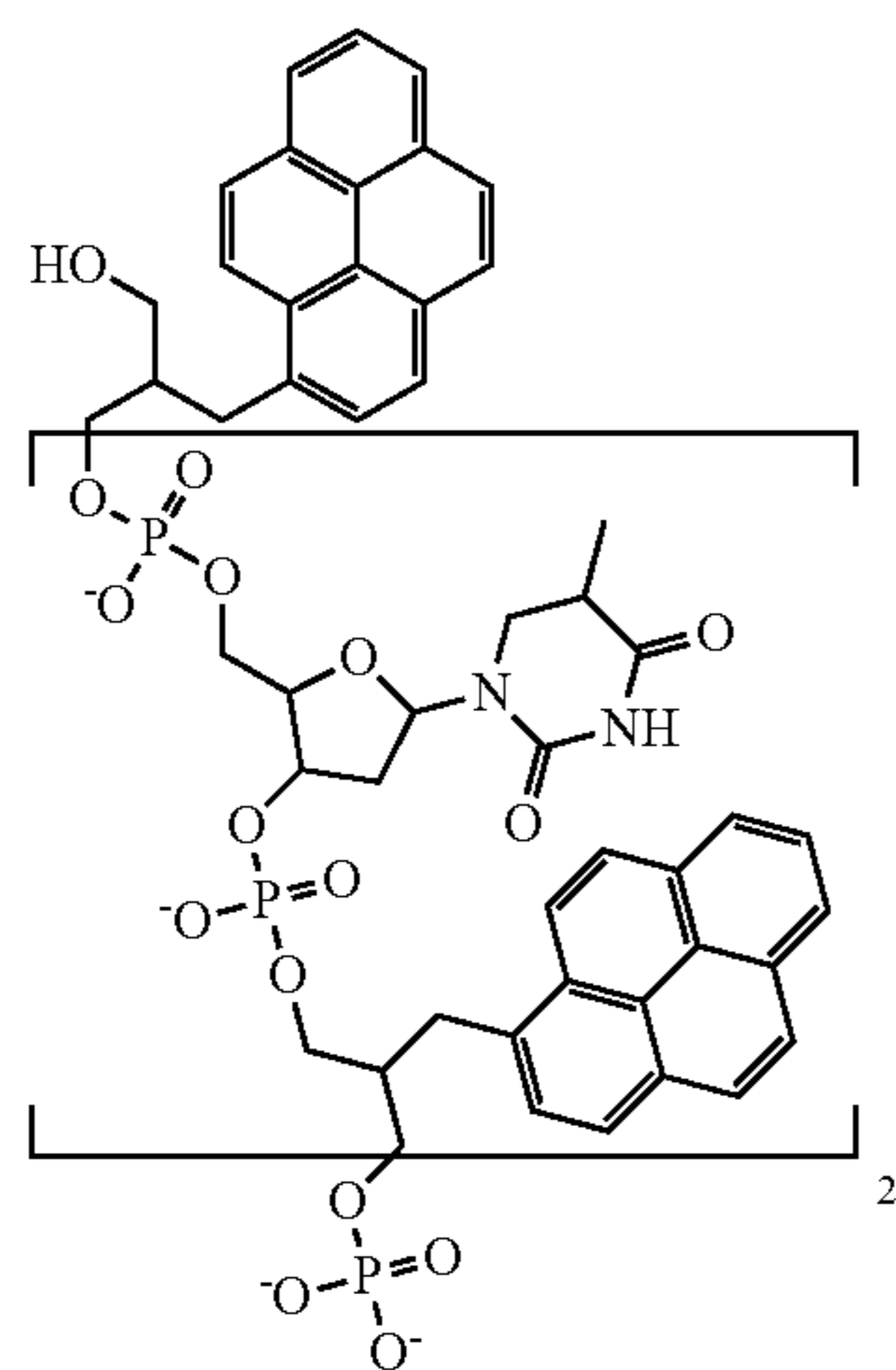
5'-YT h YT h Y-3'
