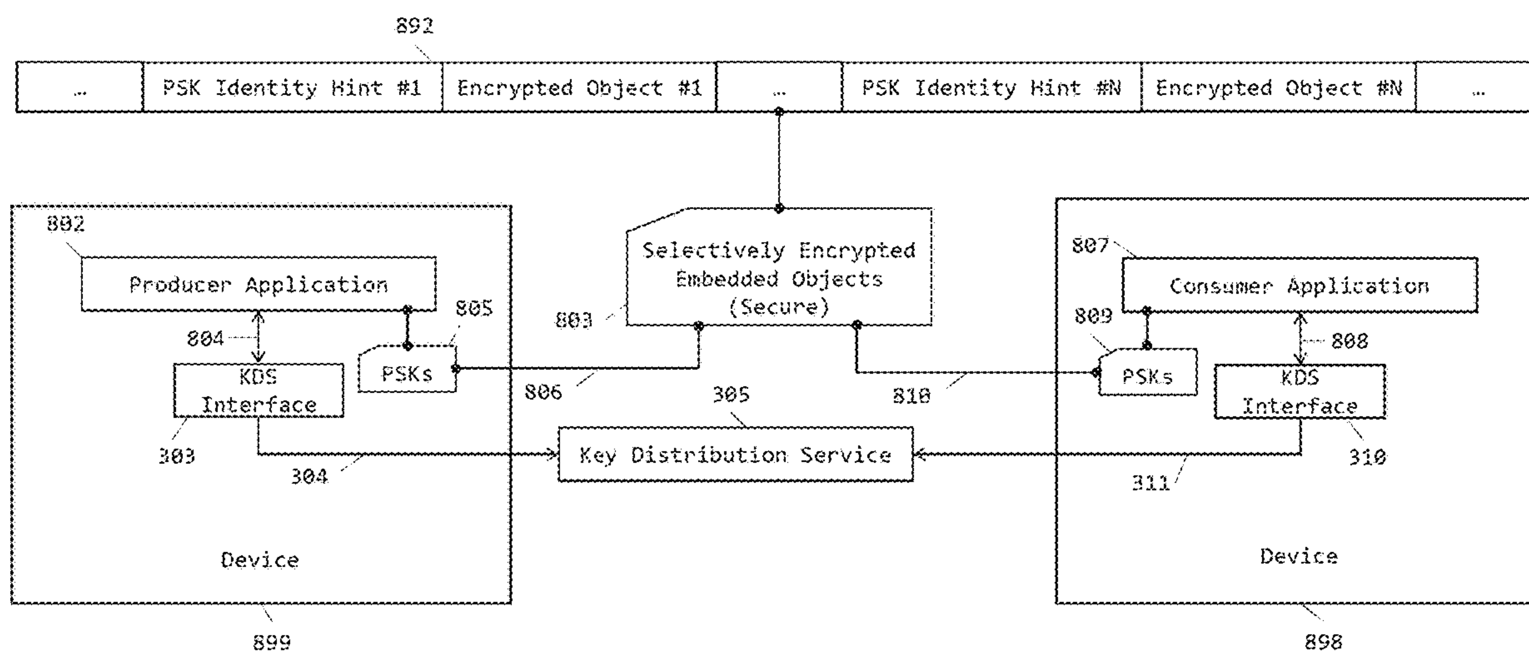
FIG. 8B PRE-SHARED KEY BASED SELECTIVE ENCRYPTION OF OBJECTS EMBEDDED WITHIN DOCUMENTS
