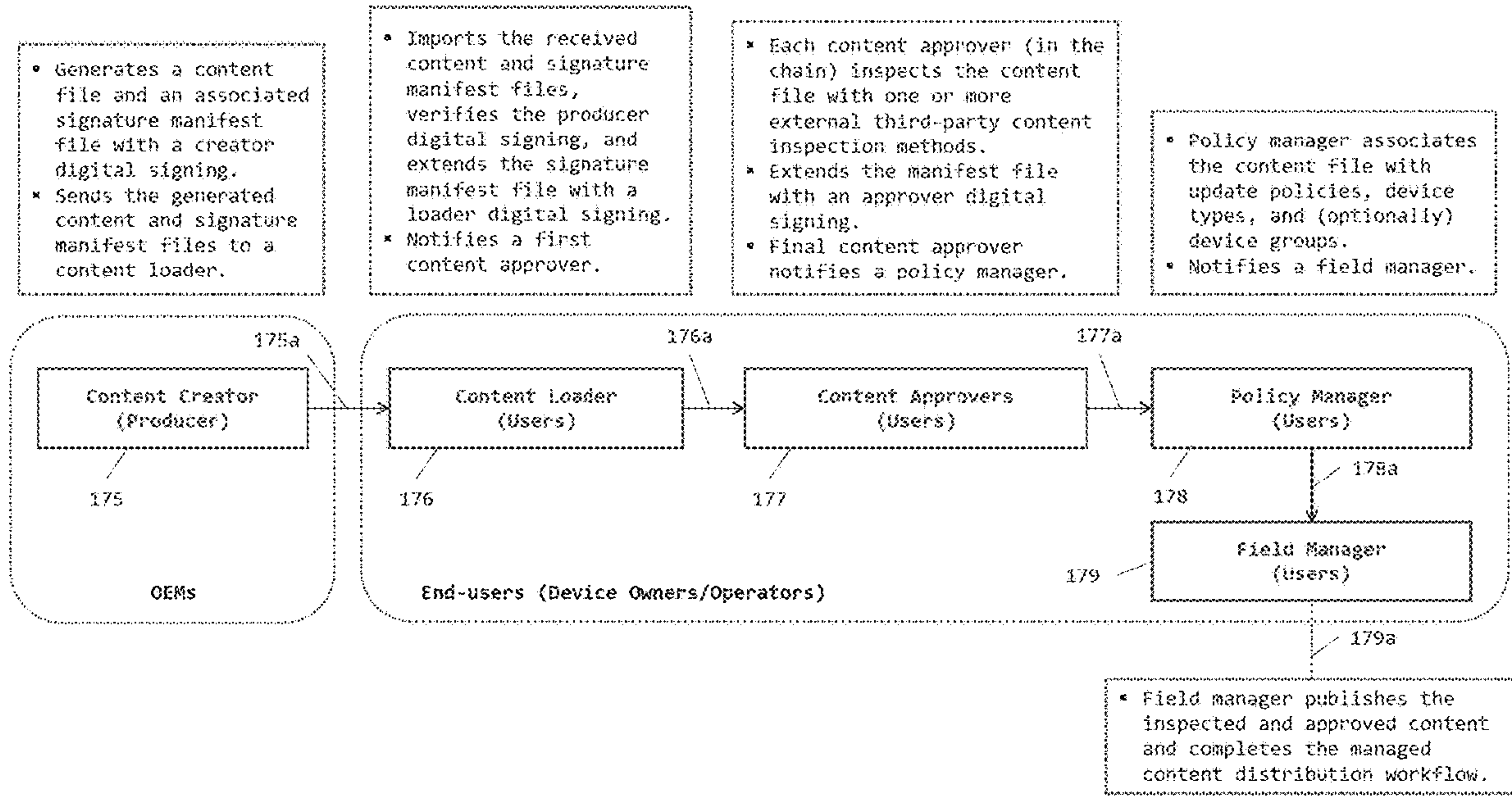
FIG. 1E MULTI-PARTY MULTI-PERSON MULTI-PART CONTENT INSPECTION AND APPROVAL WORKFLOW
