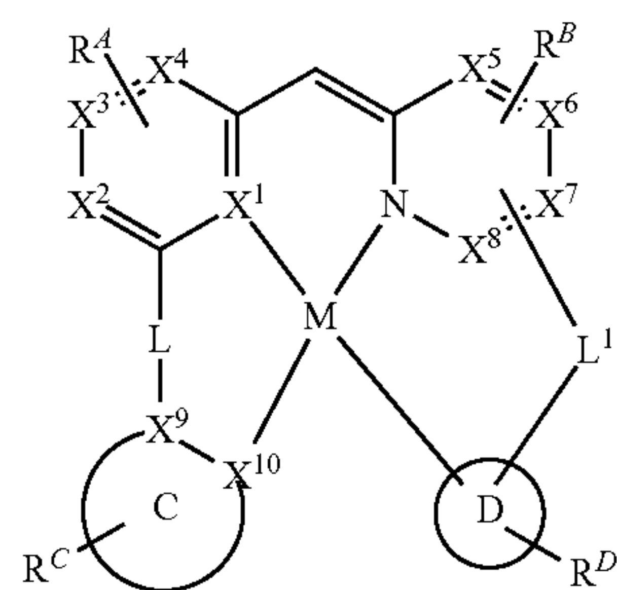
8a (M = Pt) 8b (M = Pd)
