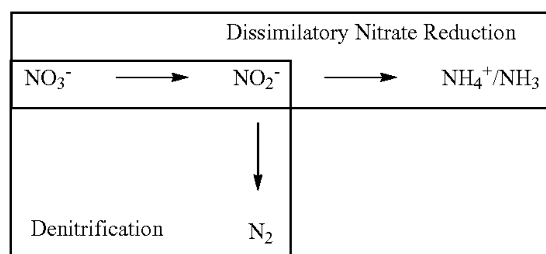
Scheme 1: Denitrification and DNRA pathways
