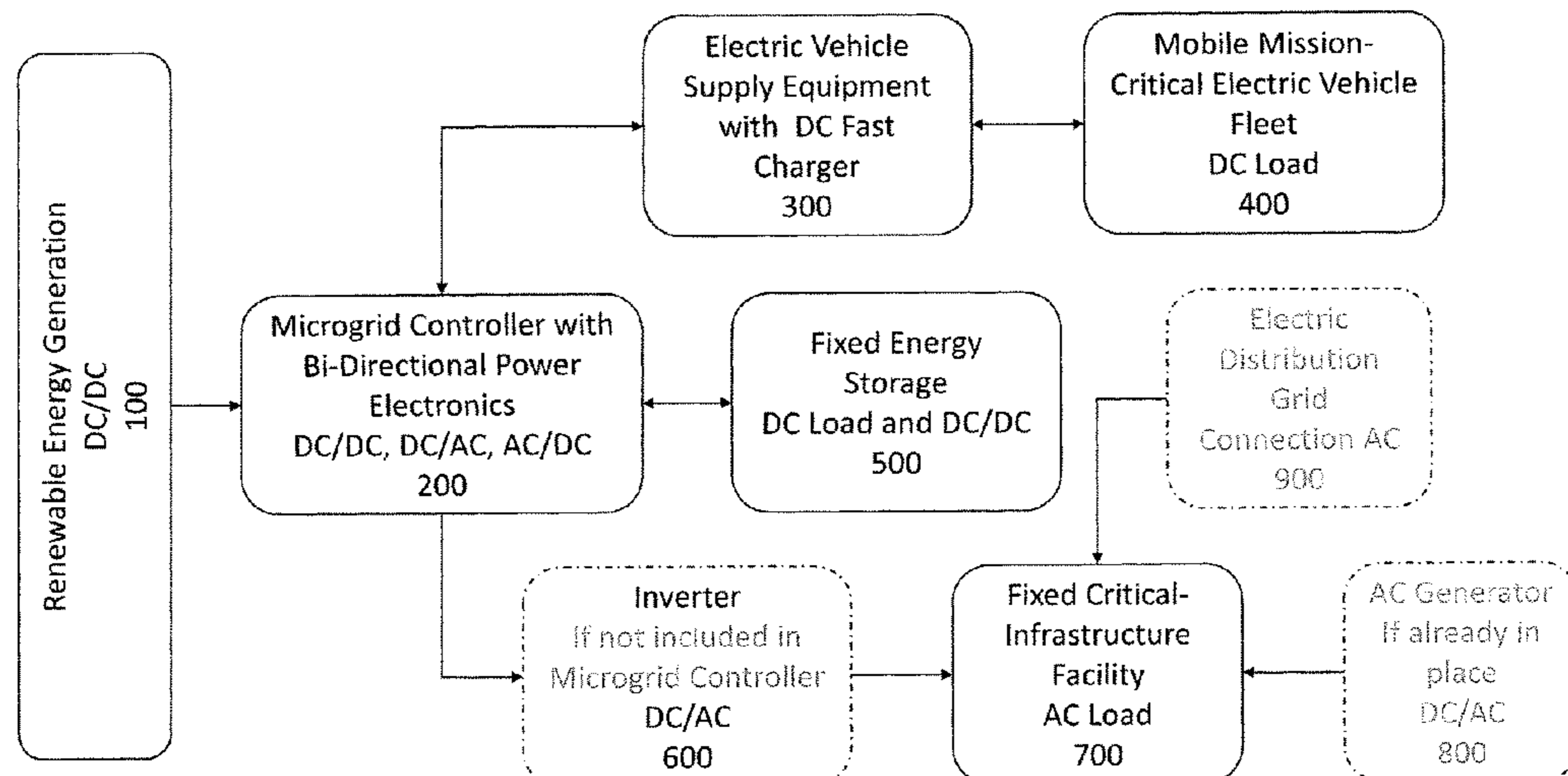
Mission-Critical Microgrid 1000
