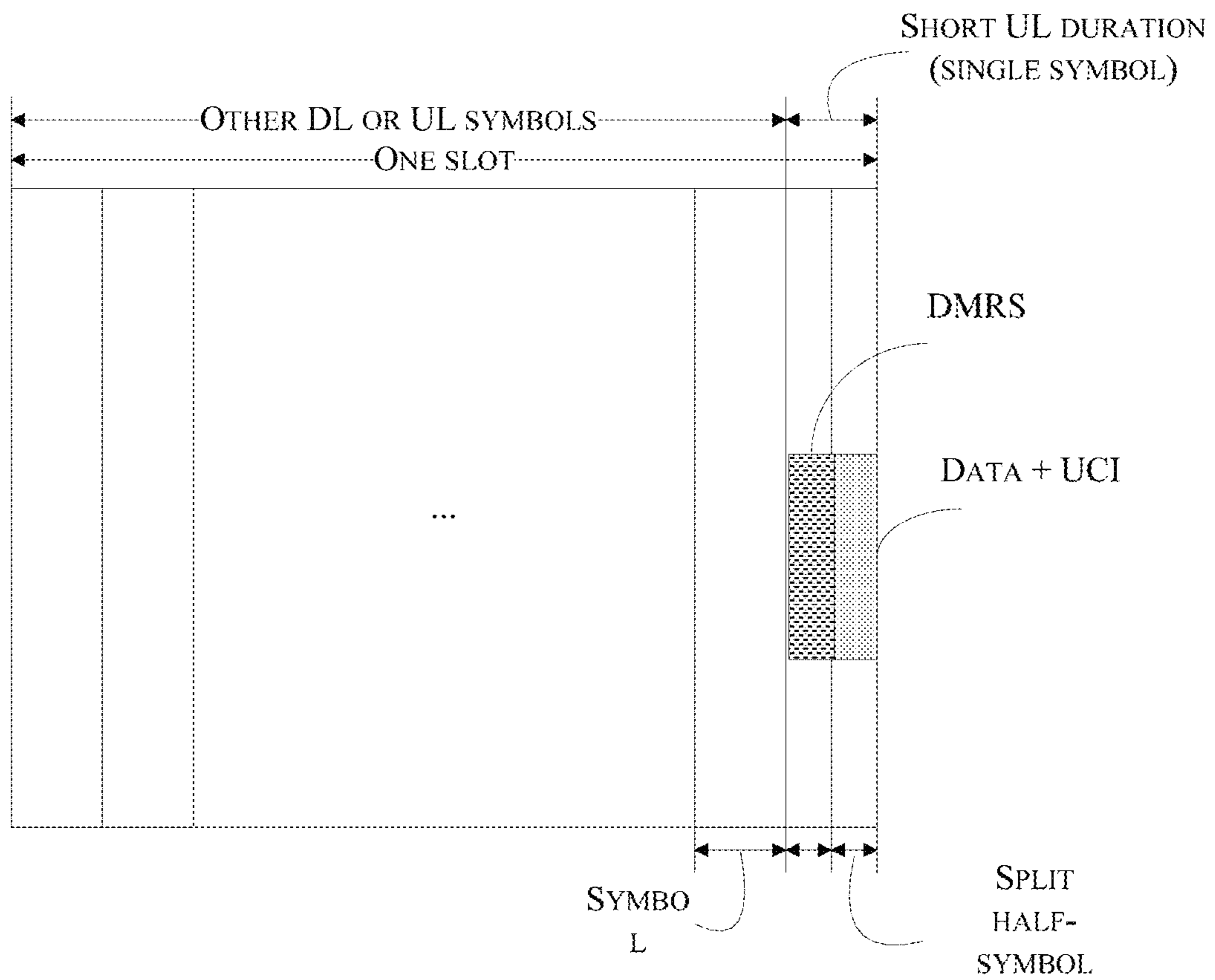
Figure 1C (Prior Art)
