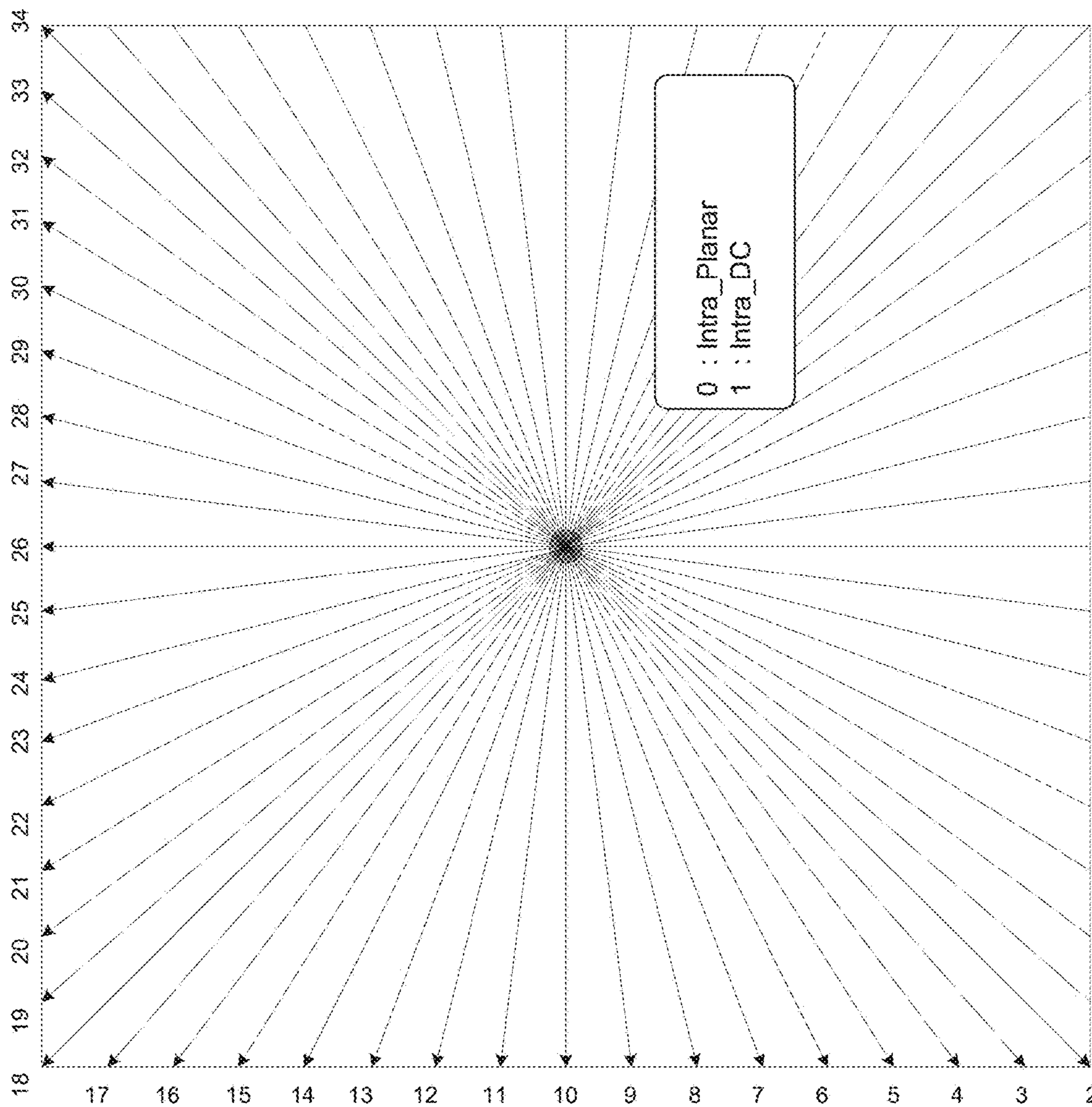
The 33 intra prediction directions
