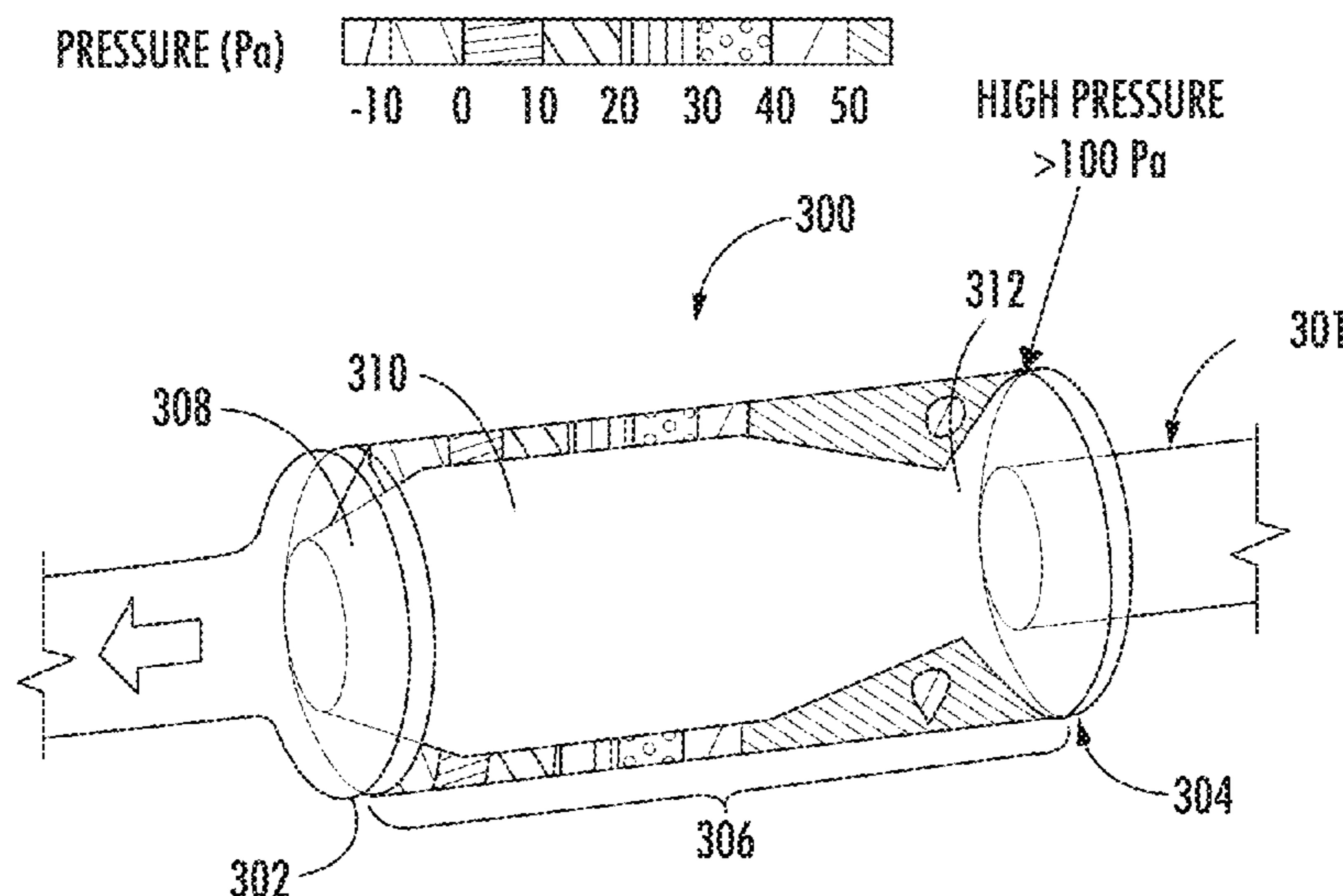
PRESSURE DISTRIBUTION
