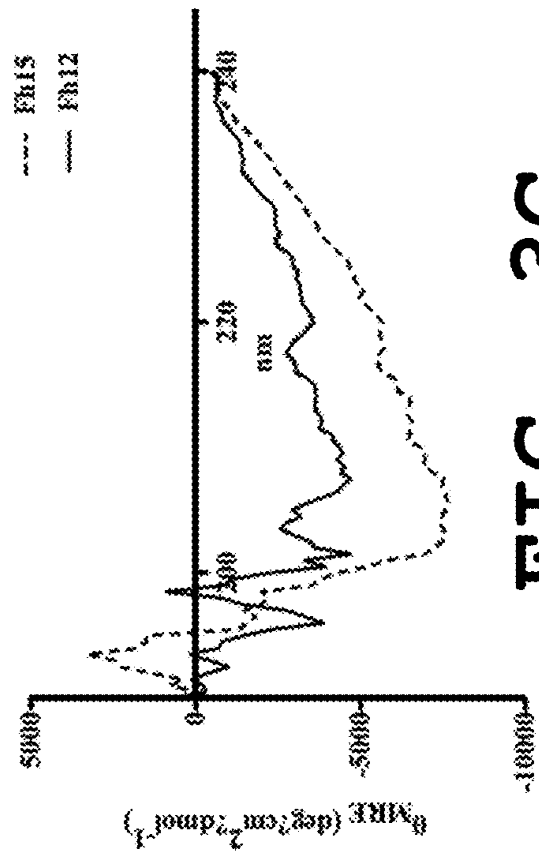
CD spectra 95°C
