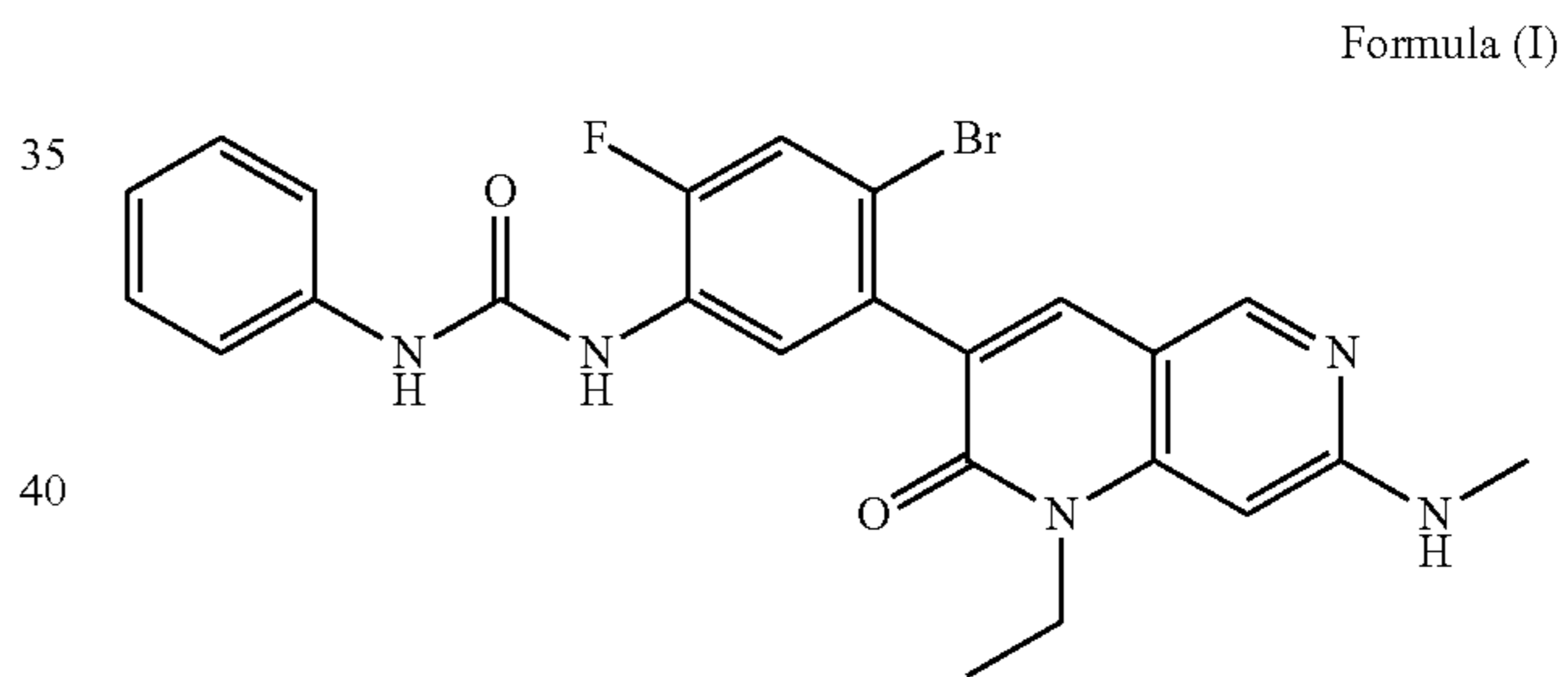
Formula (I)
