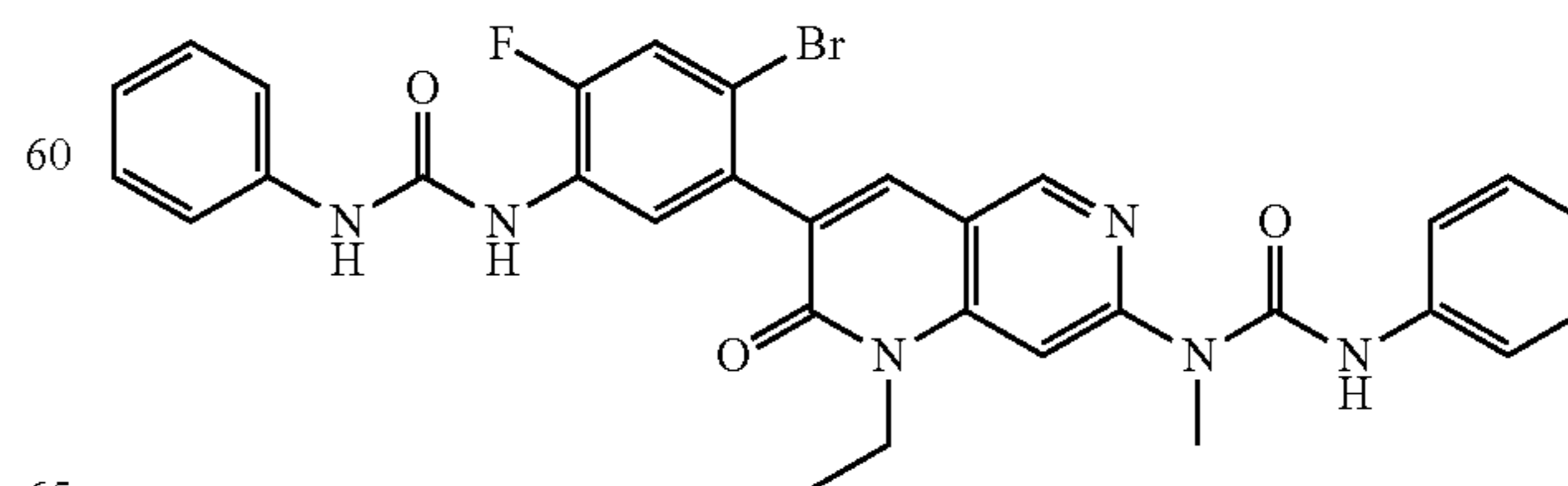
Formula (III)
