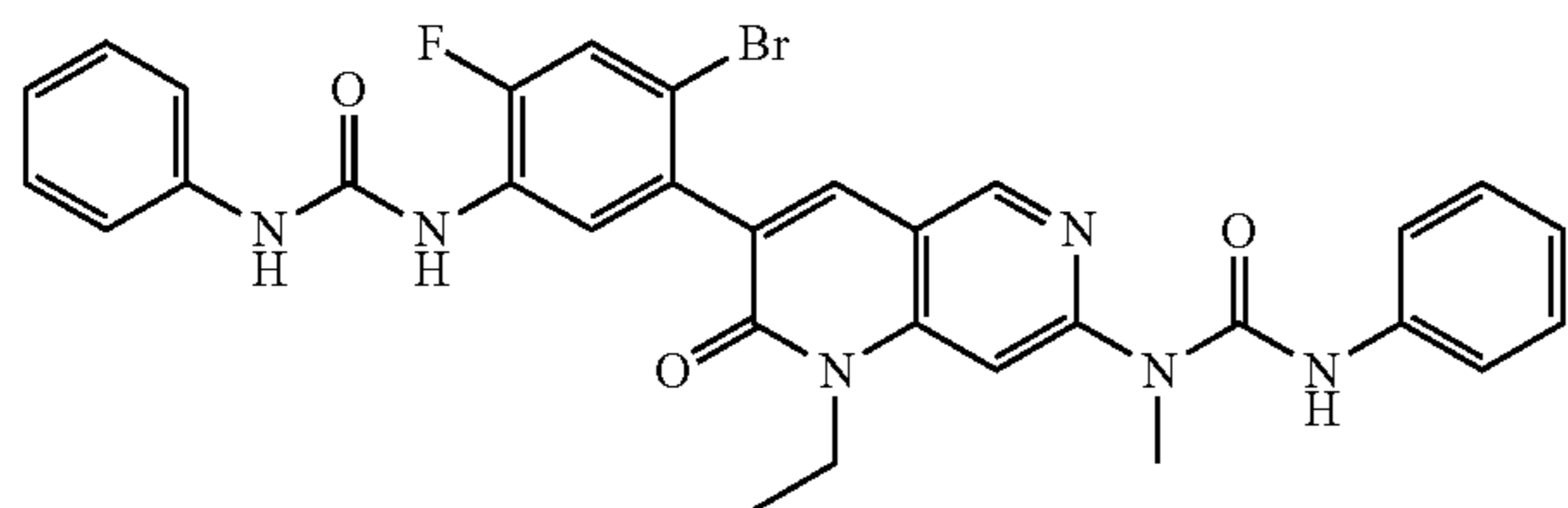
Formula (III)
