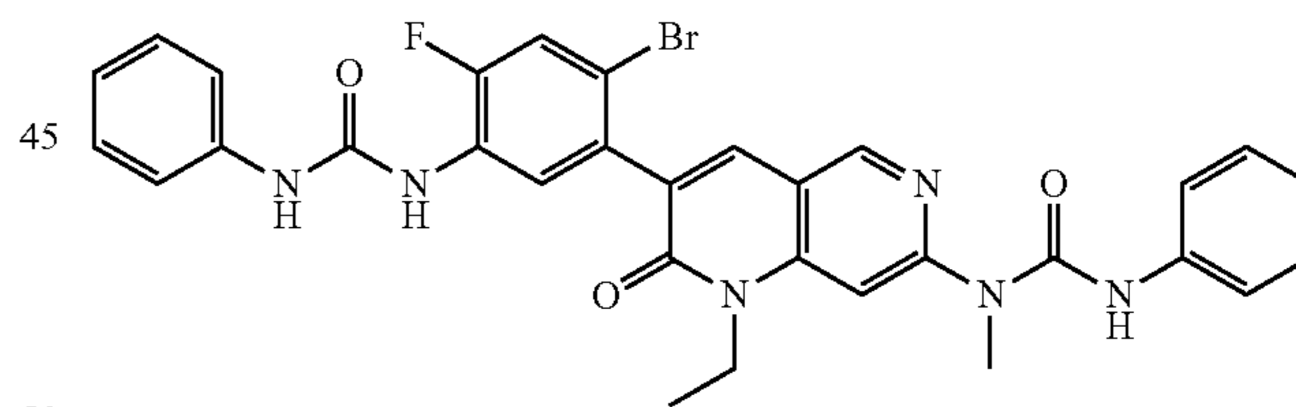
Formula (III)
