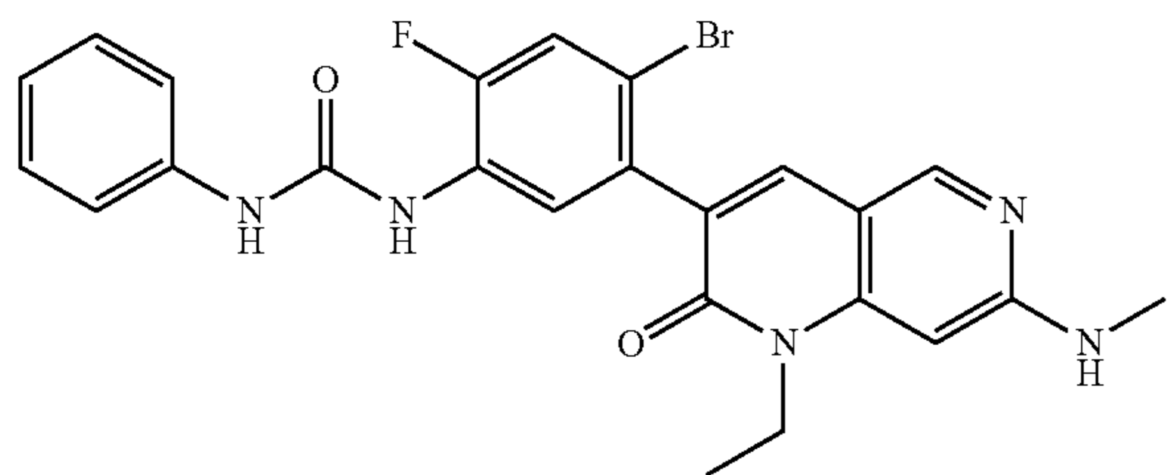
Formula (I)
