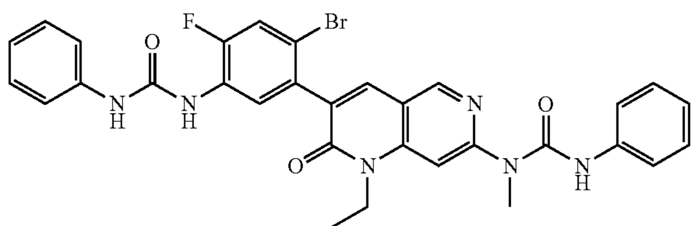
Formula (III)
