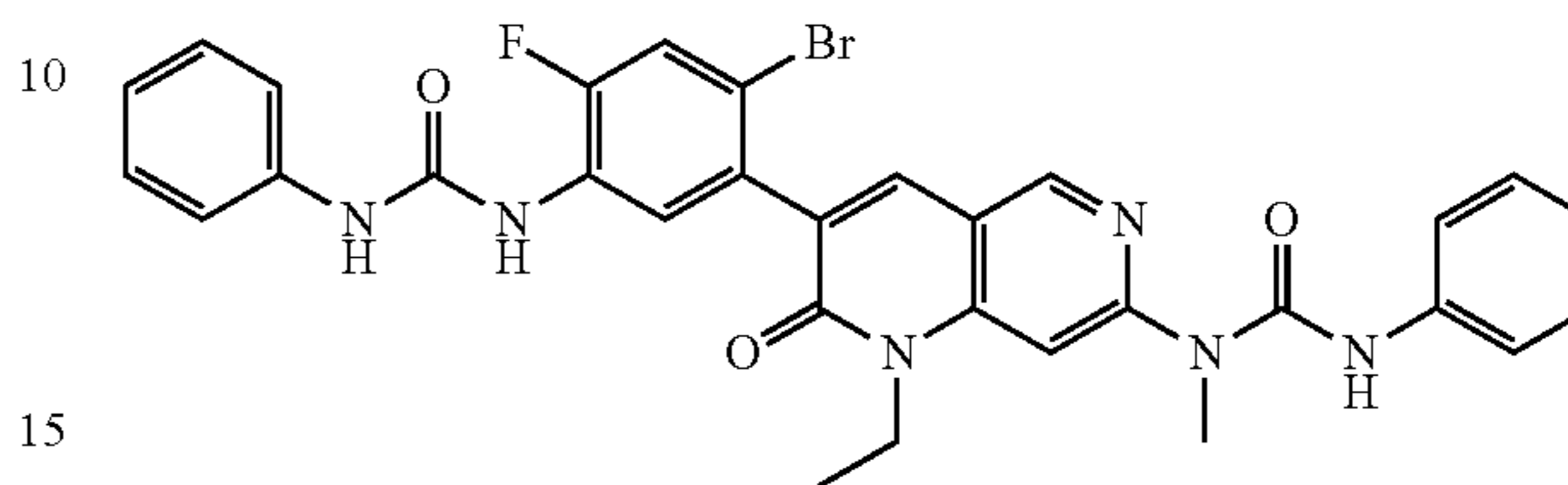
Formula (III)
