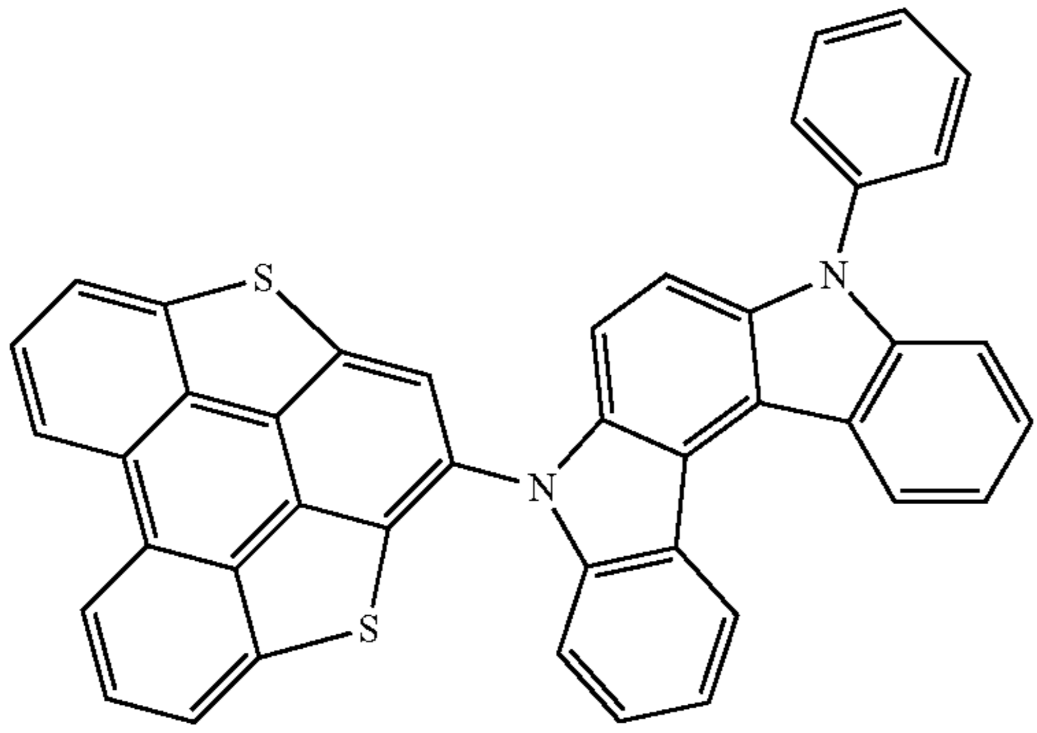
Compound 135
