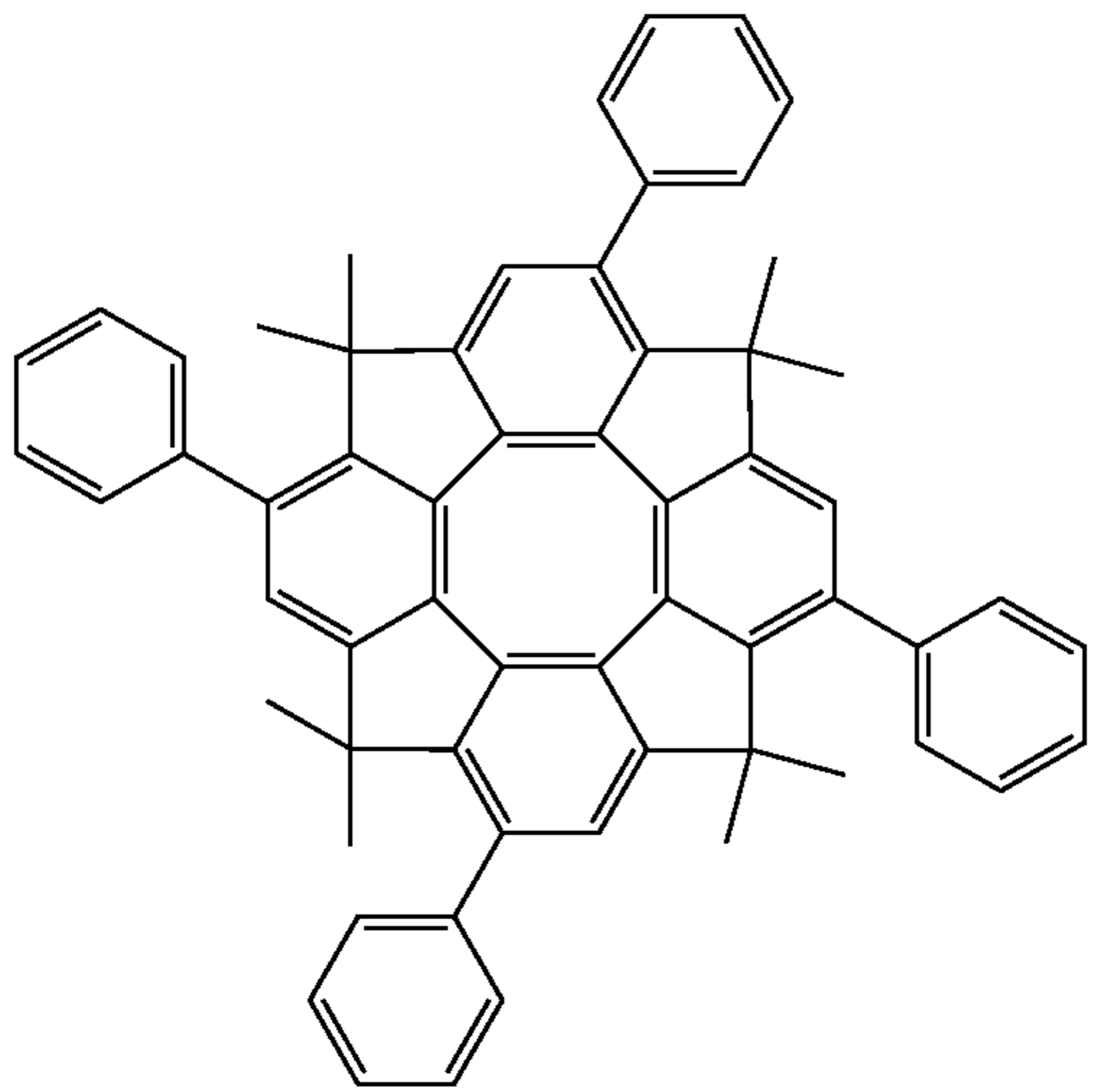
Compound 119
