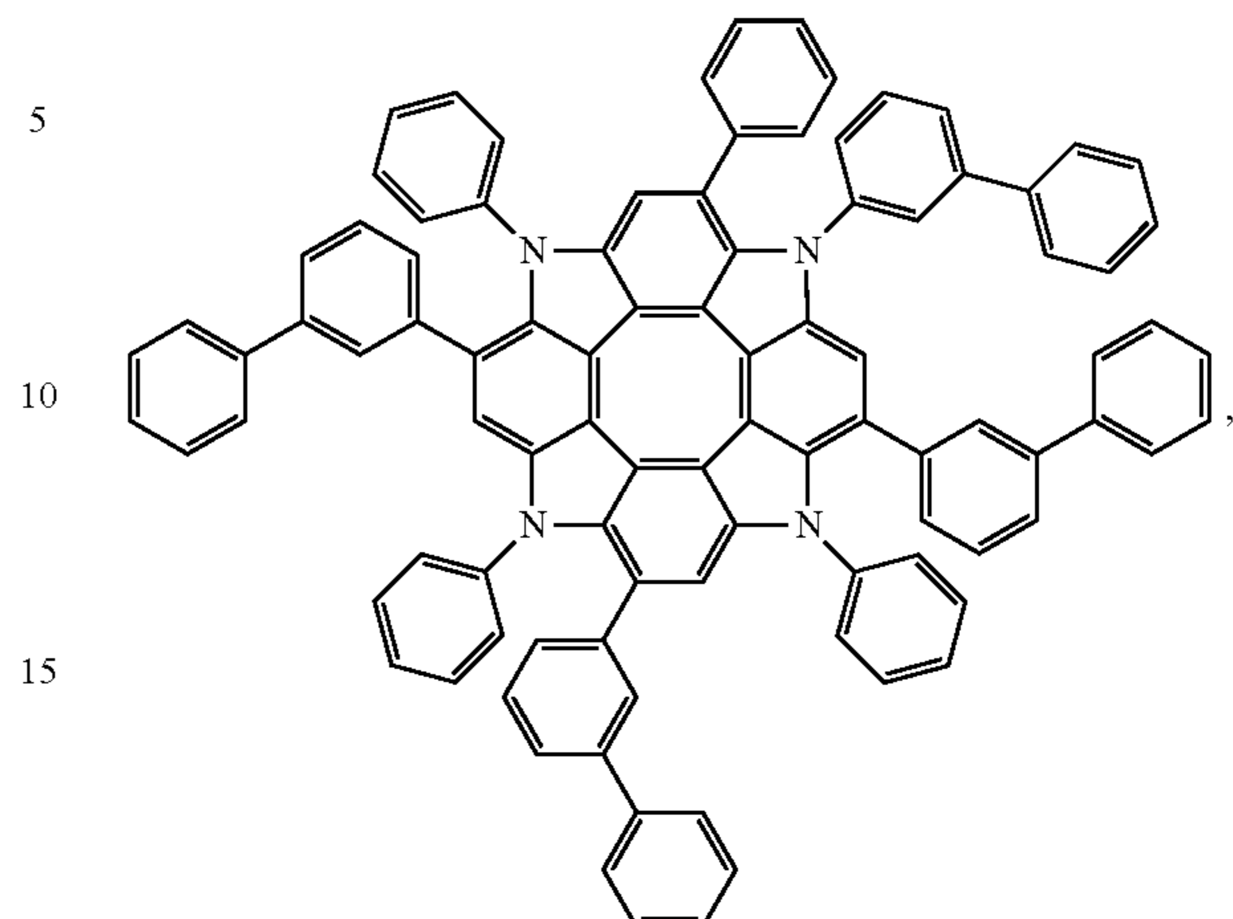
Compound 122
