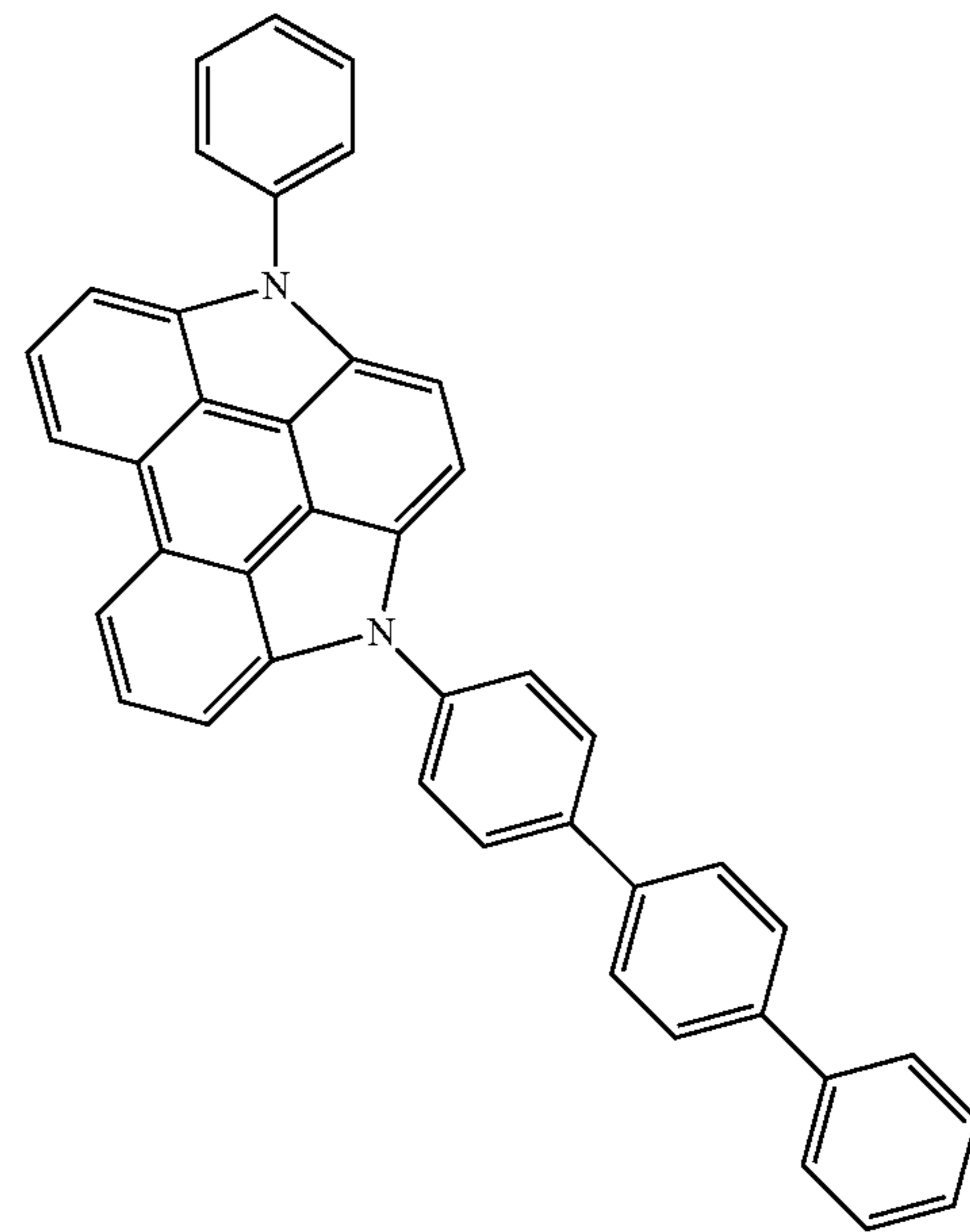
Compound 139
