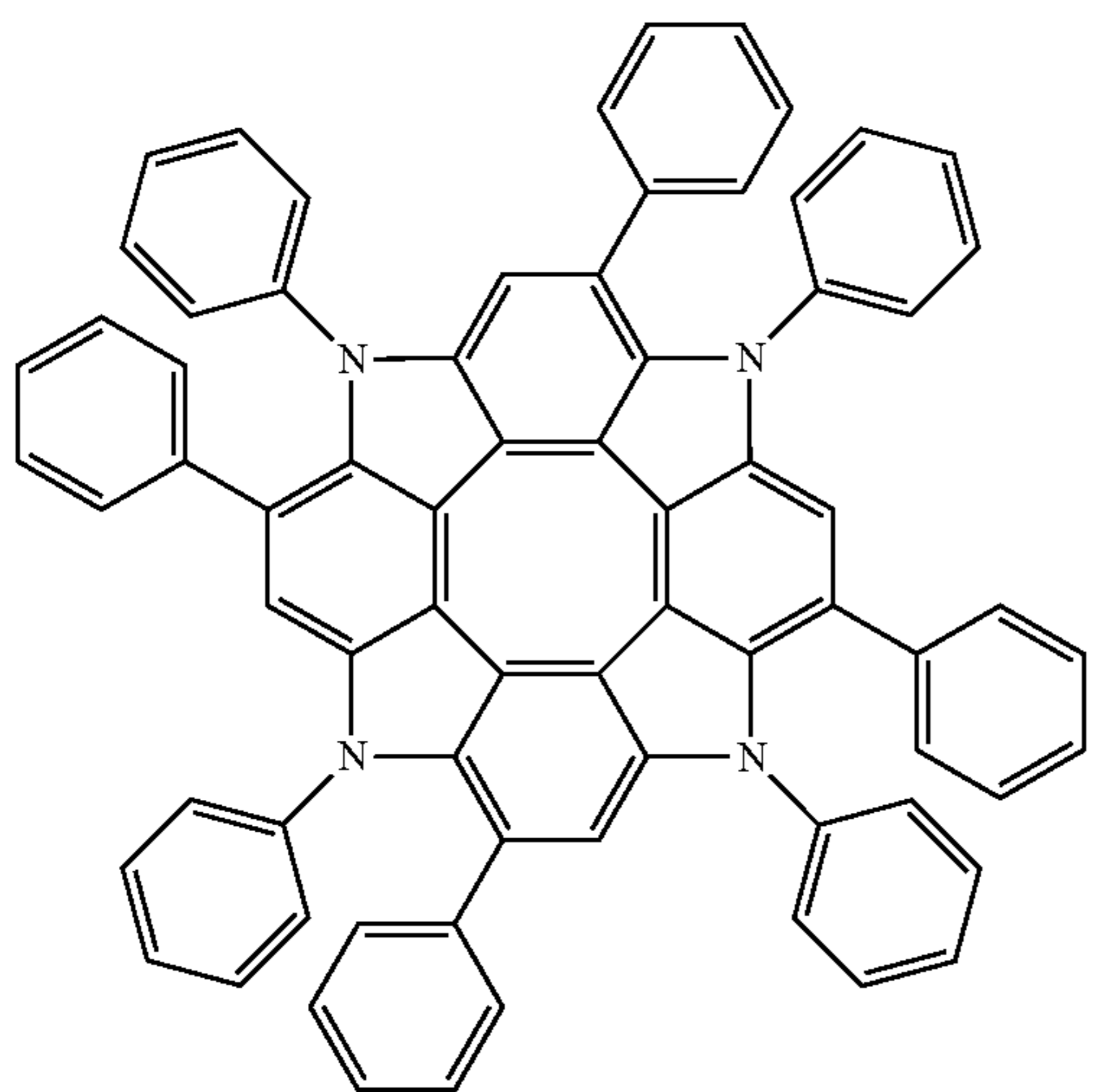
Compound 121
