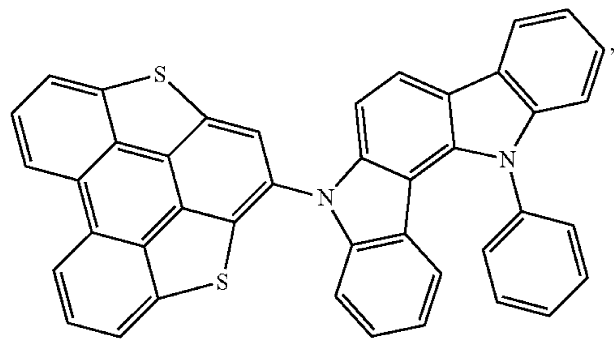
Compound 136
