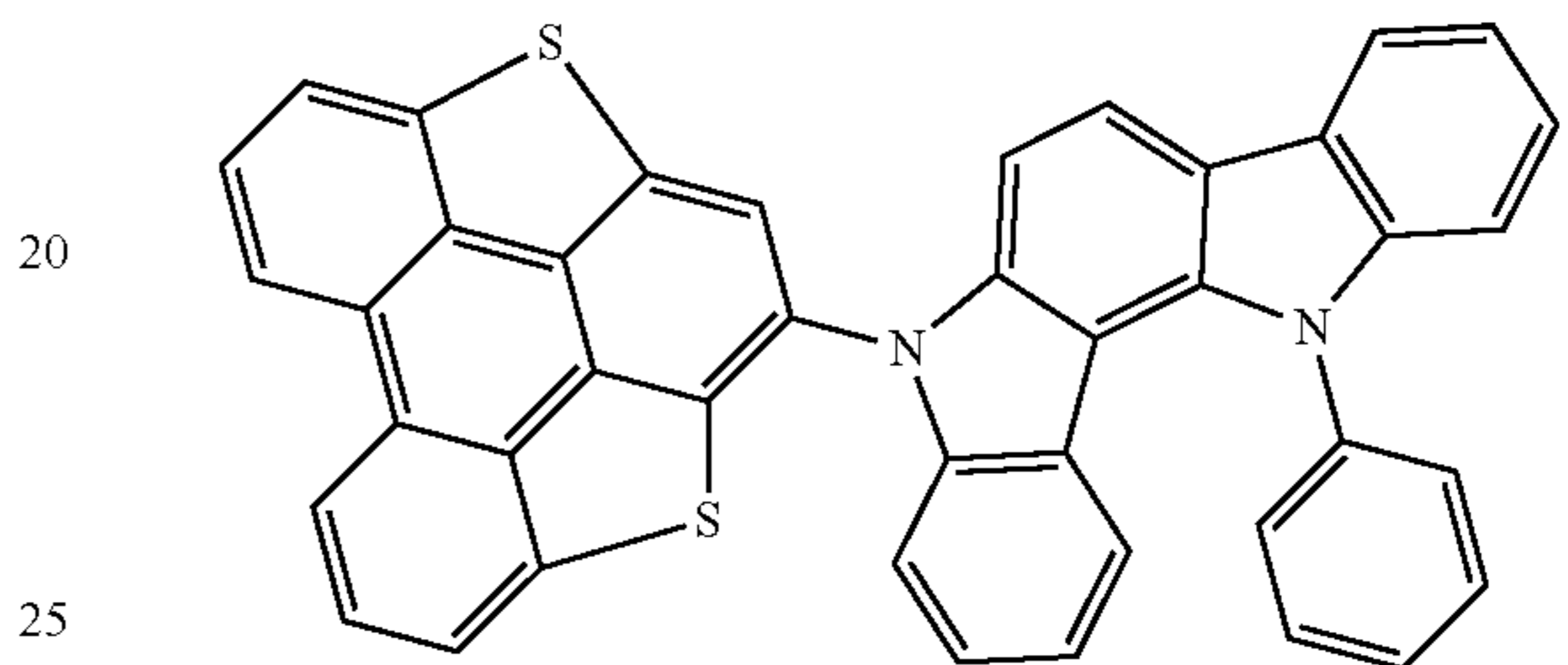
Compound 136
