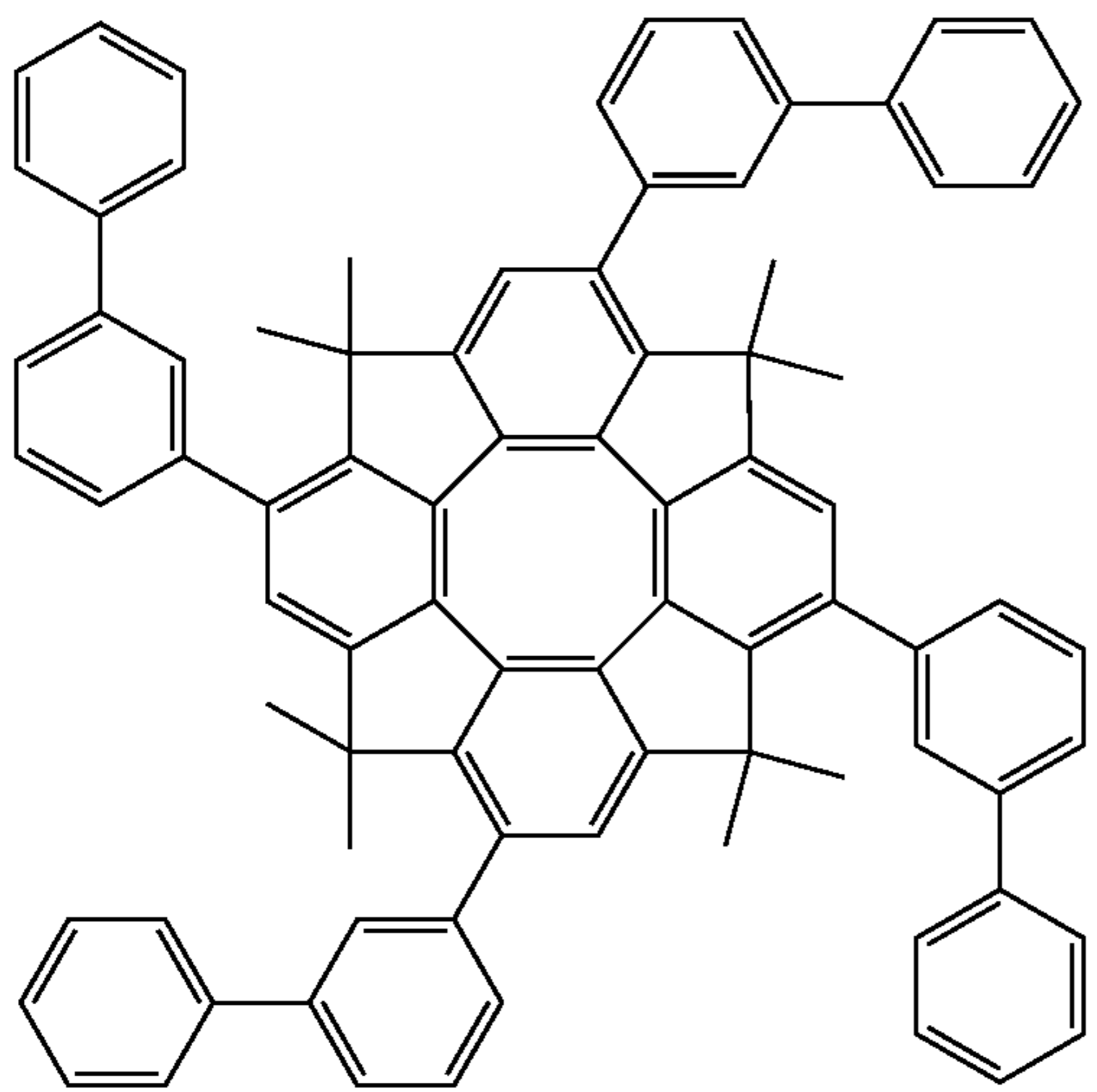
Compound 120
