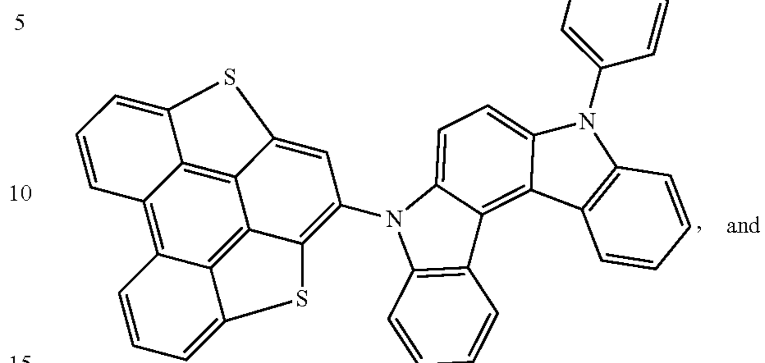
Compound 136
