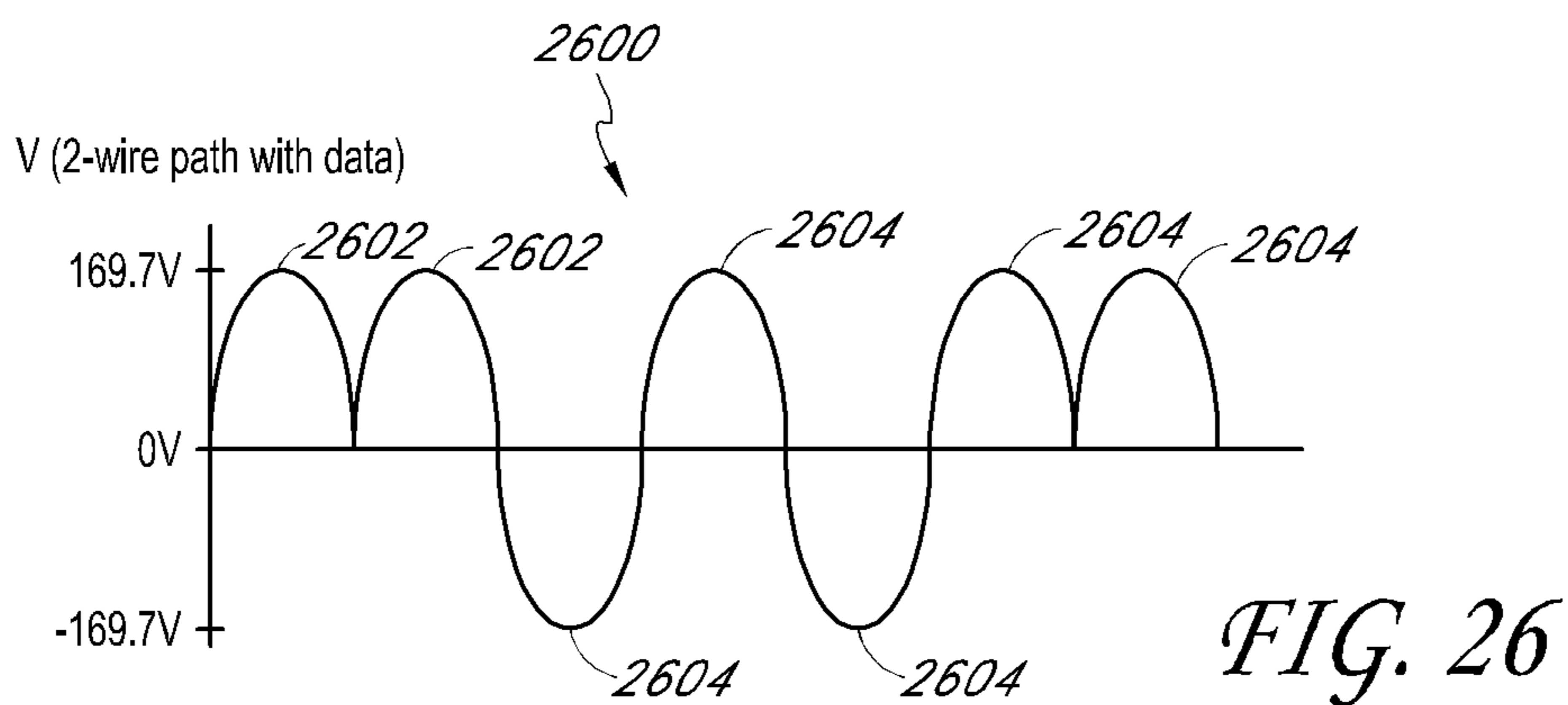
Bridge Waveforms
