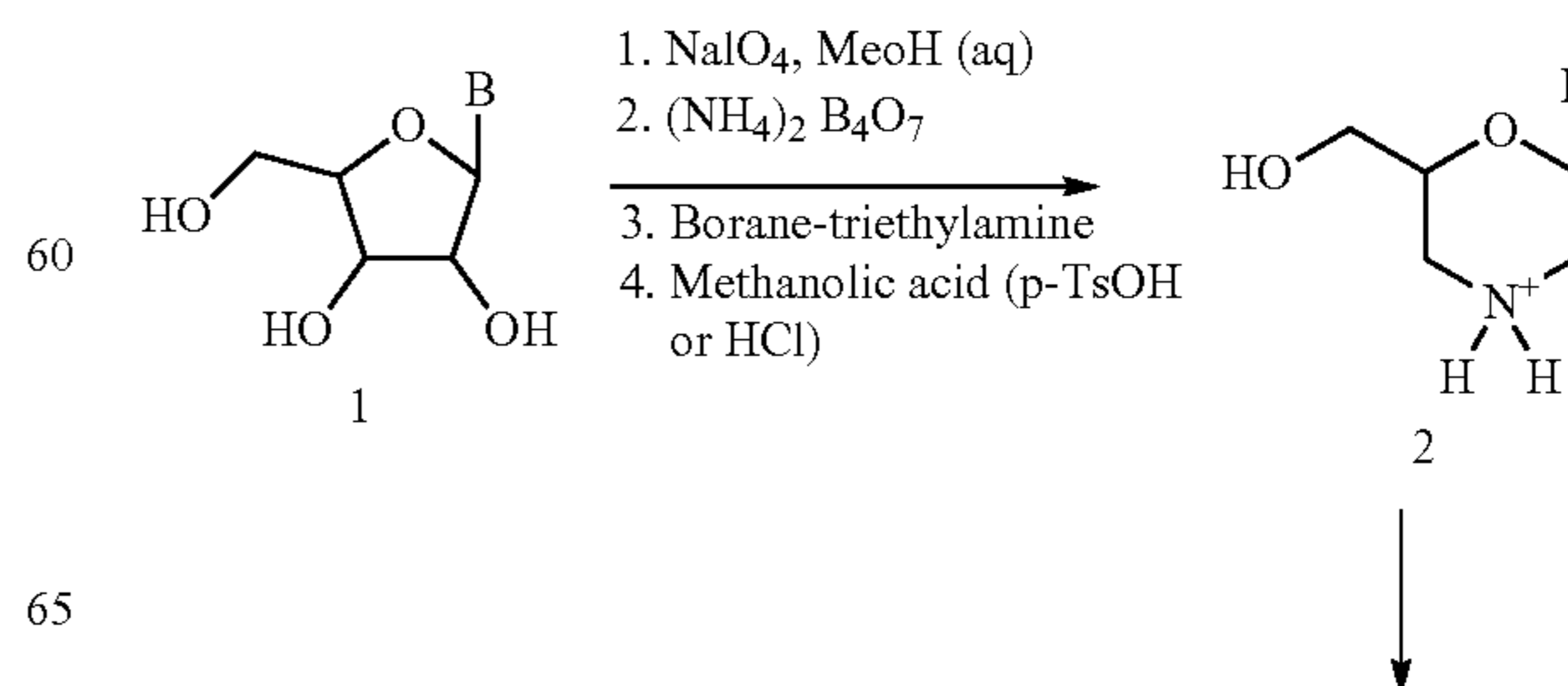
Reaction Scheme 1. Preparation, Protection, and Activation of Morpholino Subunit
