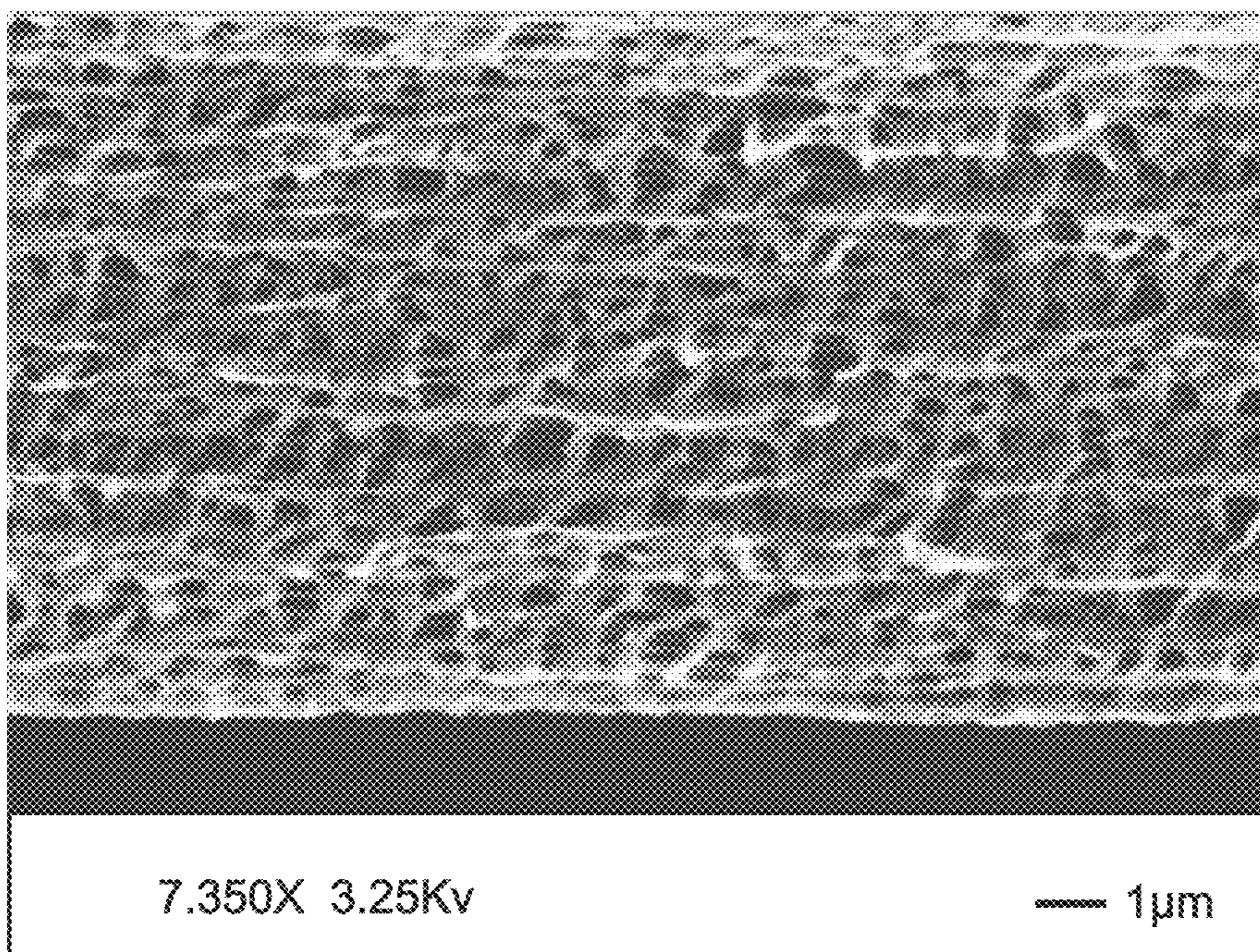
SEM Cross Sectional Micrograph of 8 \mu\text{m} PE1/PE2/PE1 Coextruded Trilayer Microporous Membrane at 7,350 Magnification.
