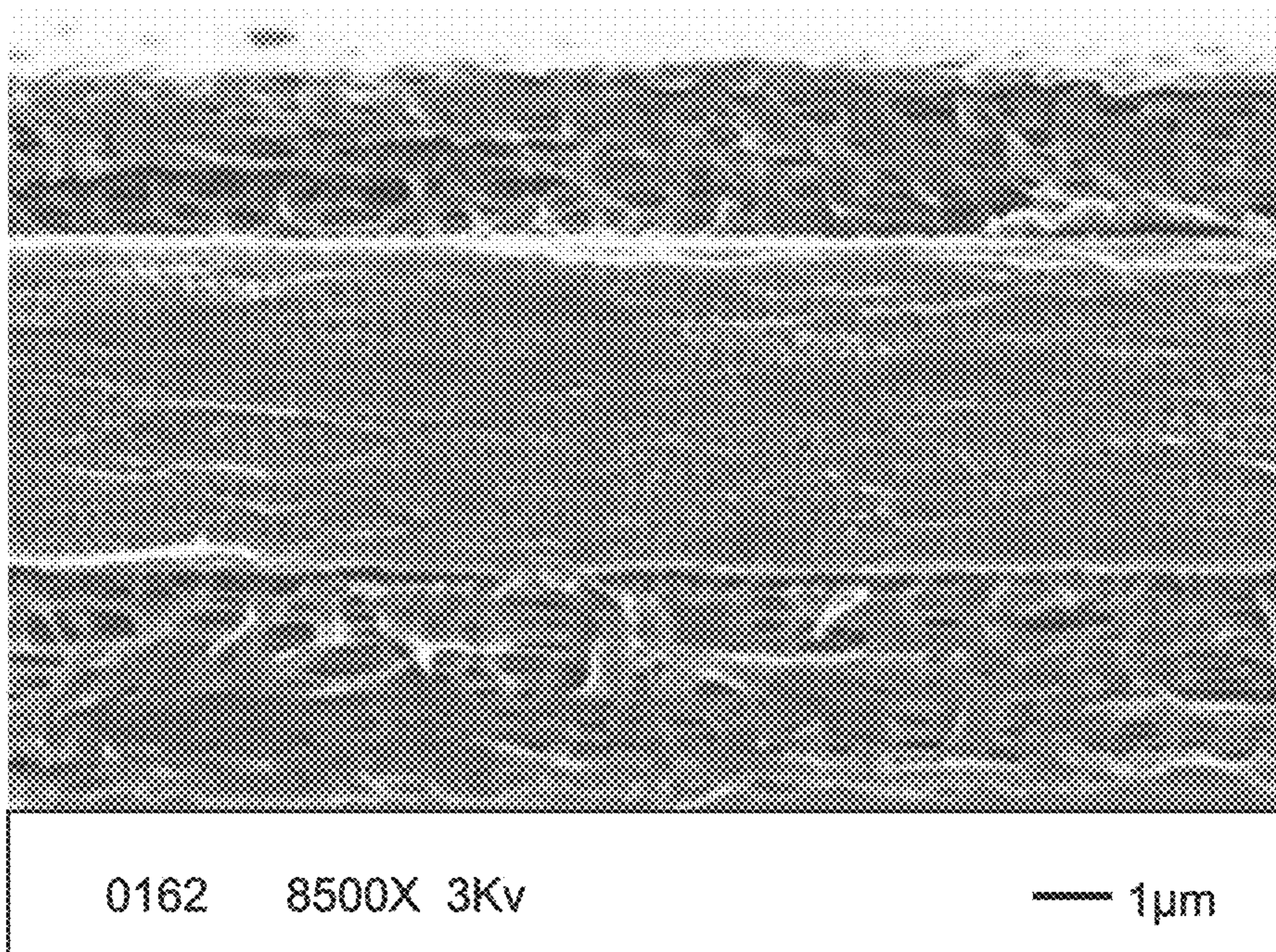
SEM Cross Sectional Micrograph of 9 \mu\text{m} PE/PP/PE Trilayer Microporous Membrane at 8,500 Magnification.
