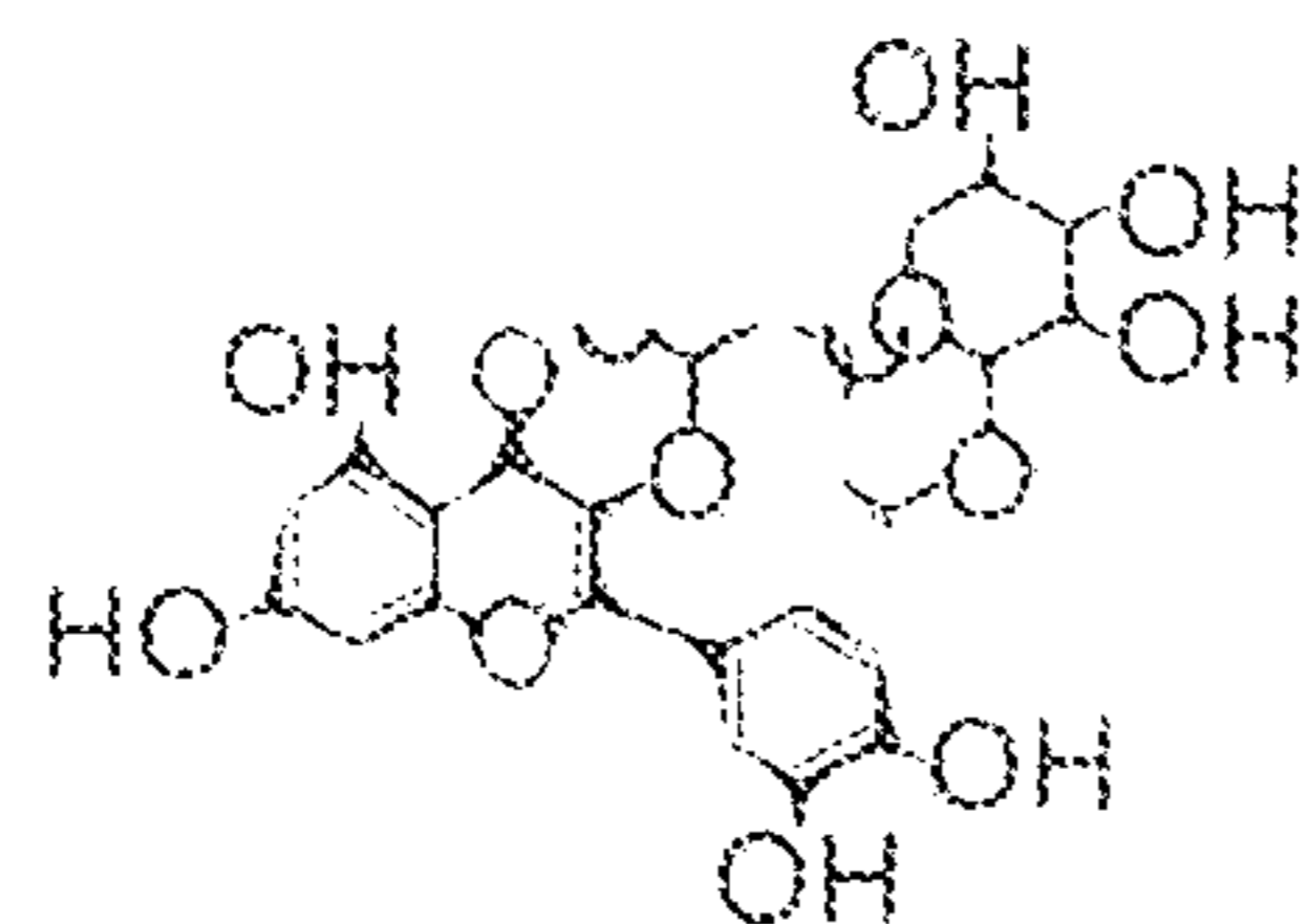
Quercetin 3-xylopyranoside
