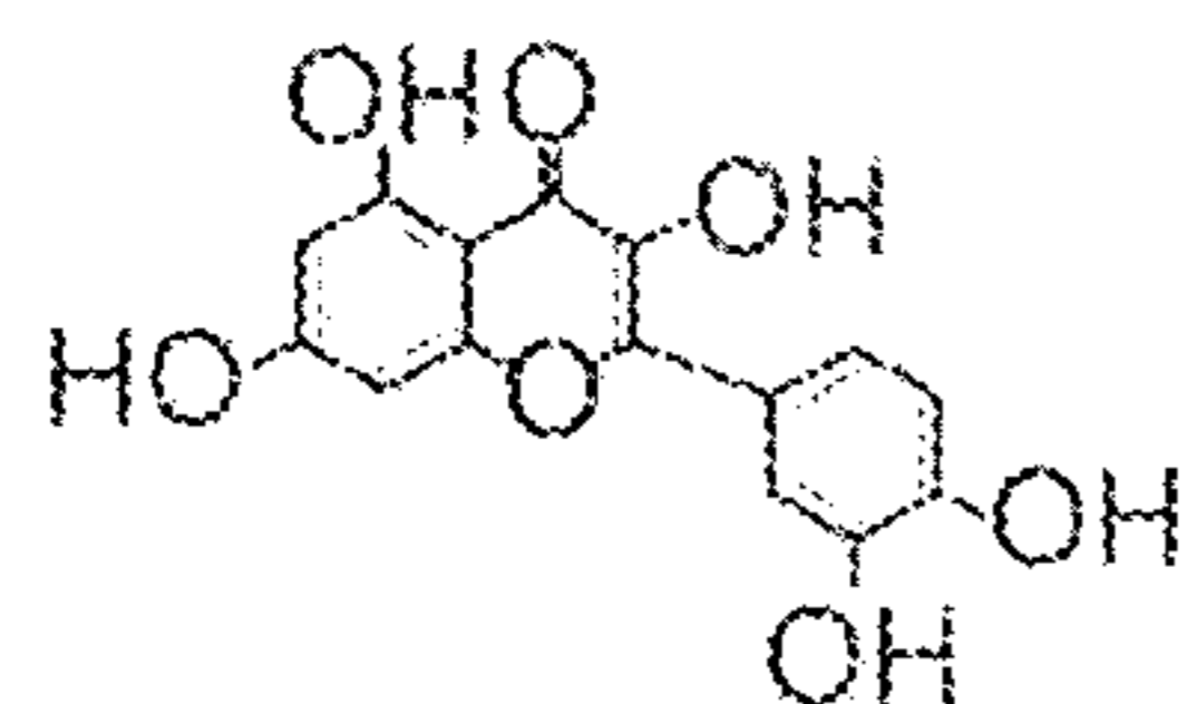
Quercetin
