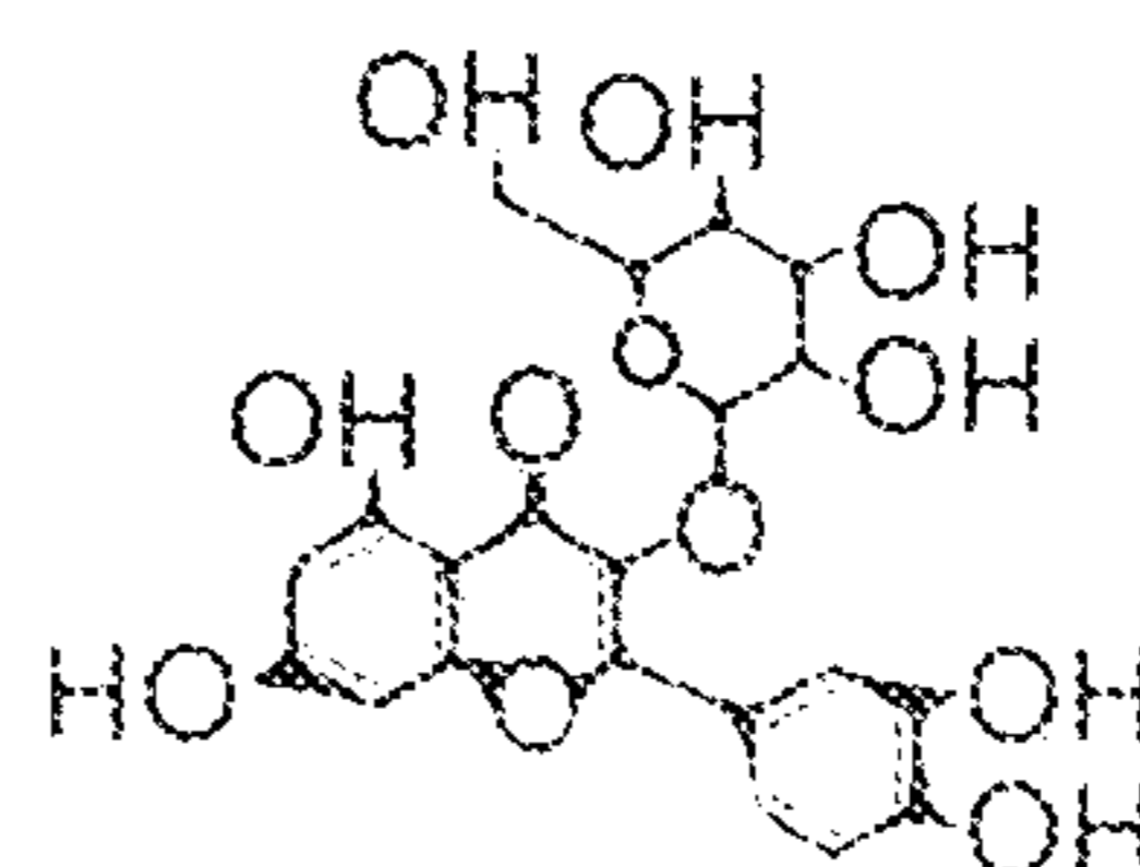
Isoquercetin
