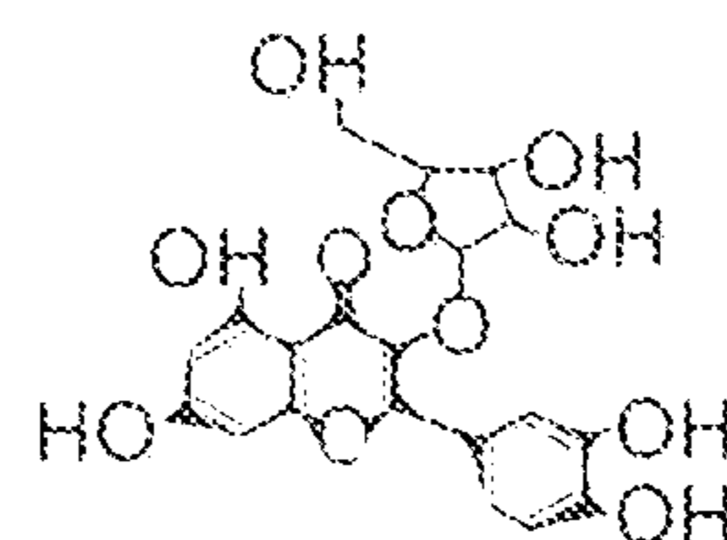
Avicularin
