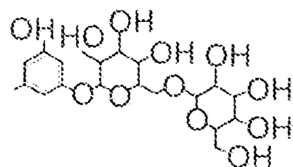
Anacardoside
