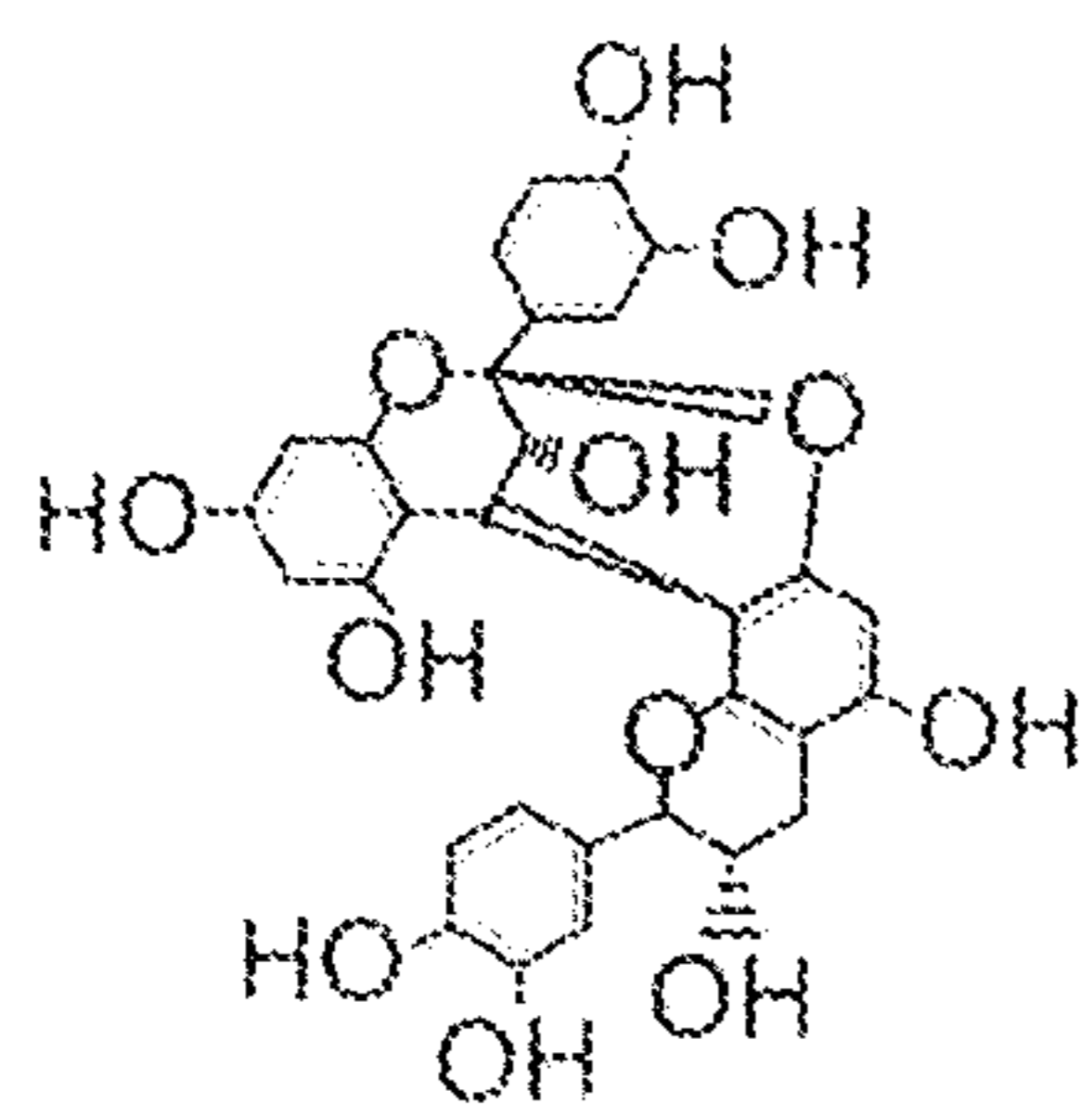
Procyanidin A1
