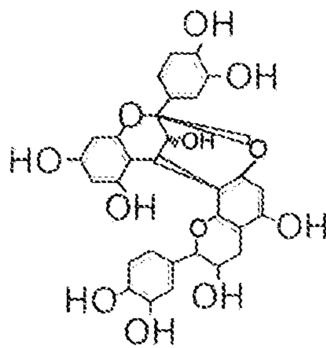
Procyanidin A2
