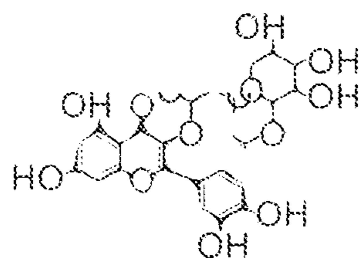
Quercetin 3-xylopyranoside
