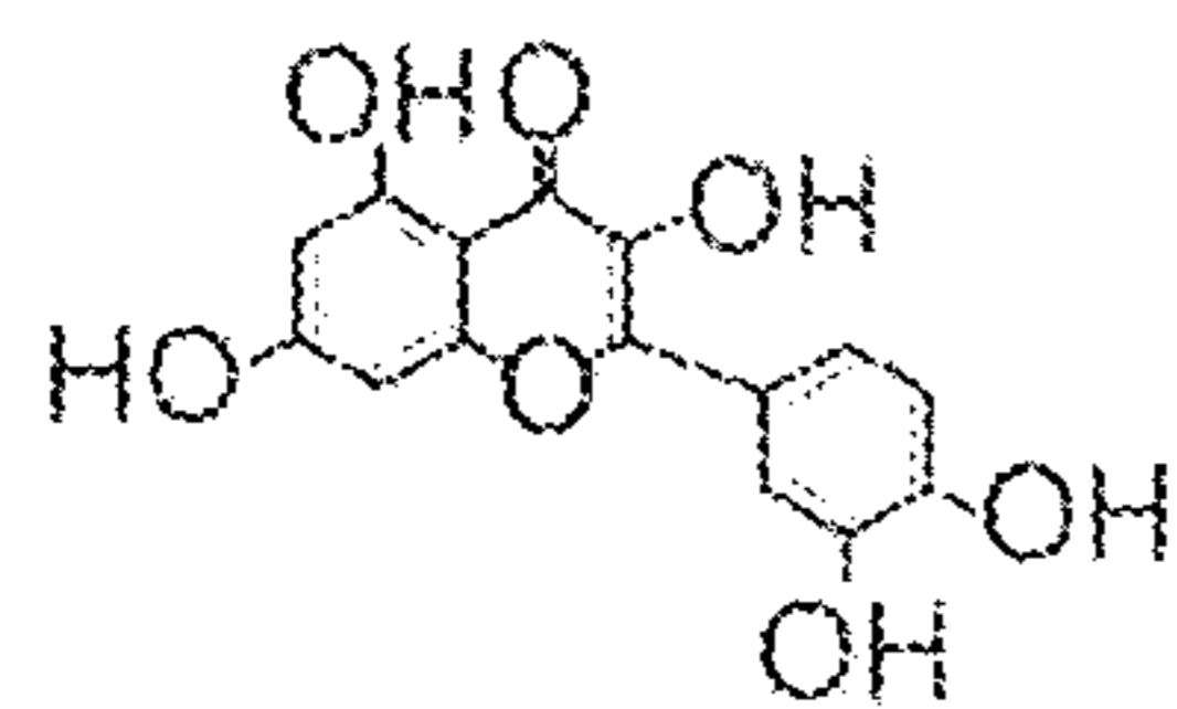
Quercetin
