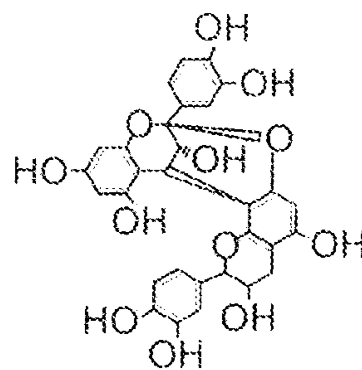
Procyanidin A2
