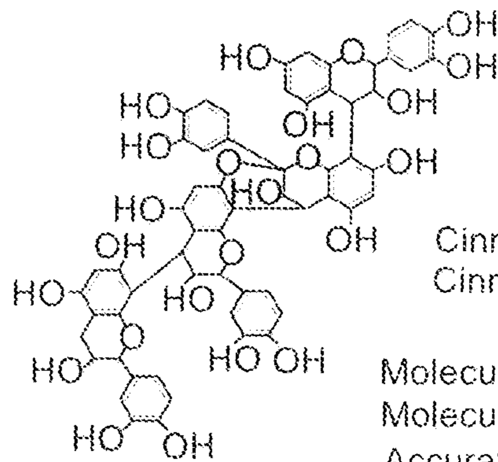
Epicatechin-(2 \beta -7,4 \beta -8)-epicatechin- (4 \beta -8)-epicatechin
