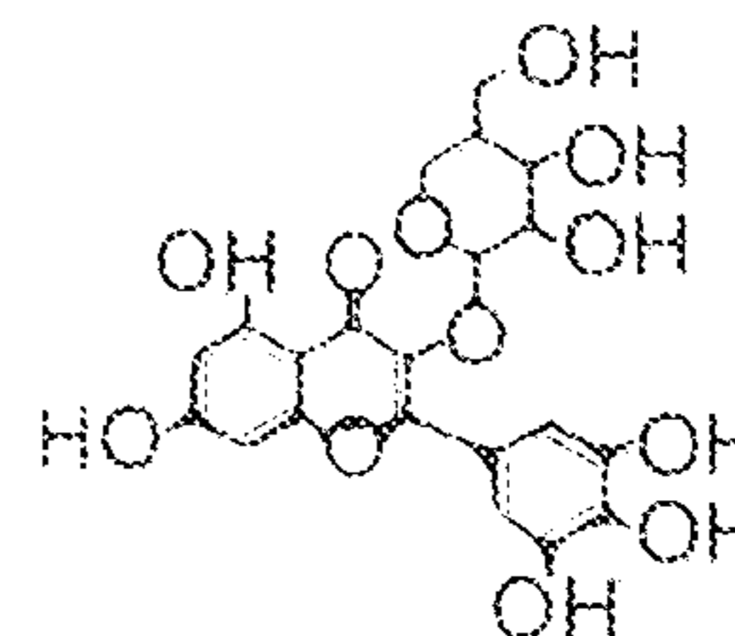
Myricetin 3-arabinofuranoside
