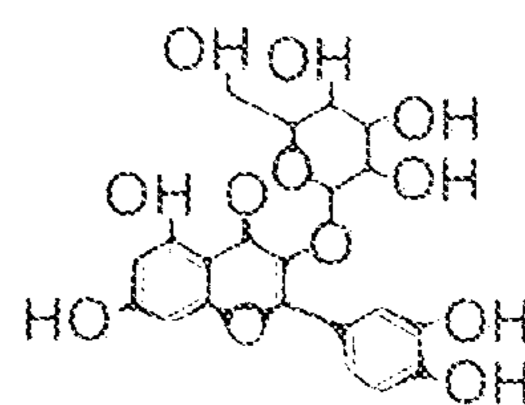
Myricetin 3-arabinofuranoside
