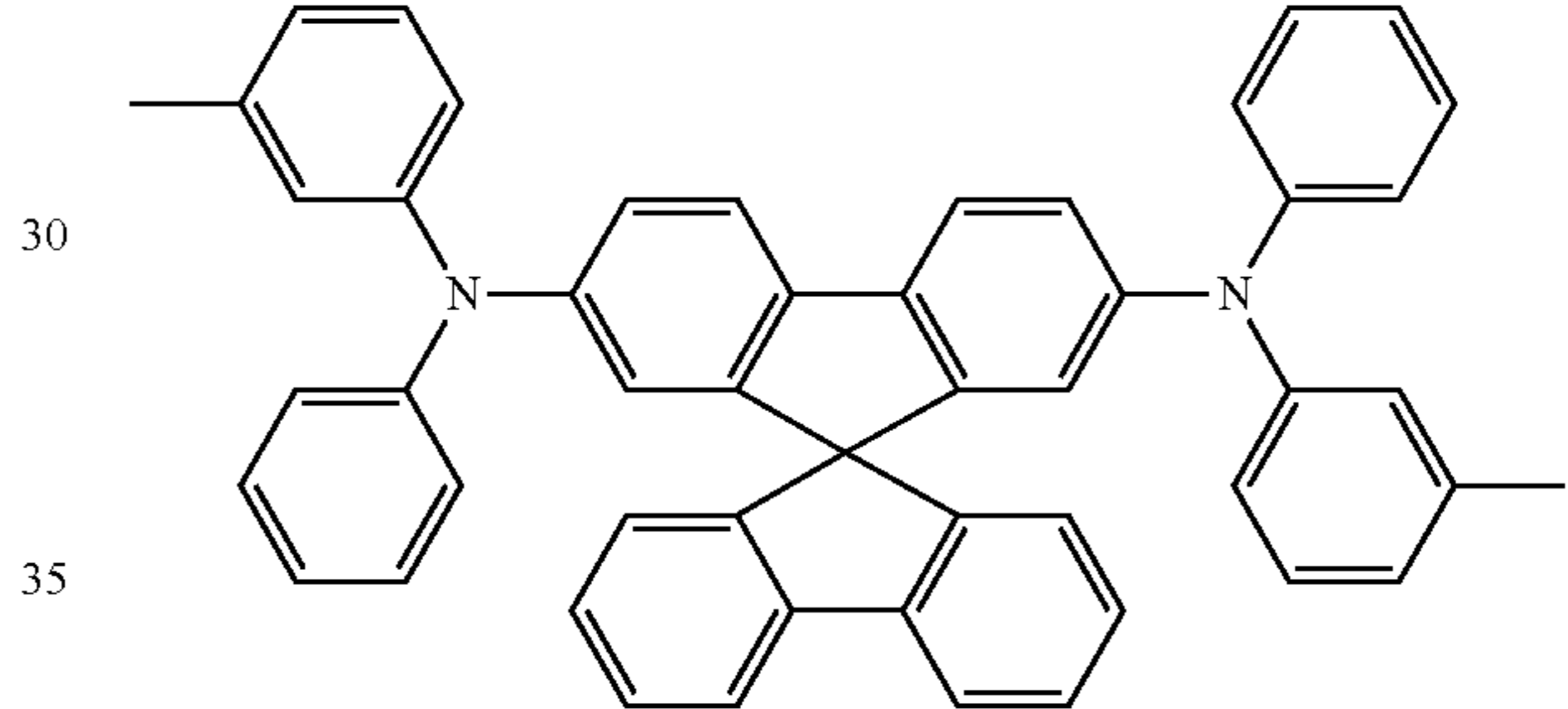
Spiro-TPD
