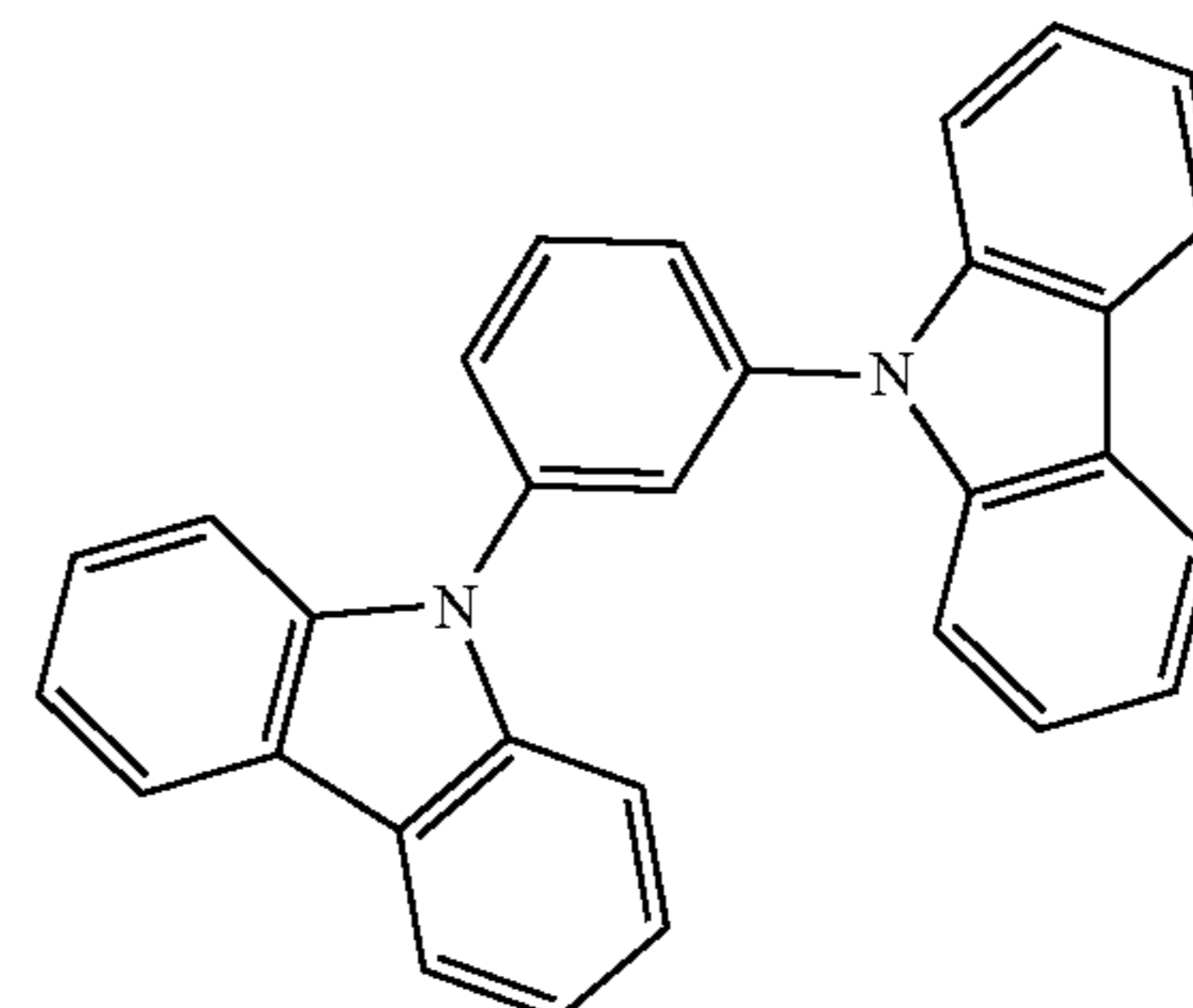
mCP
