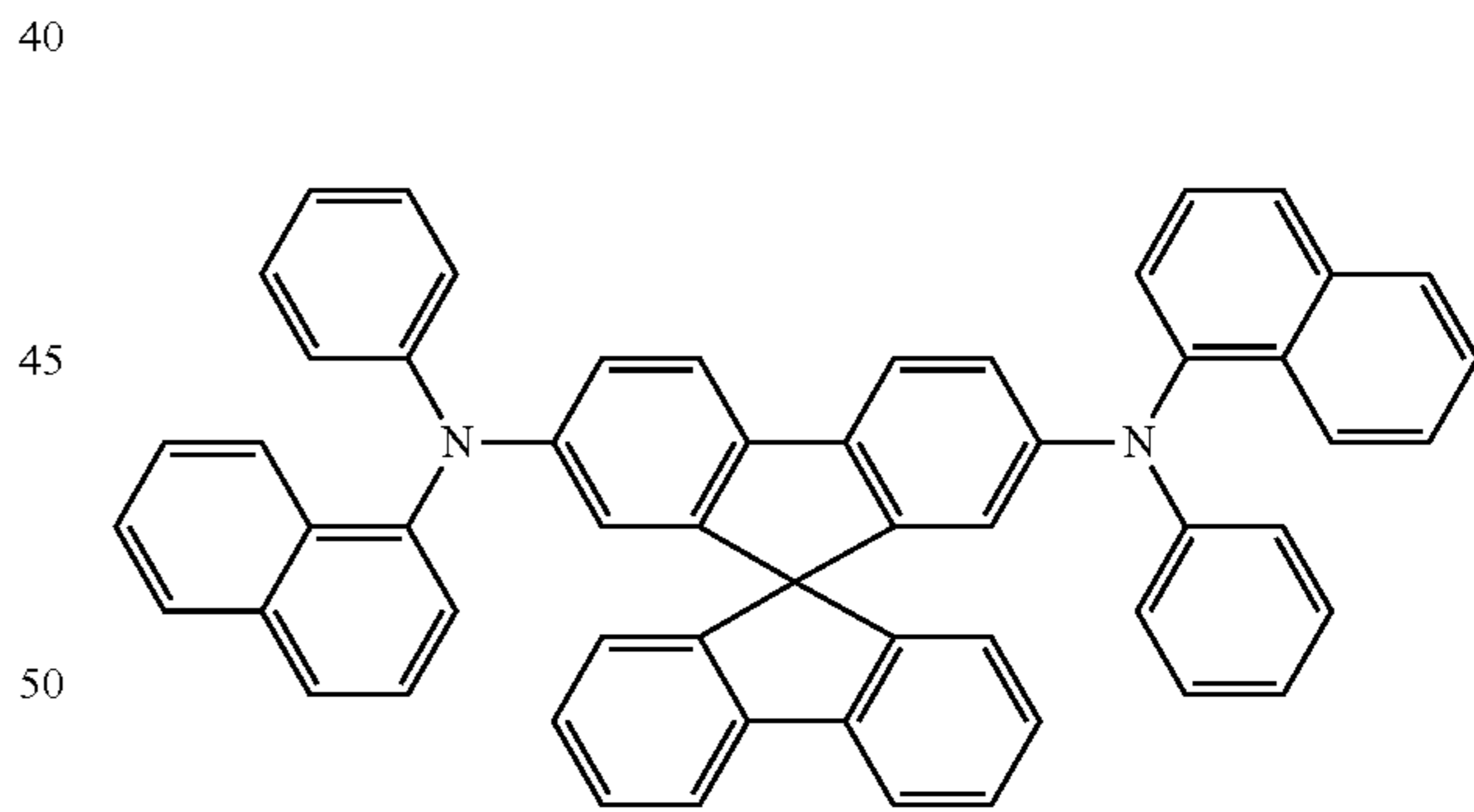
Spiro-NPB
