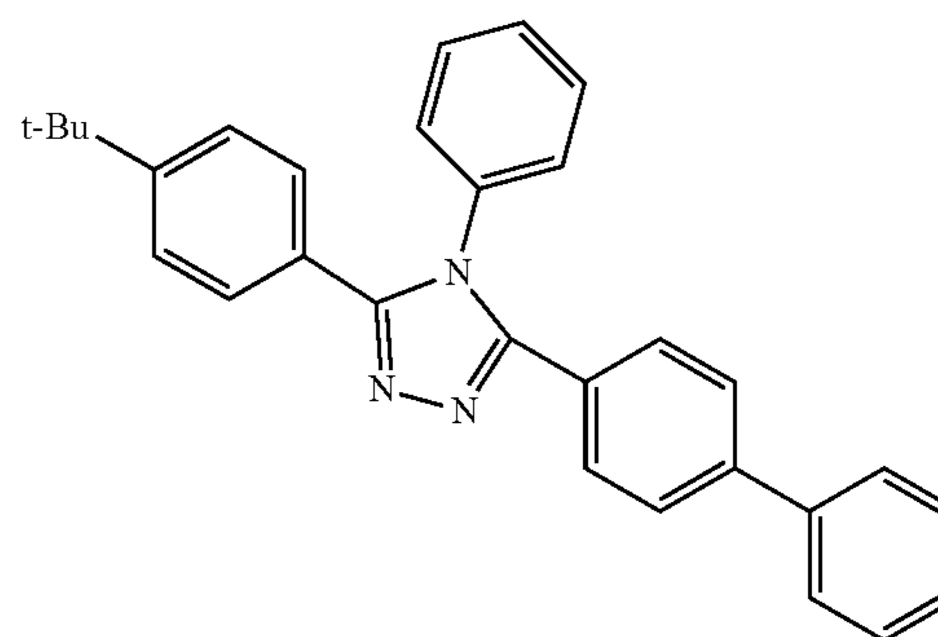
TAZ
