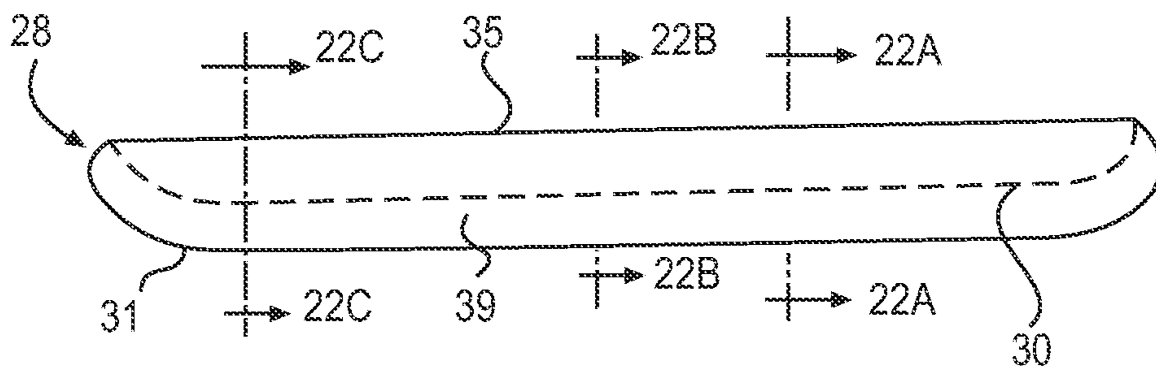
SIDE VIEW
