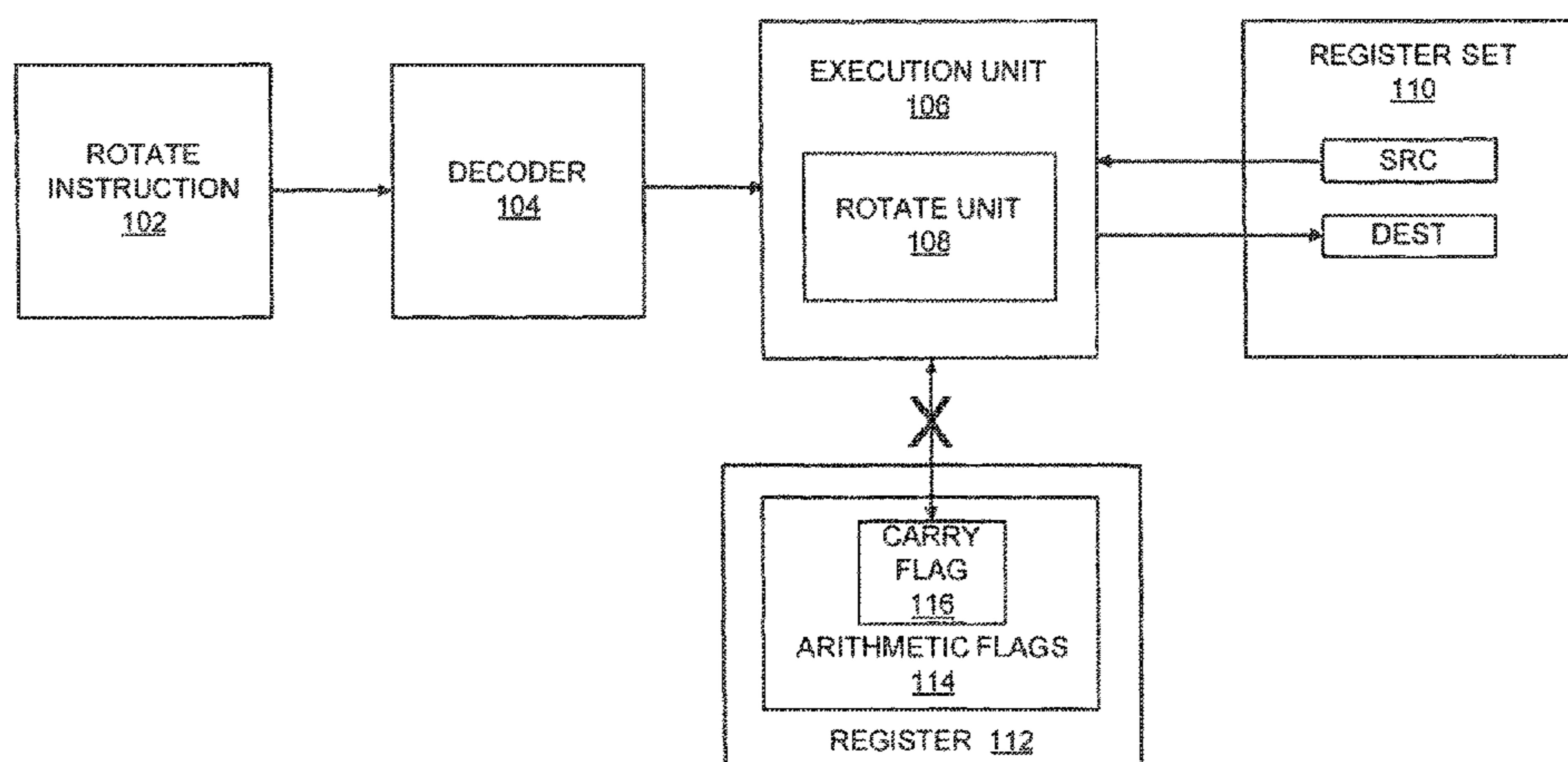
INSTRUCTION PROCESSING APPARATUS 100
