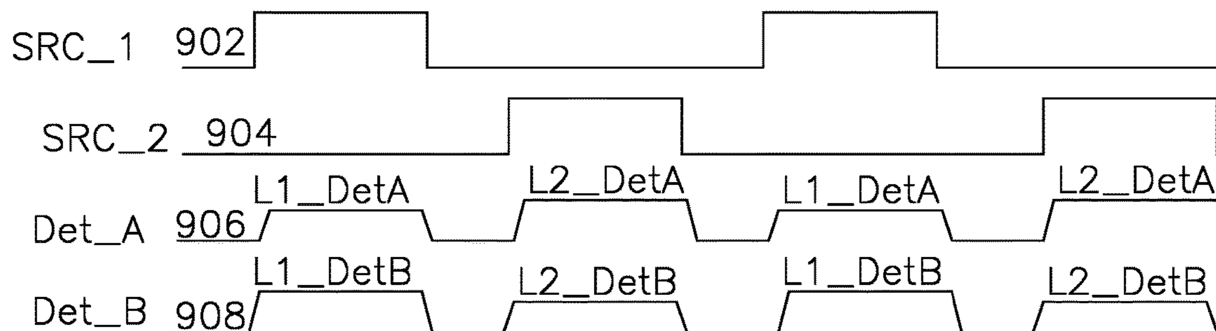
Figure 9 Wavelength Interrogator
