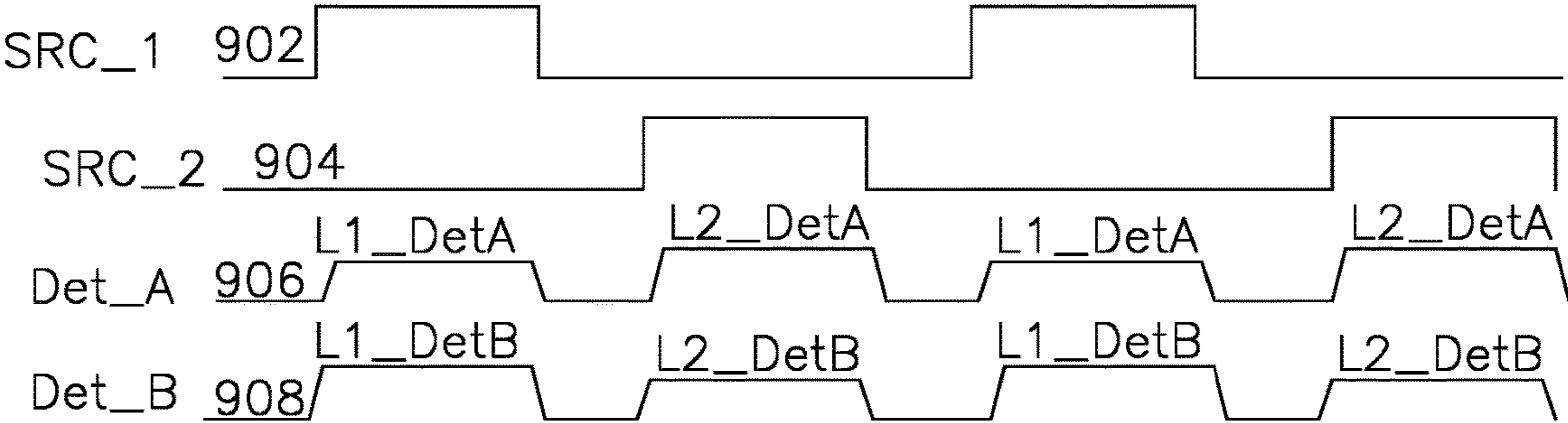
Figure 9 Wavelength Interrogator
