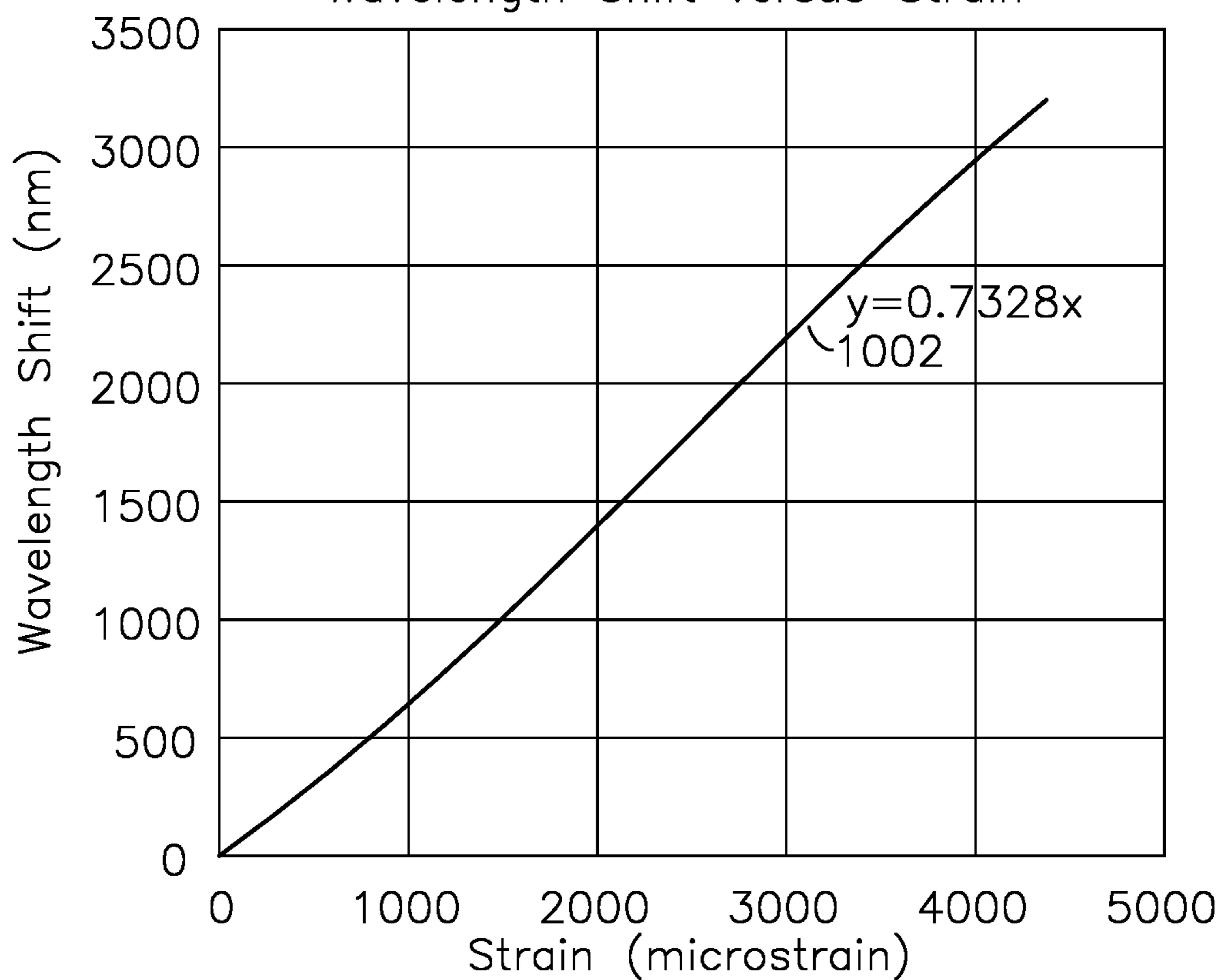
Wavelength Shift versus Strain
