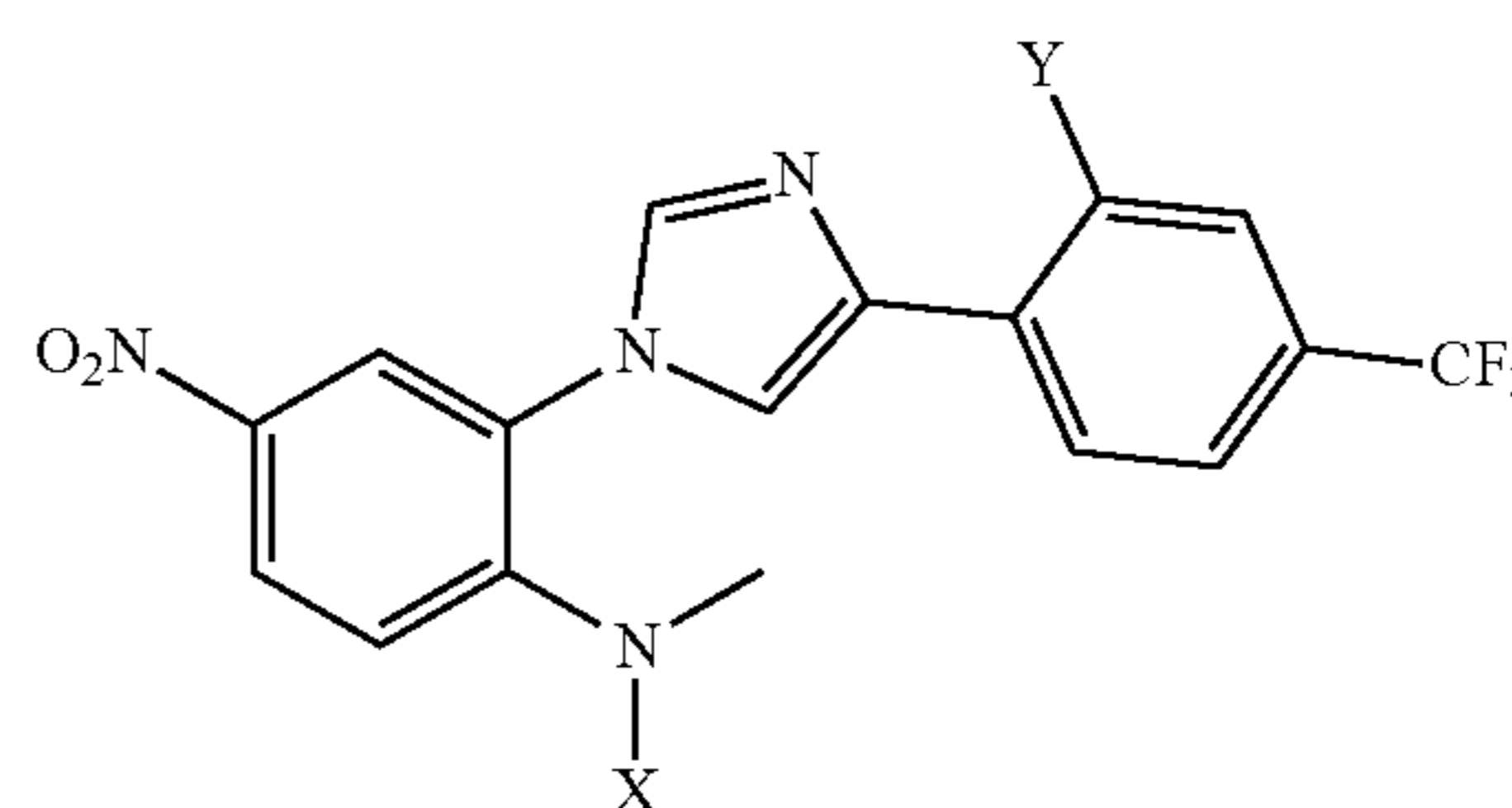
FORMULA I
