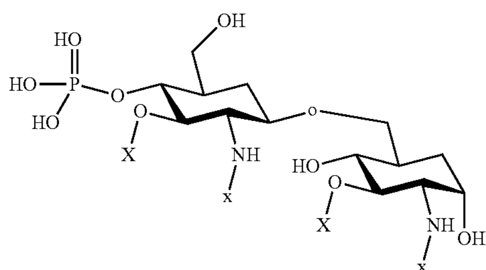
FORMULA III
