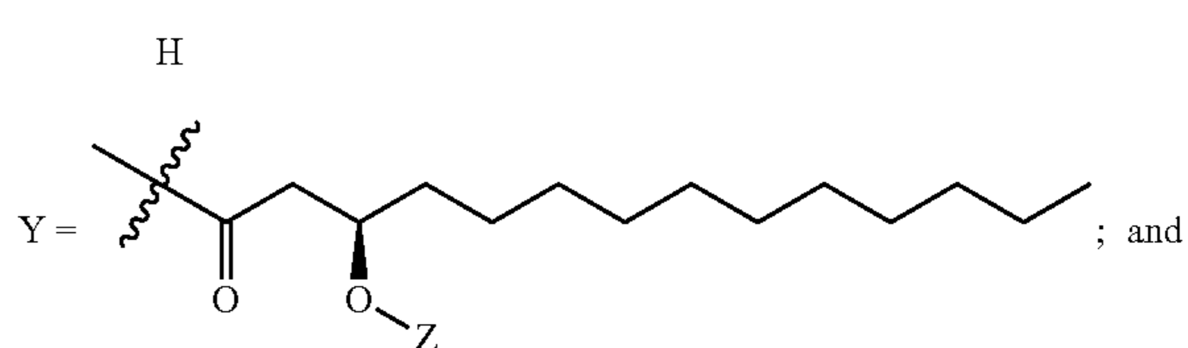
FORMULA III
