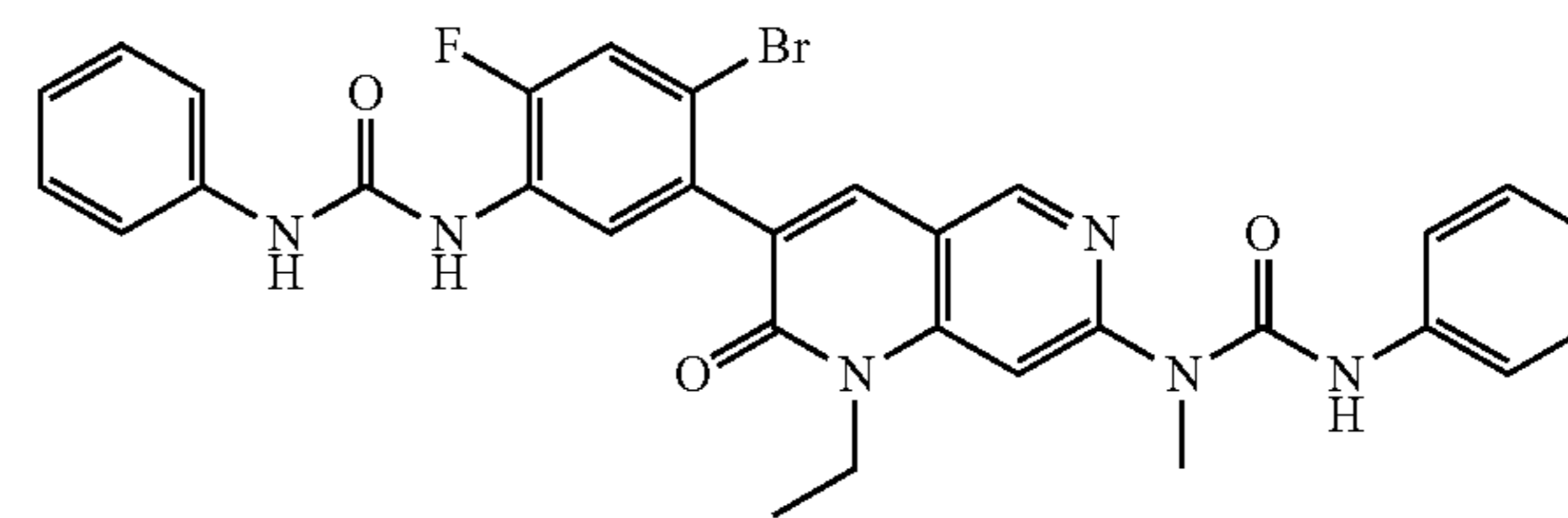
Formula (III)
