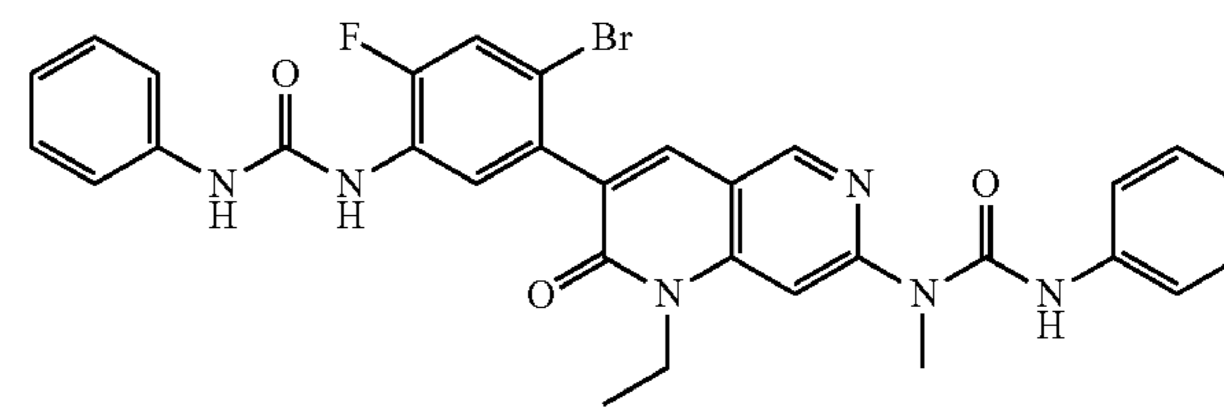
Formula (III)
