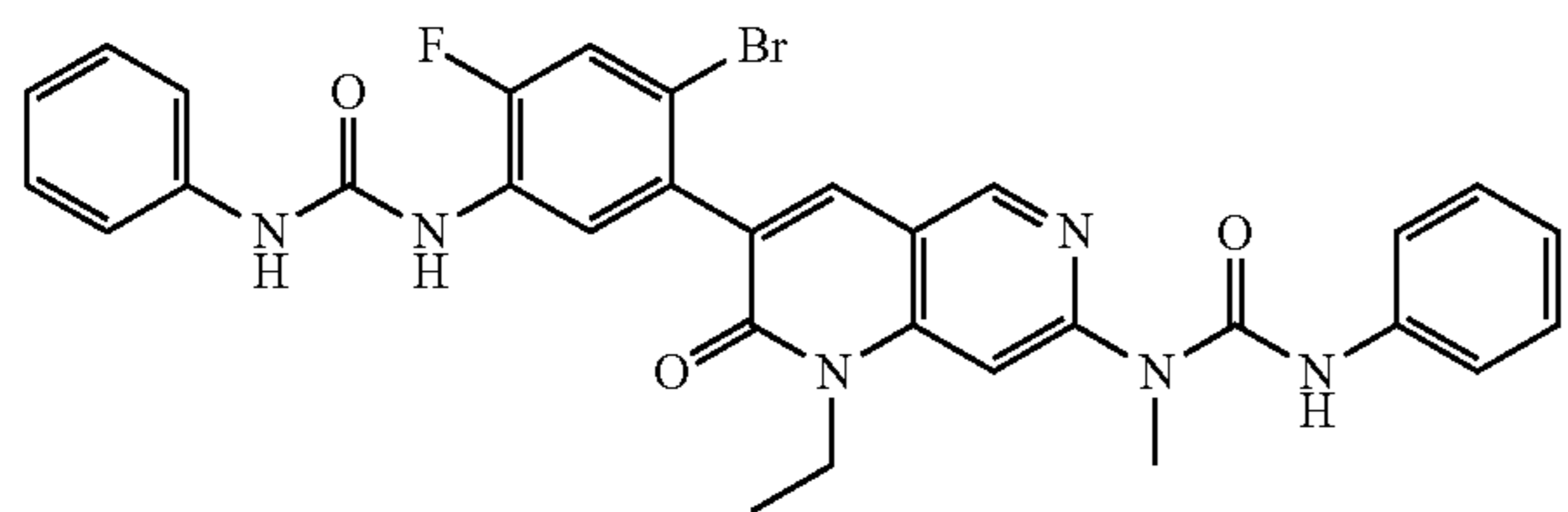
Formula (III)
