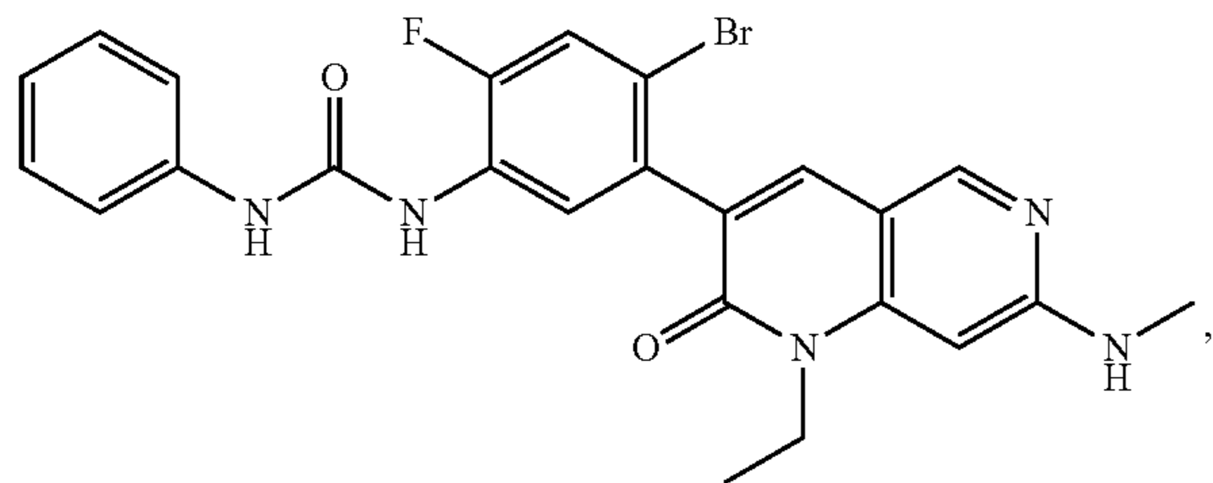
Formula (I)
