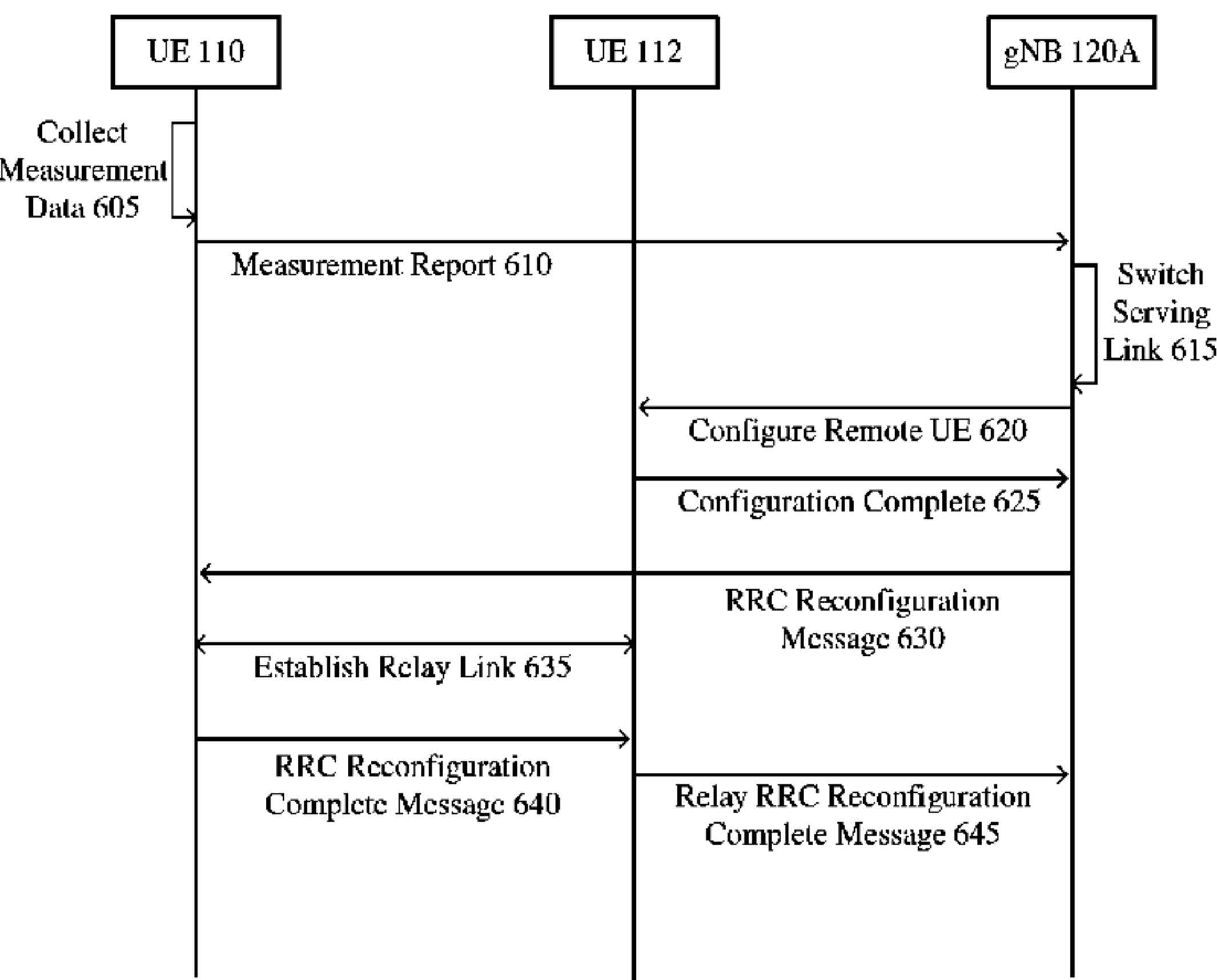
Signaling Diagram 600
