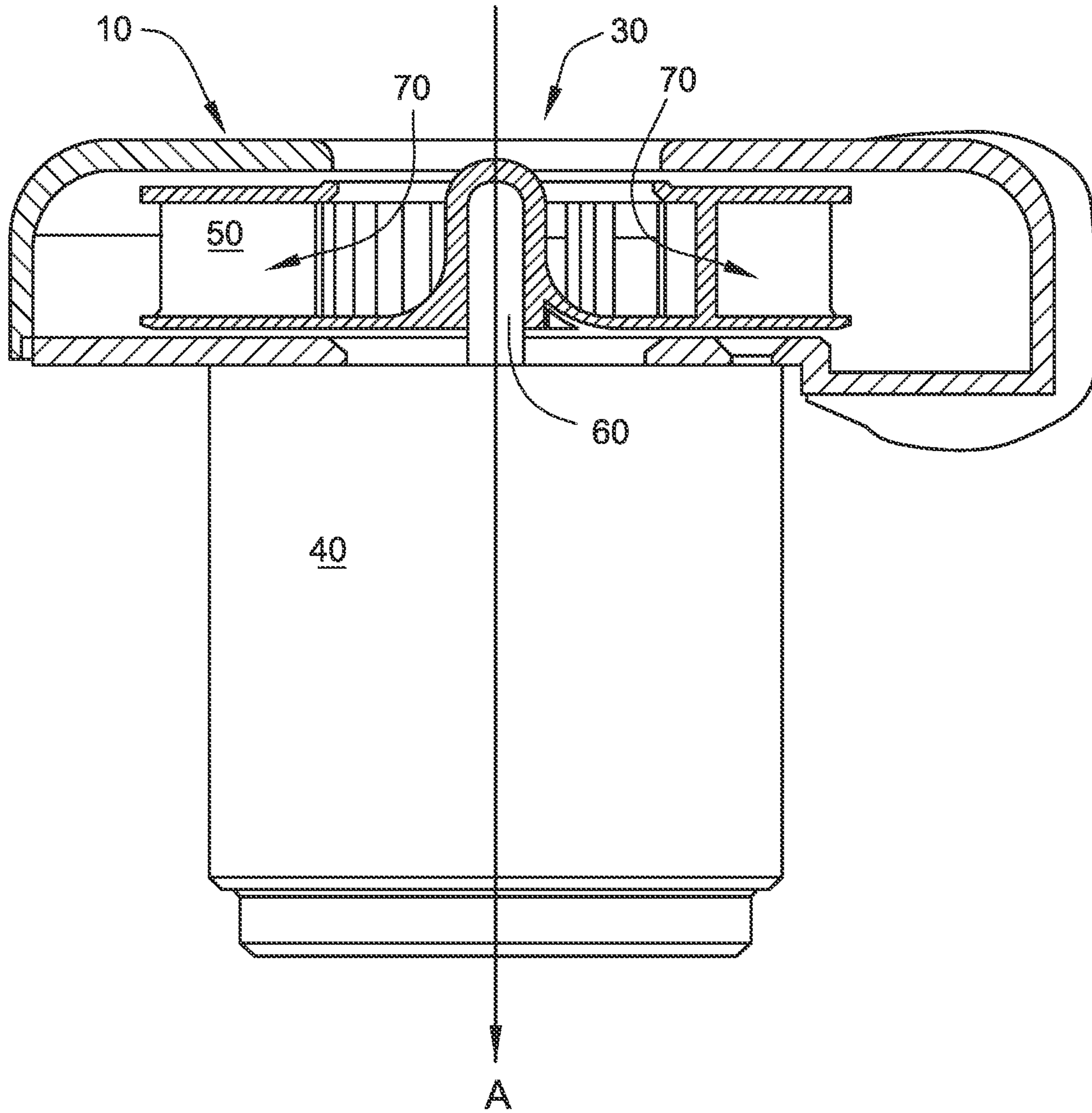
FIG. 2 (PRIOR ART)
