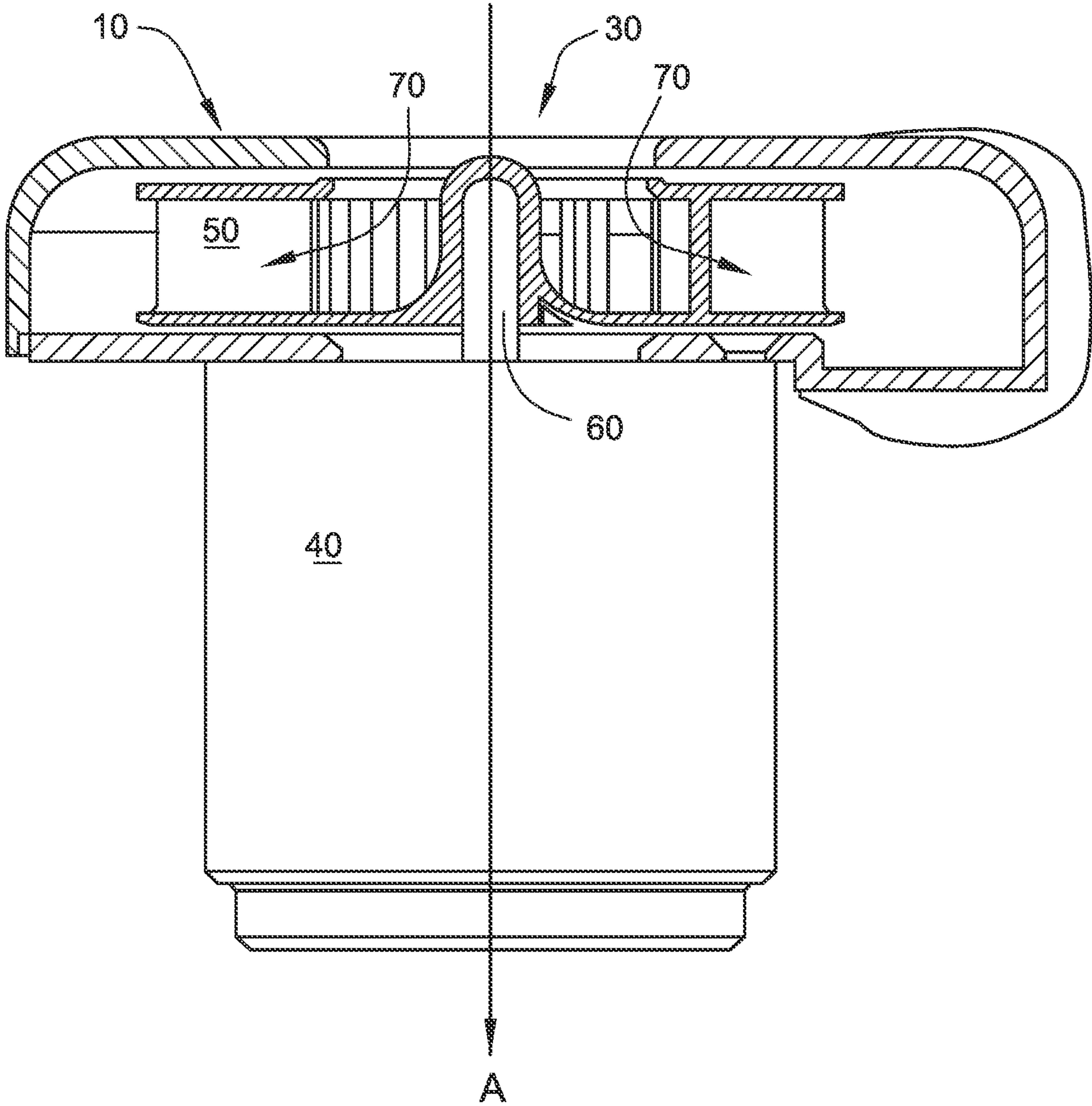
FIG. 2 (PRIOR ART)
