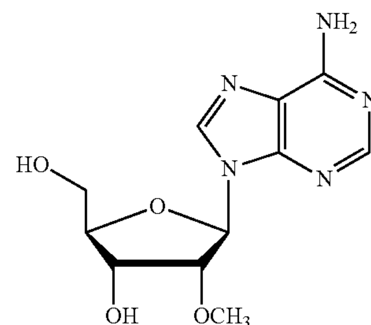
2'-O-methyl-adenosine
