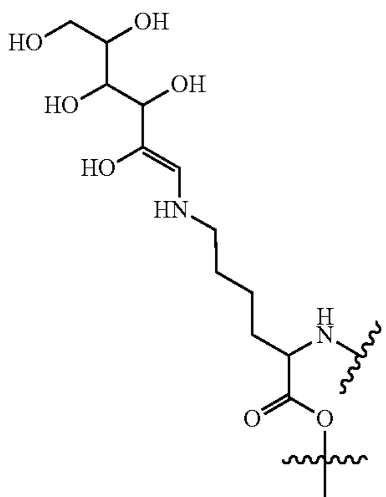
glycated lysine (enol tautomer)
