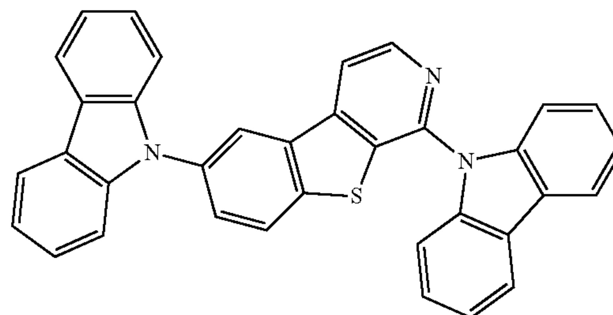
Compound 7
