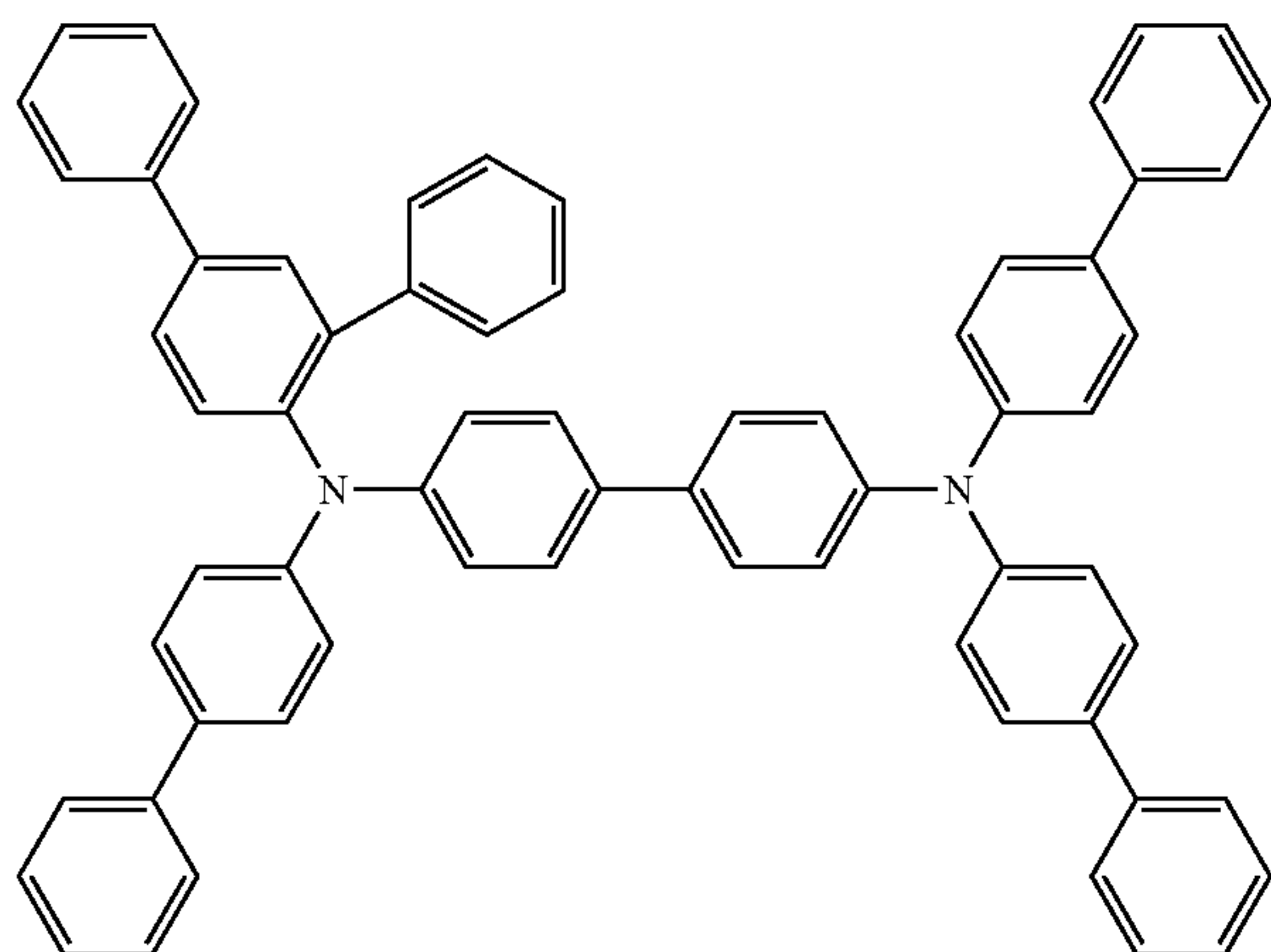
Compound 2
