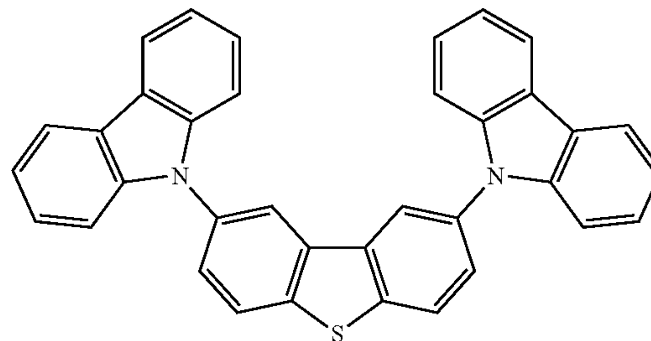
Compound 4
