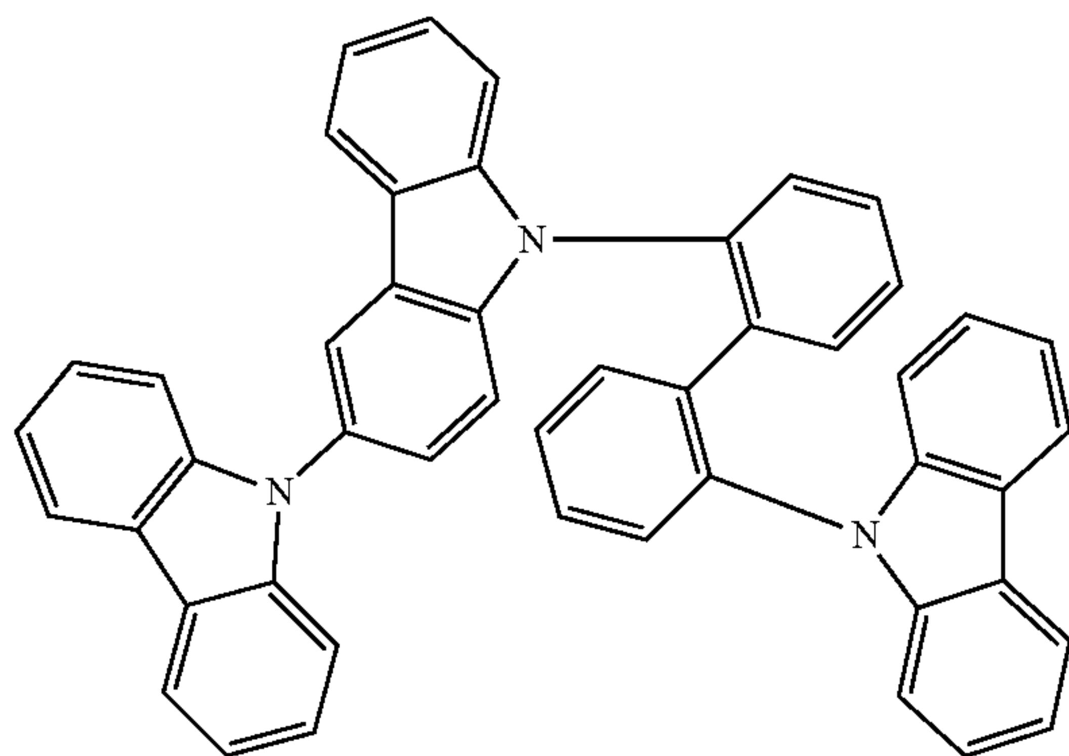
Compound A
