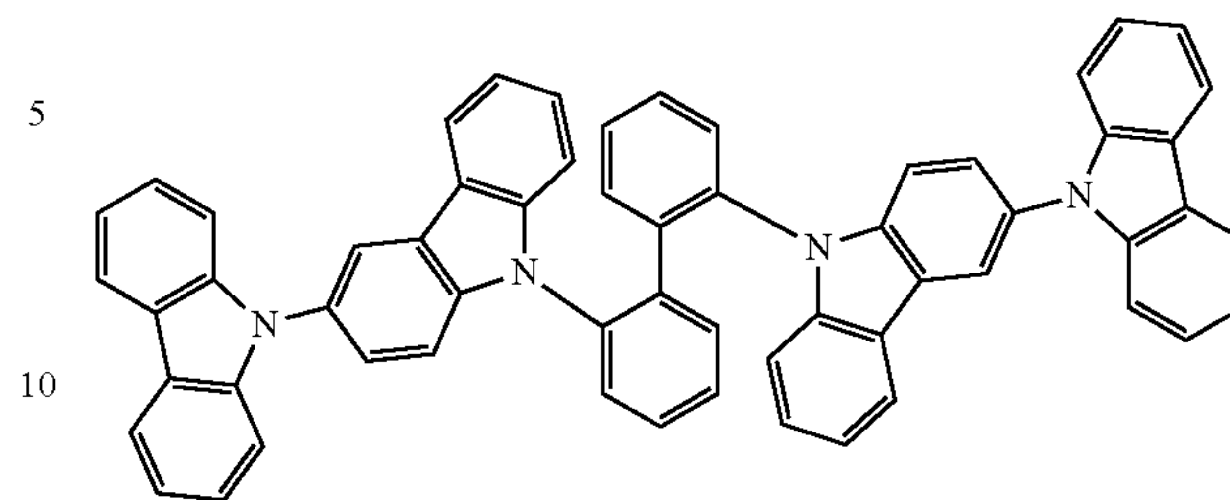
Compound B
