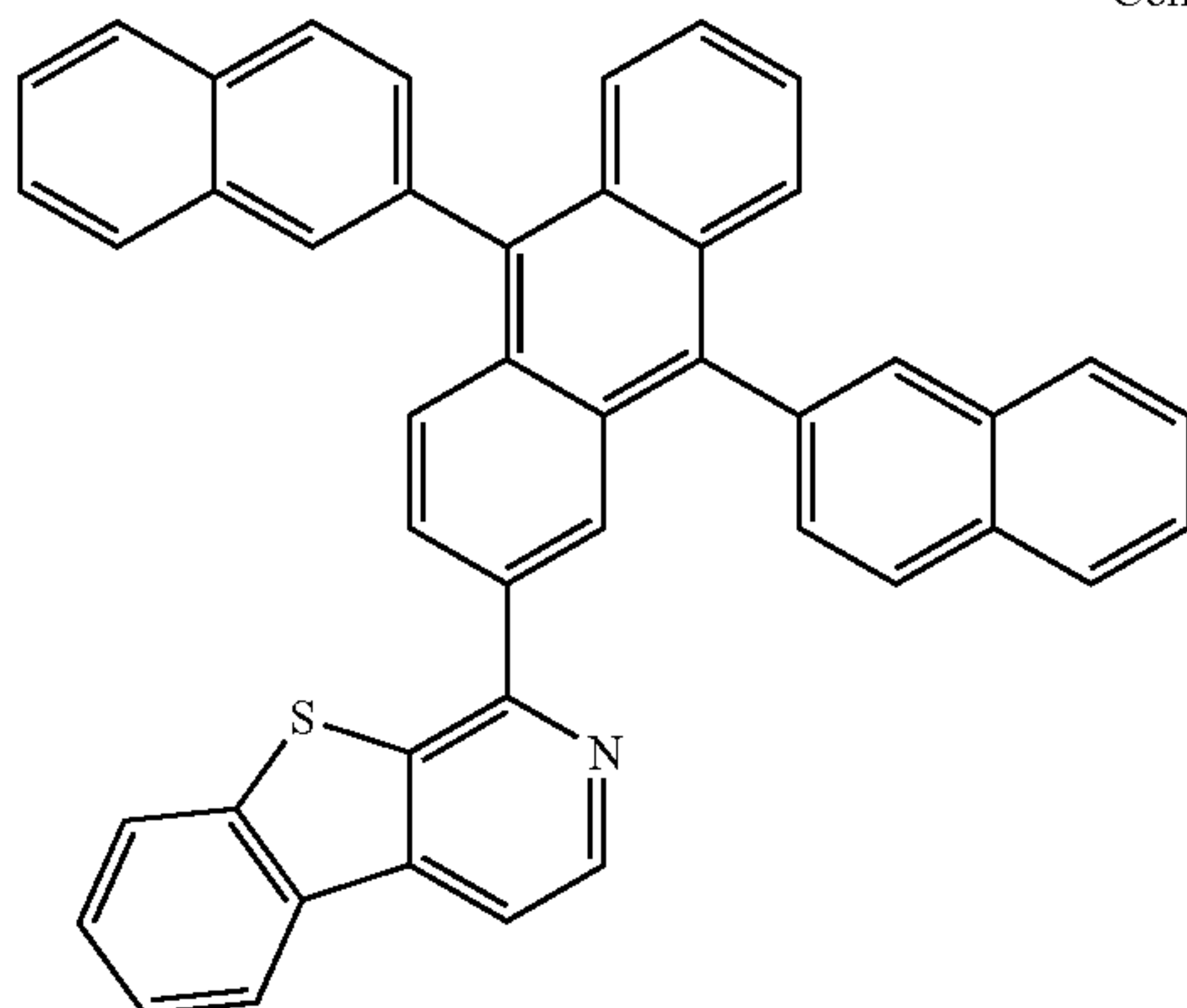
Compound 8
