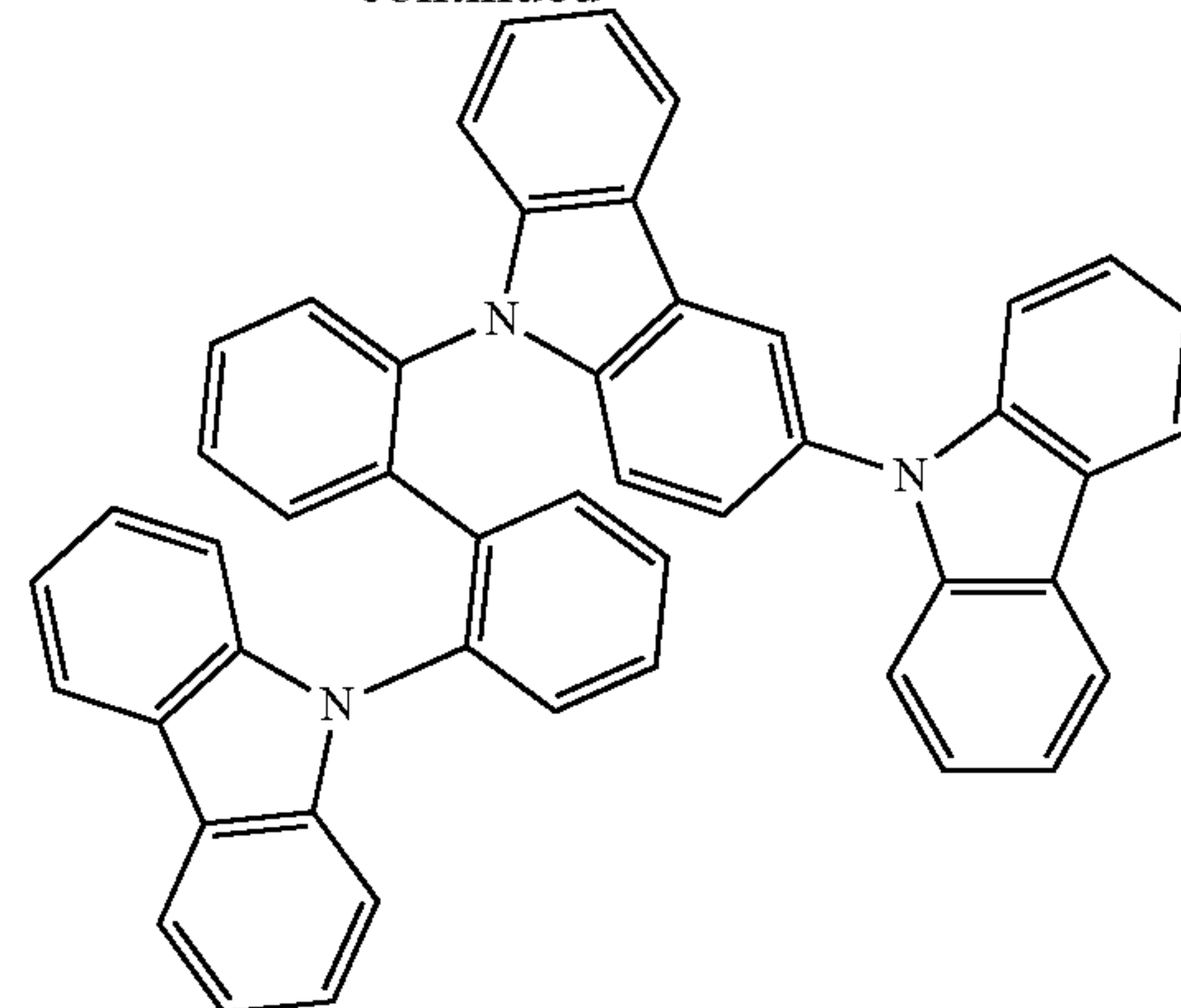
Compound A
