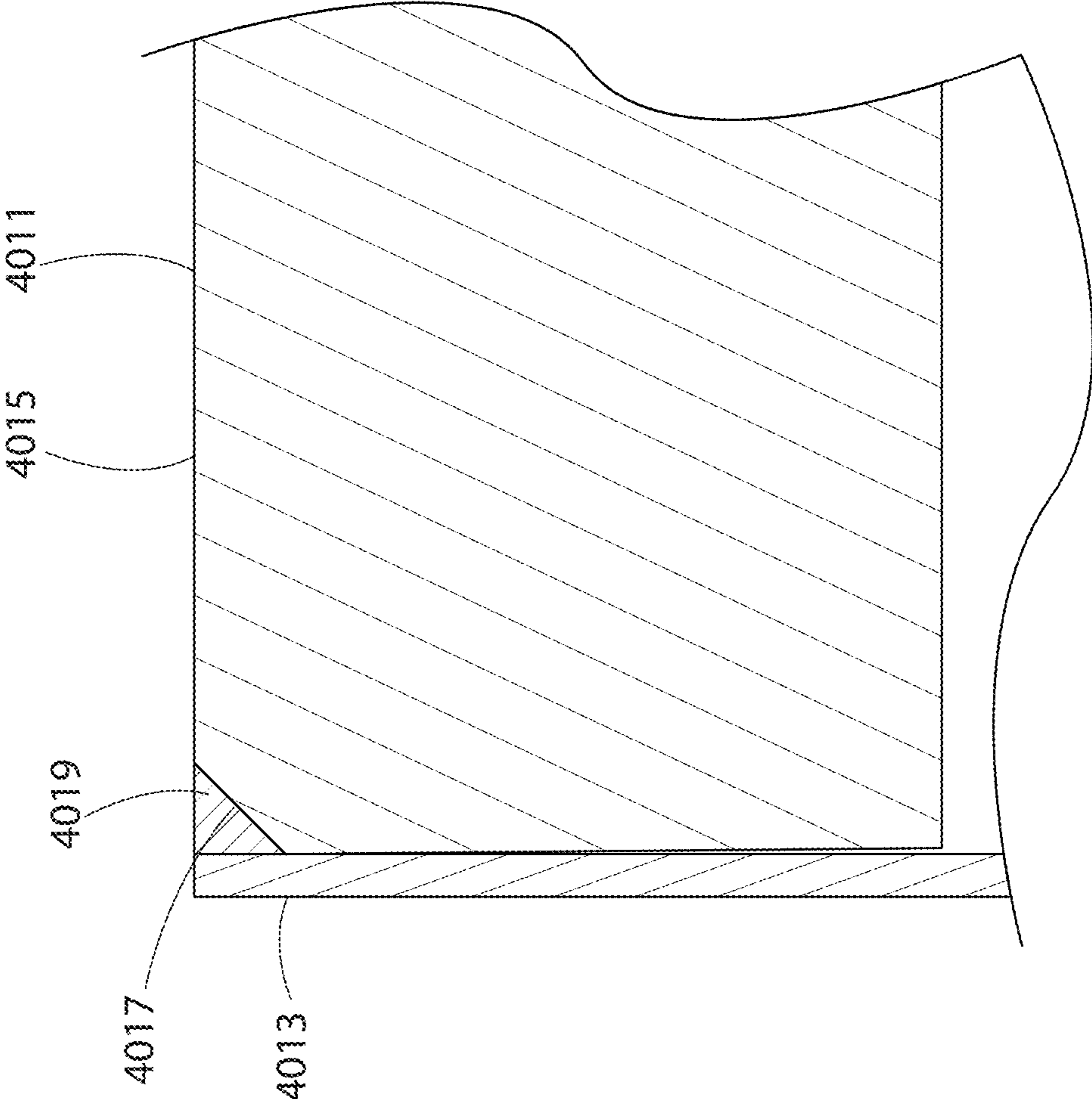
FIG. 48 (PRIOR ART)
