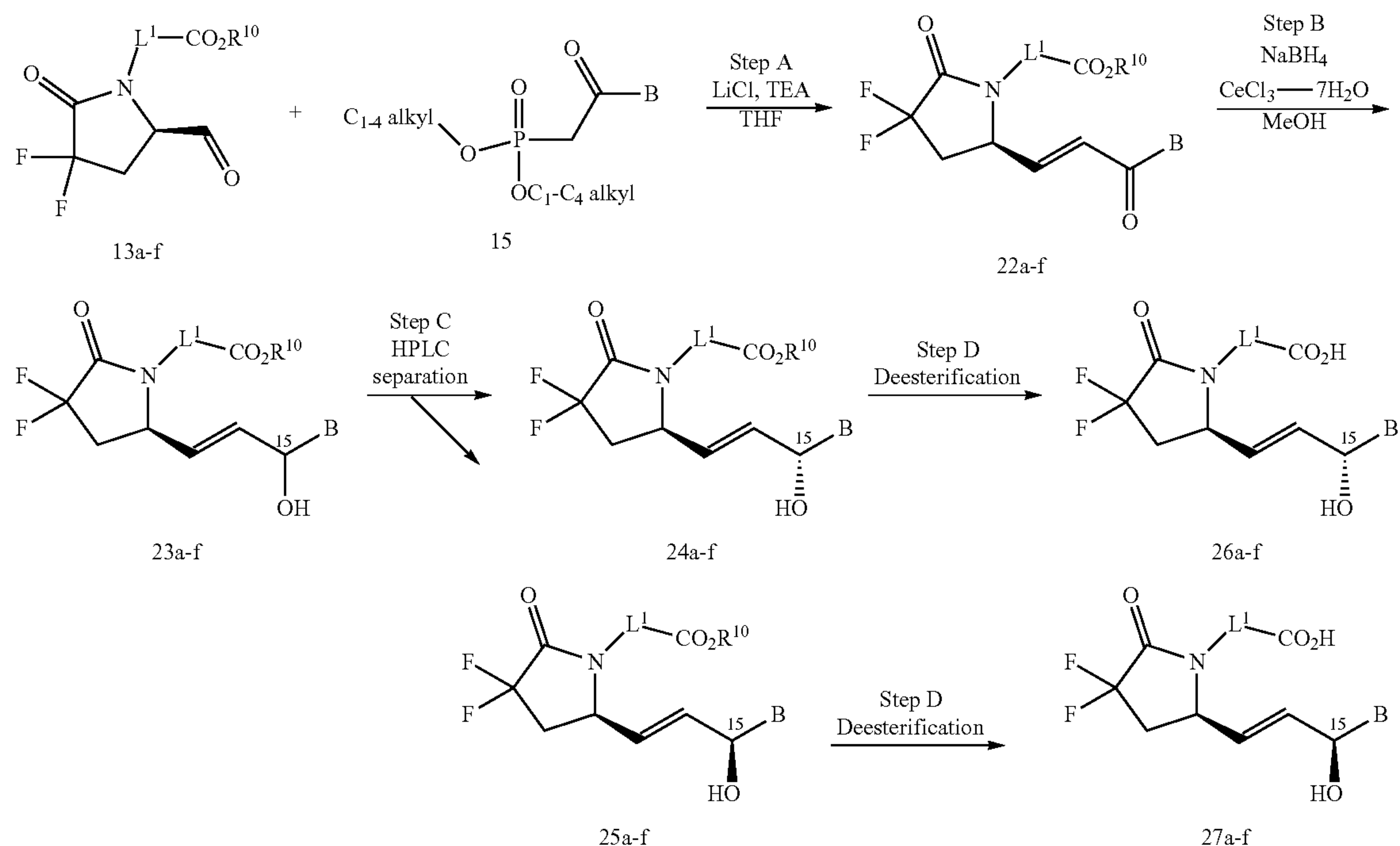
Scheme 9
