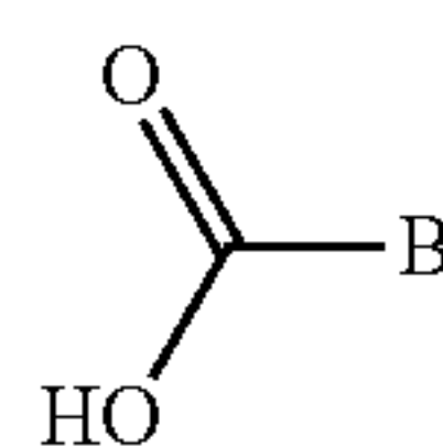
Carboxylic Acids 20
