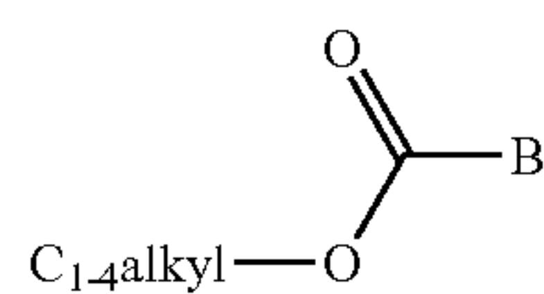
Carboxylic Esters 14
