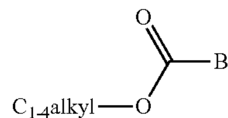
Carboxylic Esters 14
