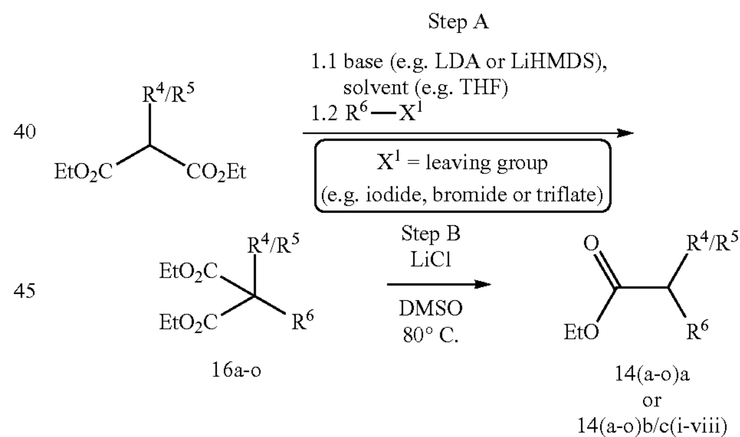
Scheme 7a
