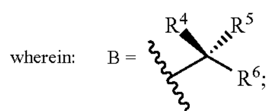
(S)-3-(B-Carbonyl)- 4-benzyloxazolidin- 2-ones
