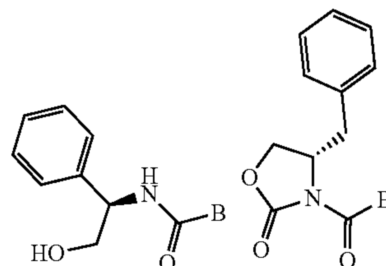
Amides 19
