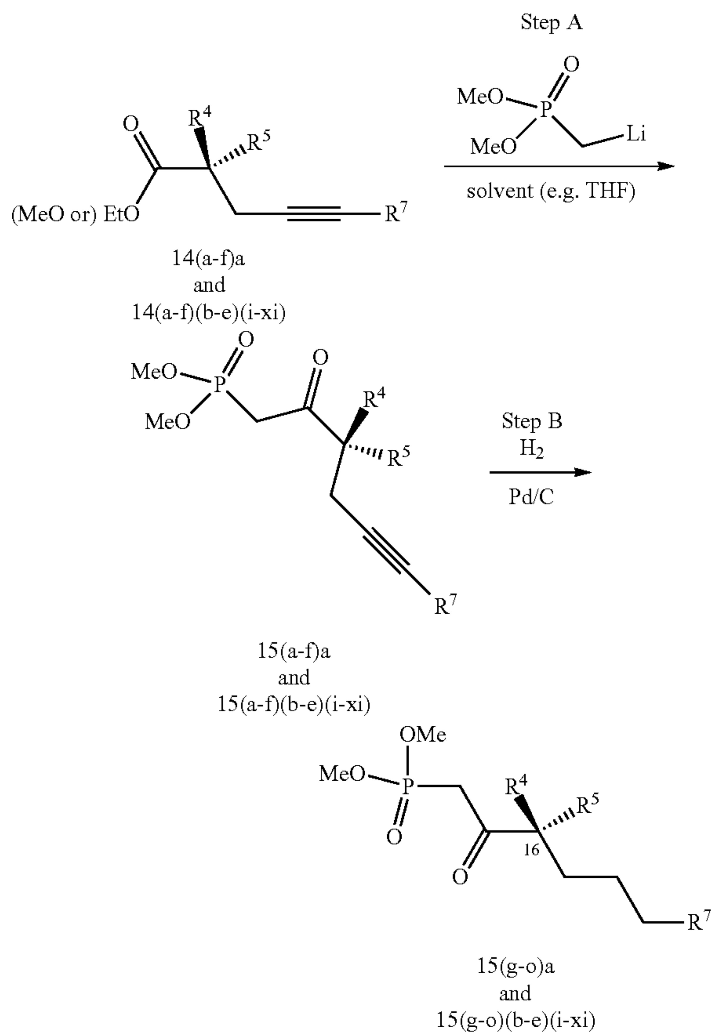
Scheme 8
