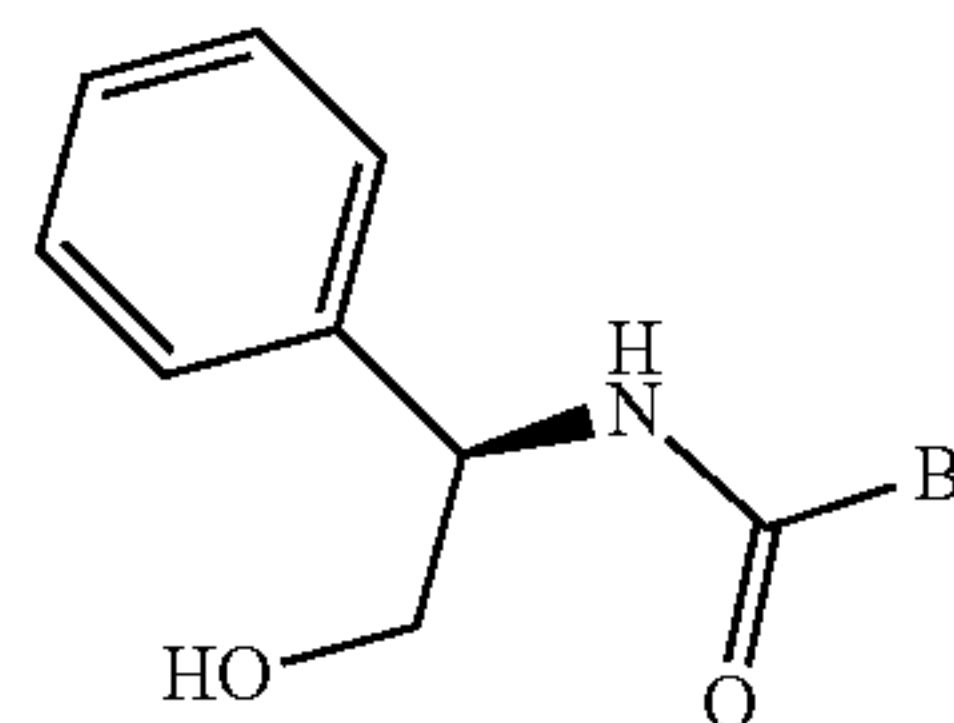
Amides
