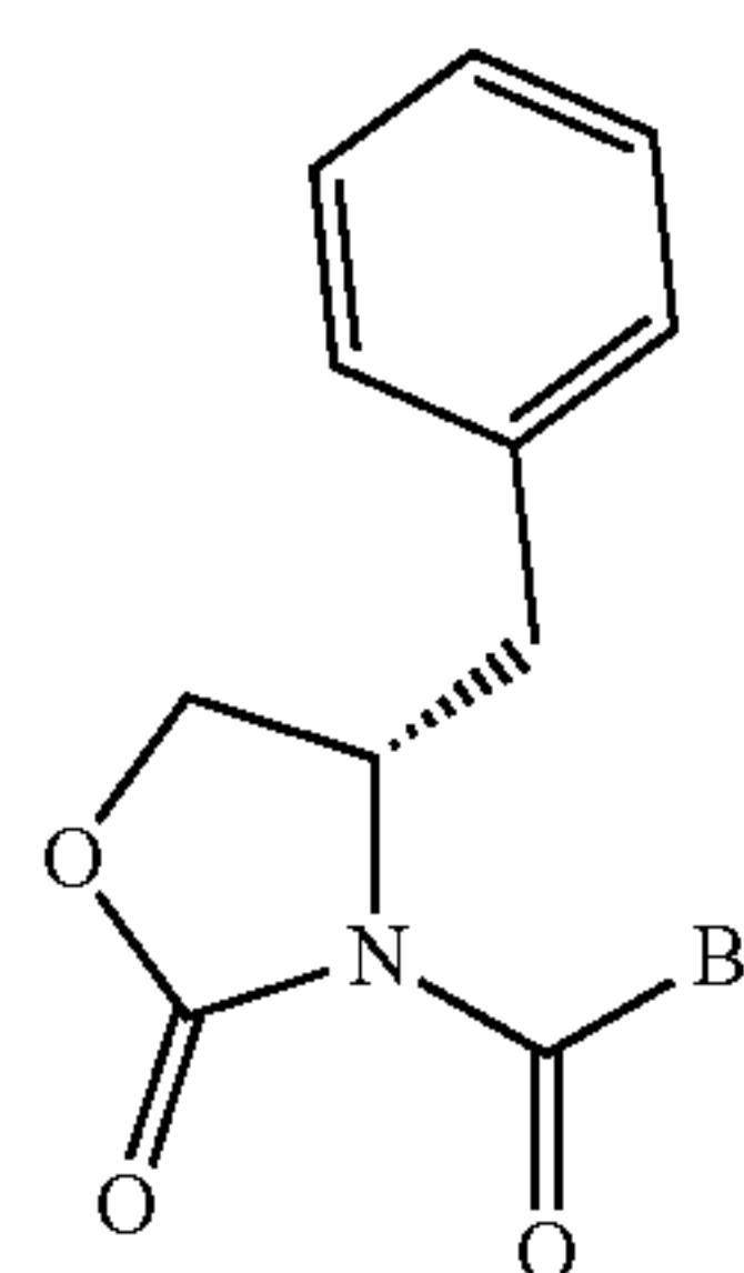
(S)-3-(B-Carbonyl)- 4-benzyloxazolidin- 2-ones
