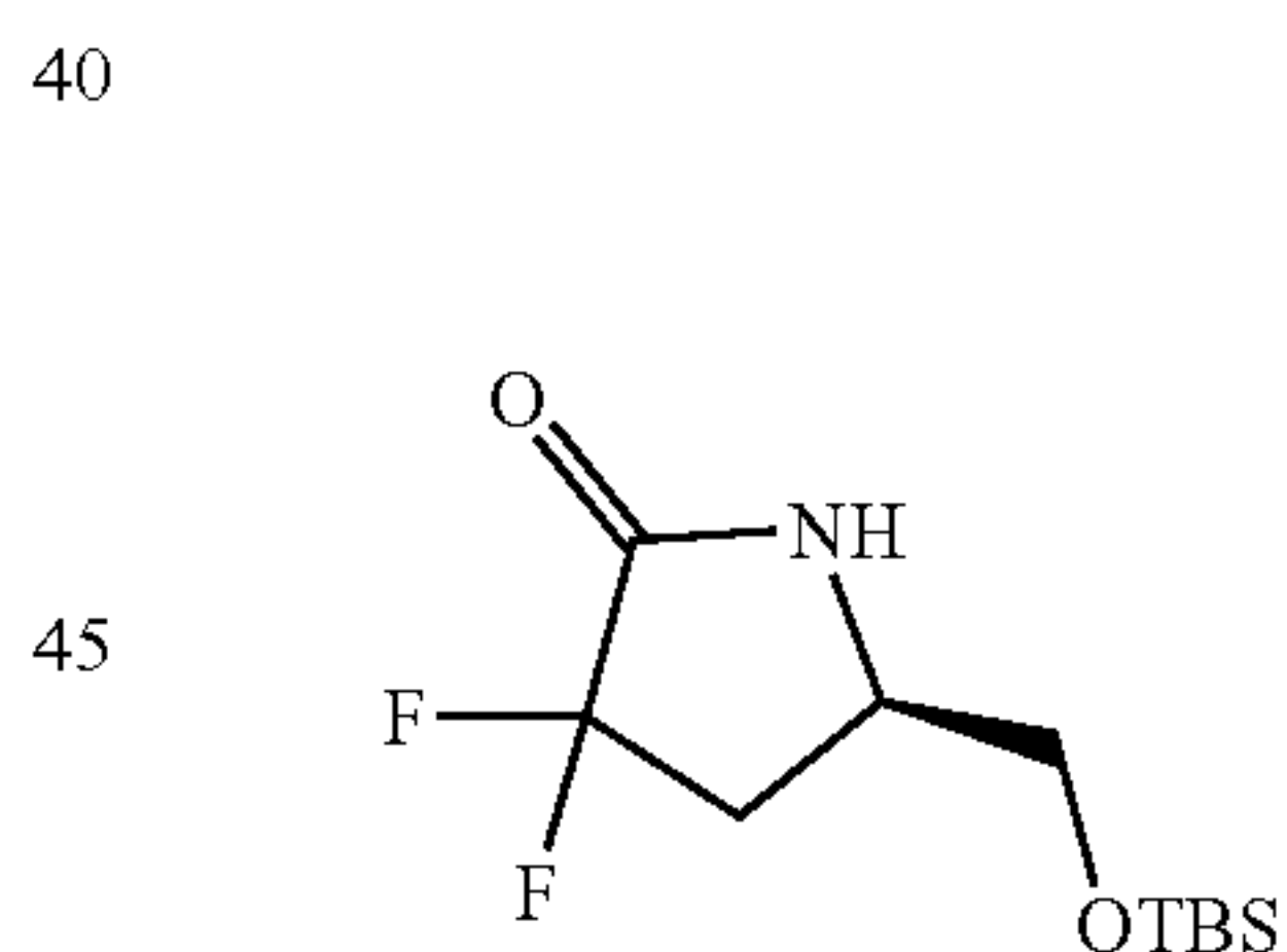
Scheme 3, Step H: Preparation of (R)-5-(((tert-butyl)dimethylsilyloxy)methyl)-3,3-difluoropyrrolidin-2-one (9; PG=TBS)
