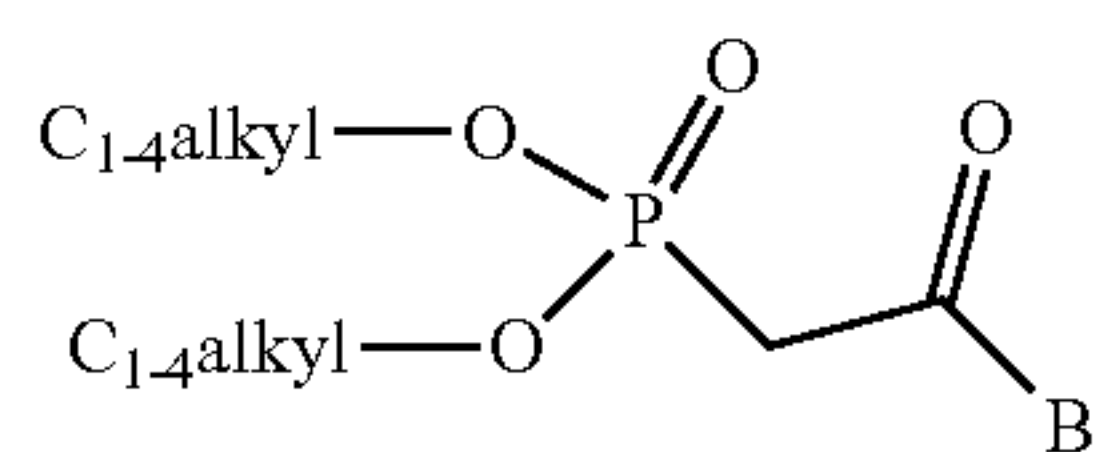
\beta -Keto Phosphonate Esters 15
