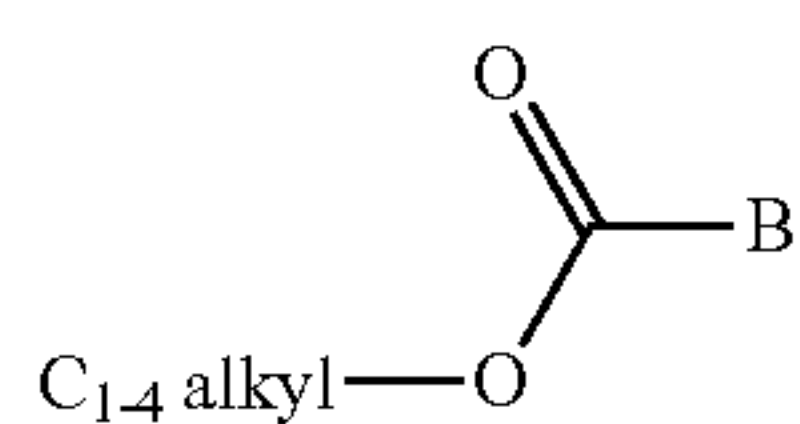
Carboxylic Esters
