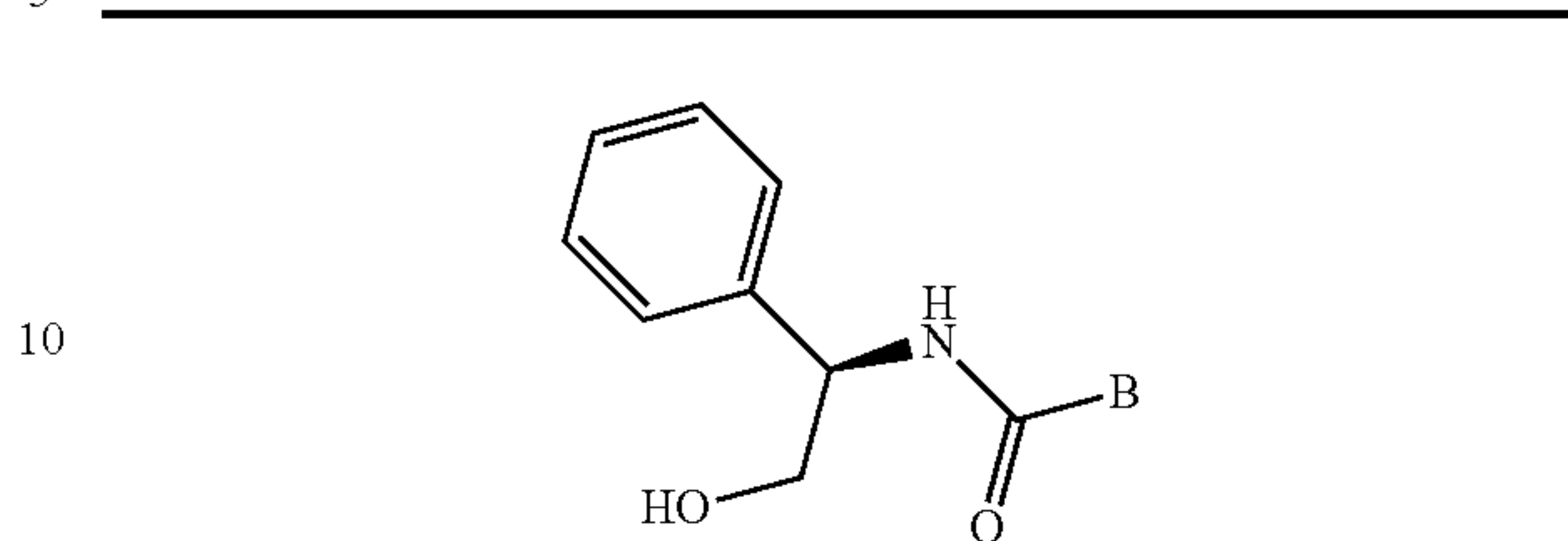
Amides 19
