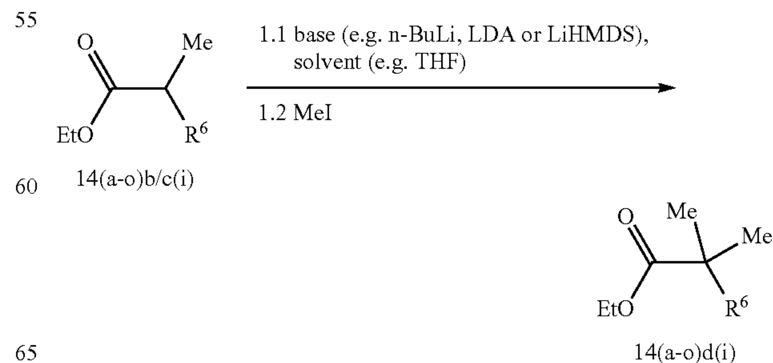
Scheme 7b
