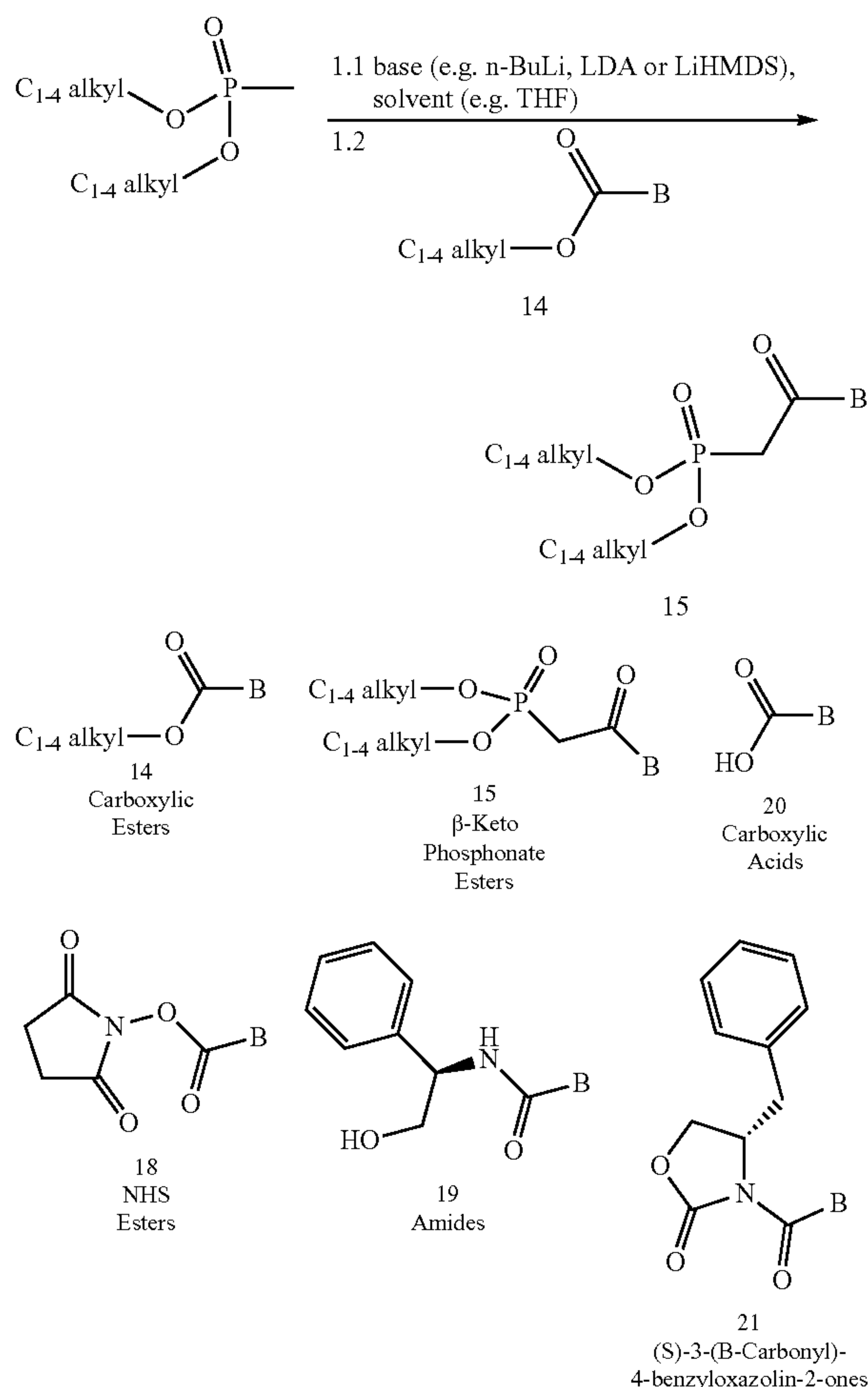
Scheme 6
