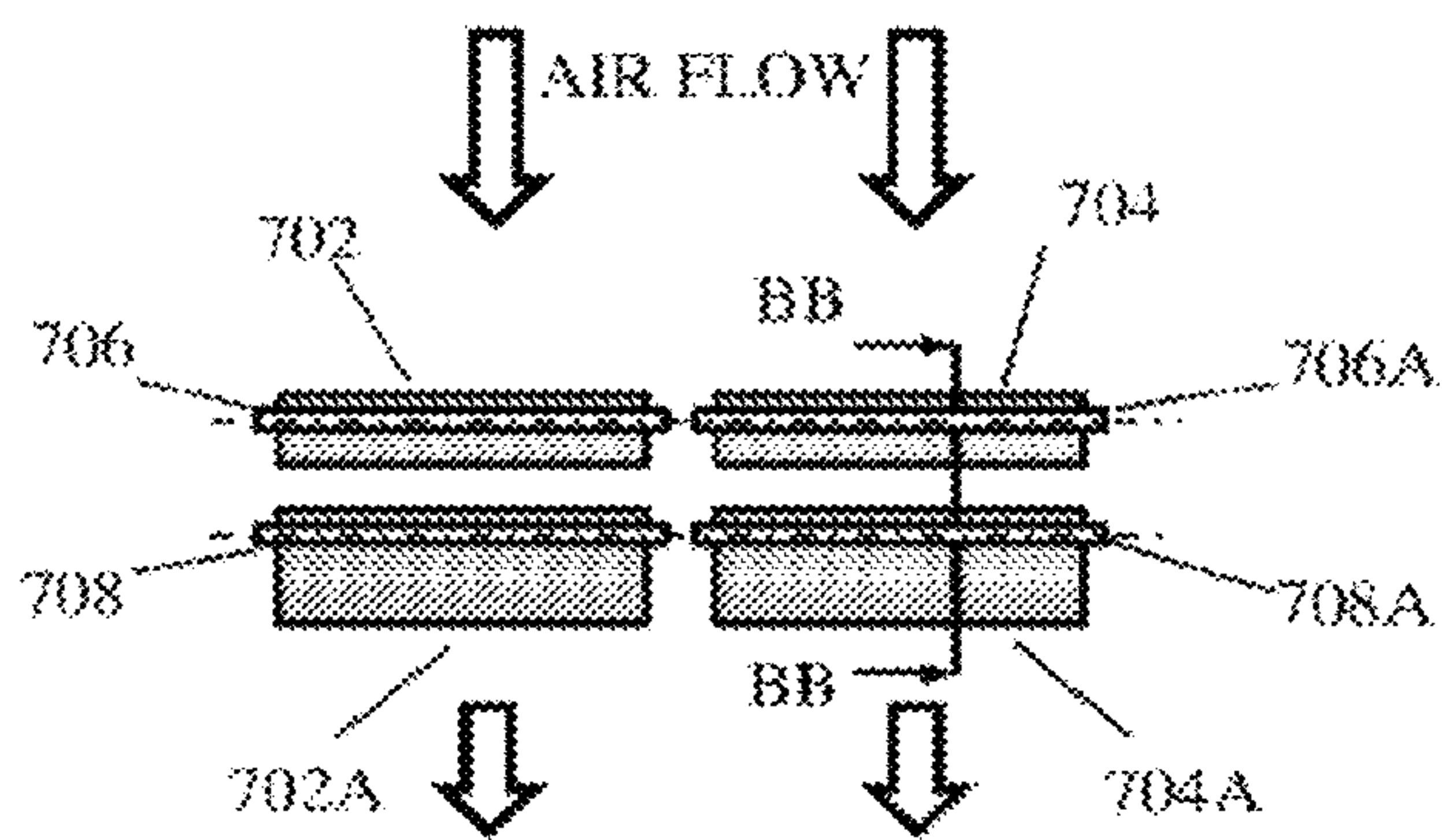
Fig. 7B CROSS SECTION AA
