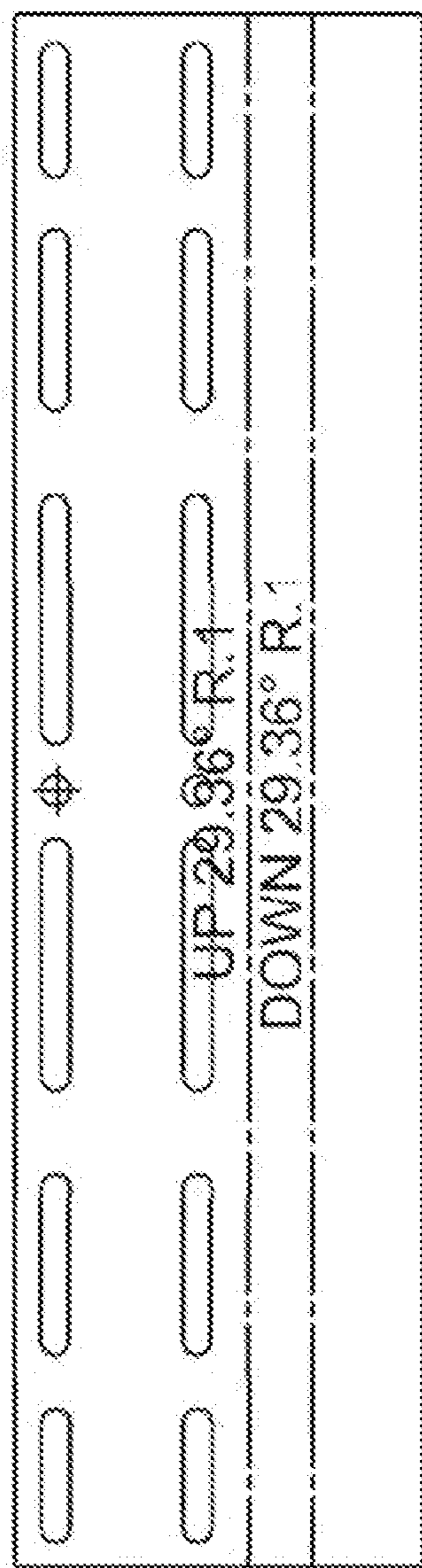
FLAT PATTERN
