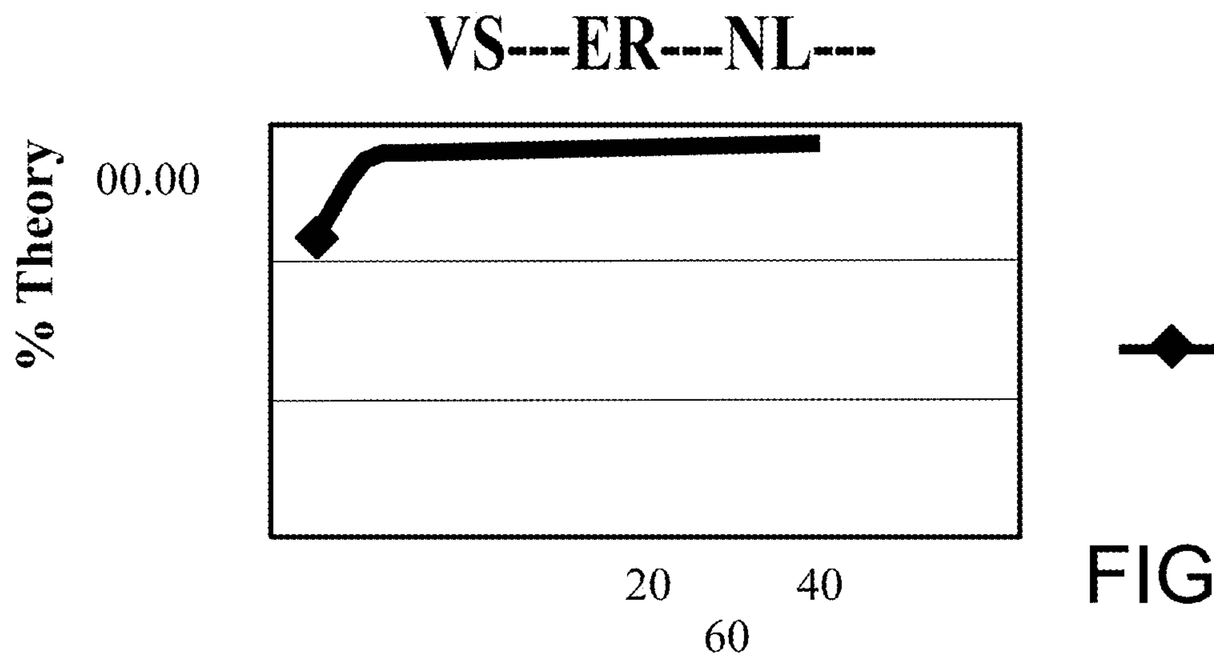
Graph of Dissolution Test Results for VS-ER-NL-55F-D (1.5% BC)
