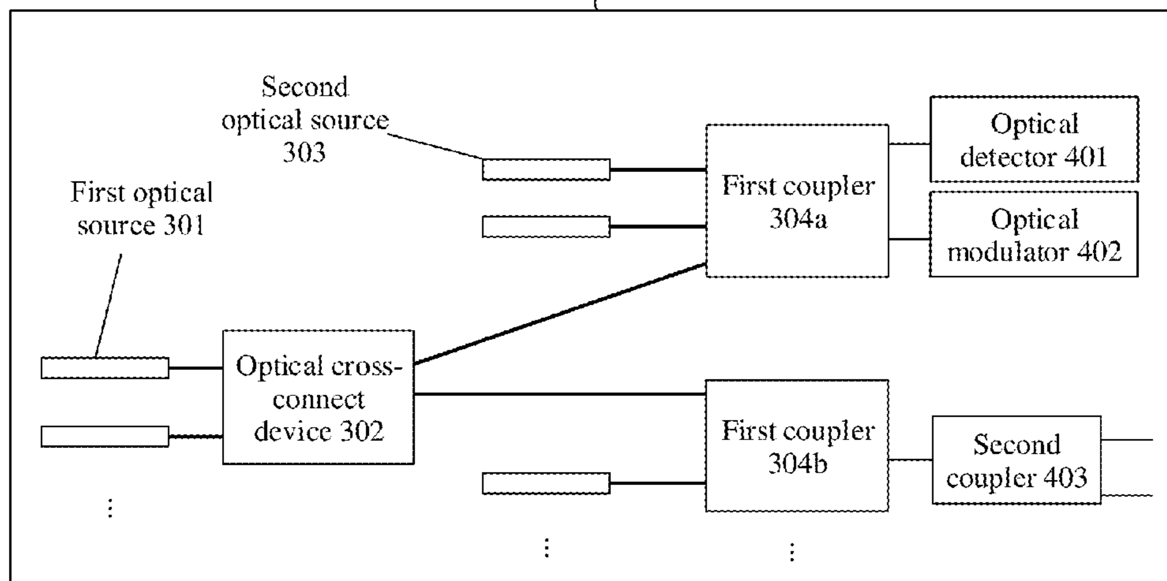
Optical source switching apparatus 400
