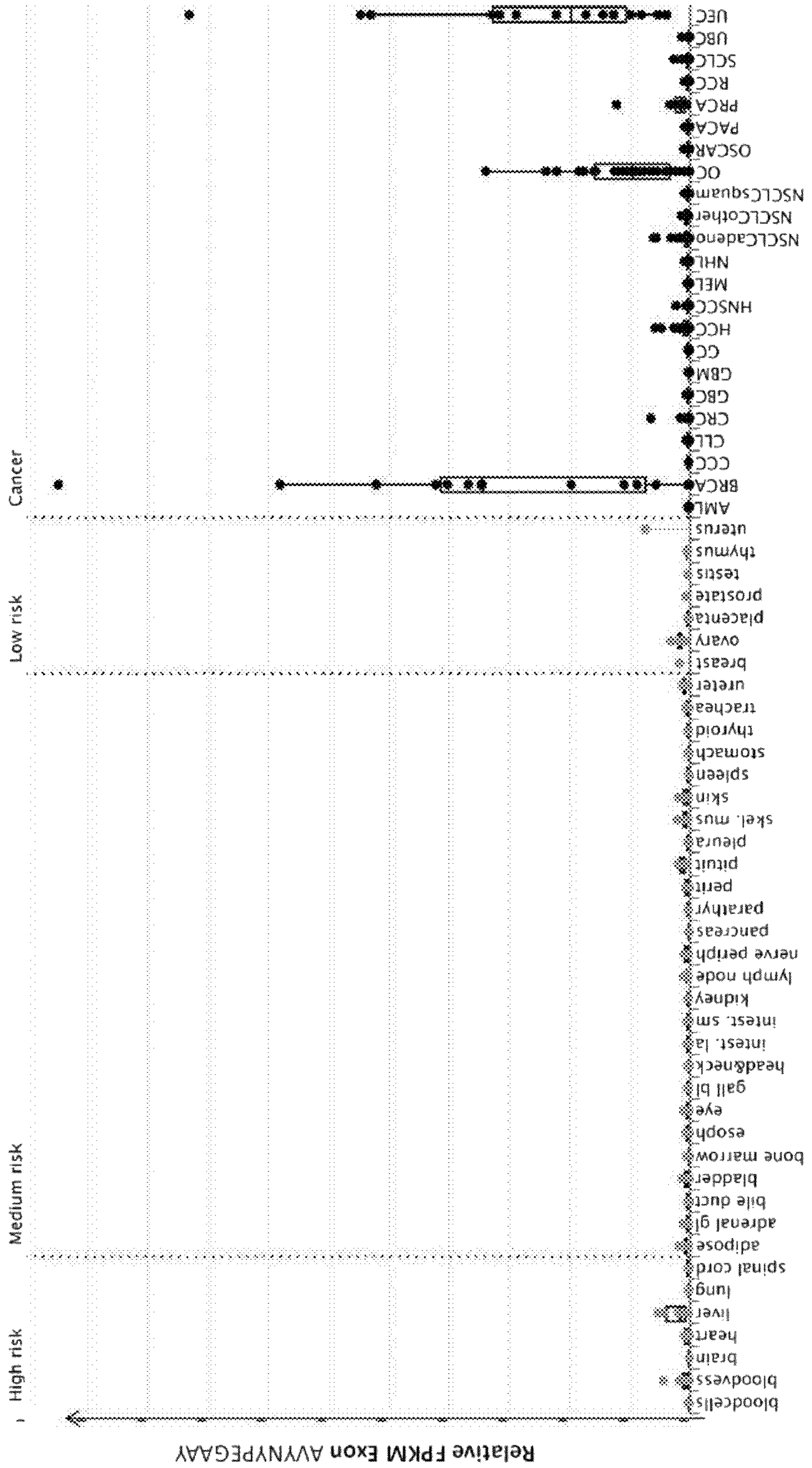
Figure 2X Gene: ESR1 Peptide: AVYNYPEGAAY SEQ ID NO: 252
