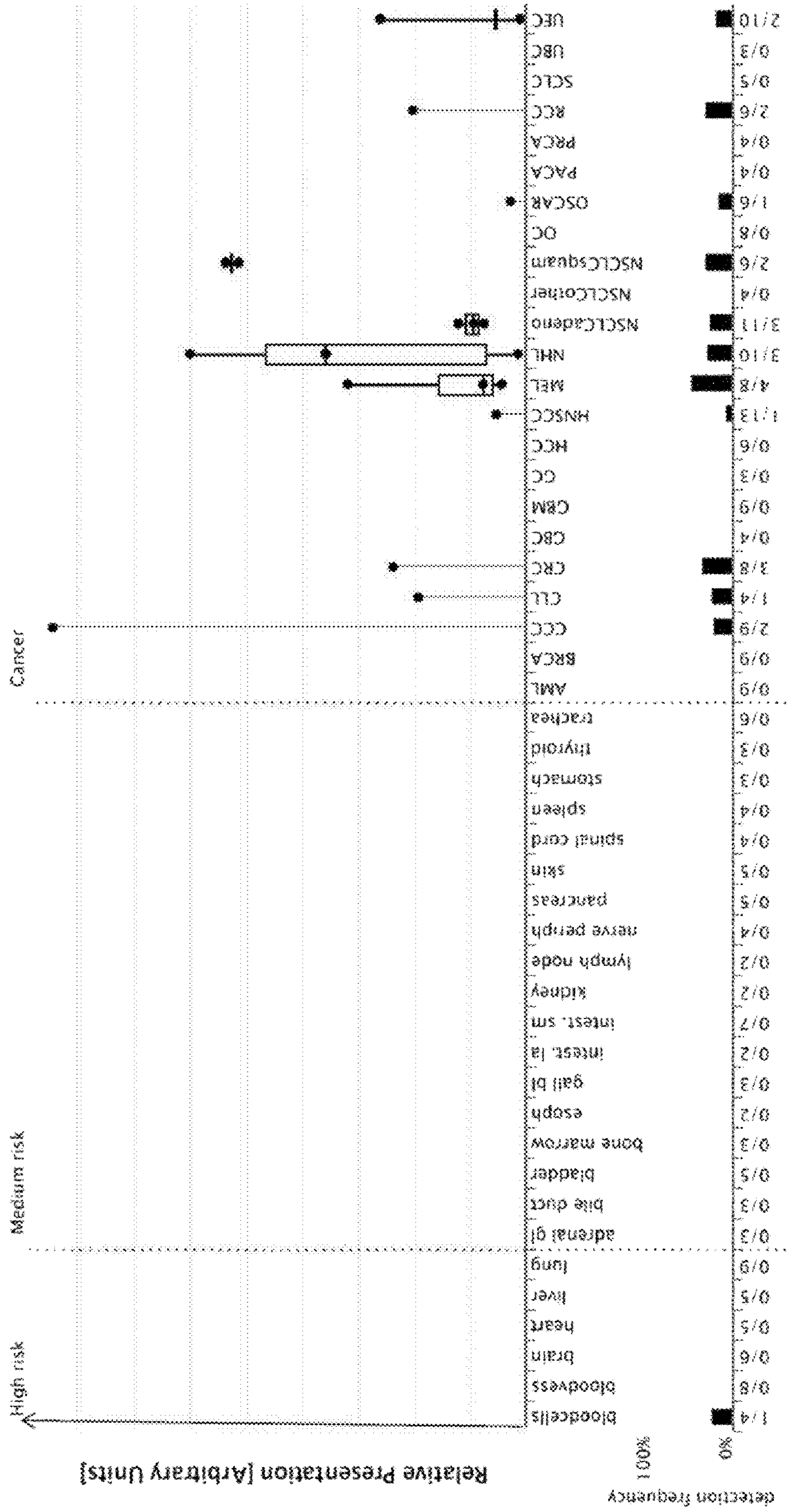
Figure 1F Peptide: AVAAVLLSR (A*03) SEQ ID NO: 79
