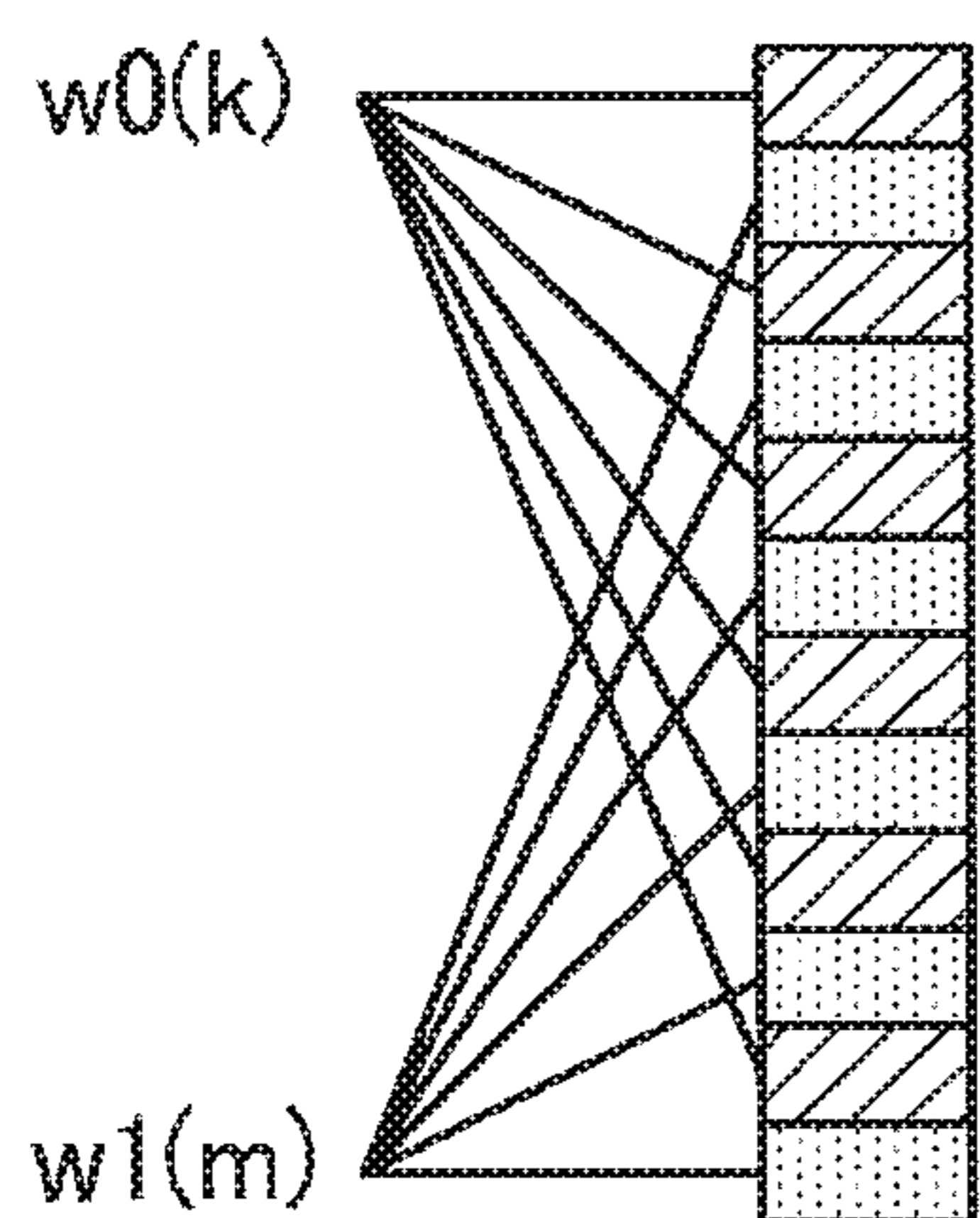
Secondary synchronization channel of slot 0
