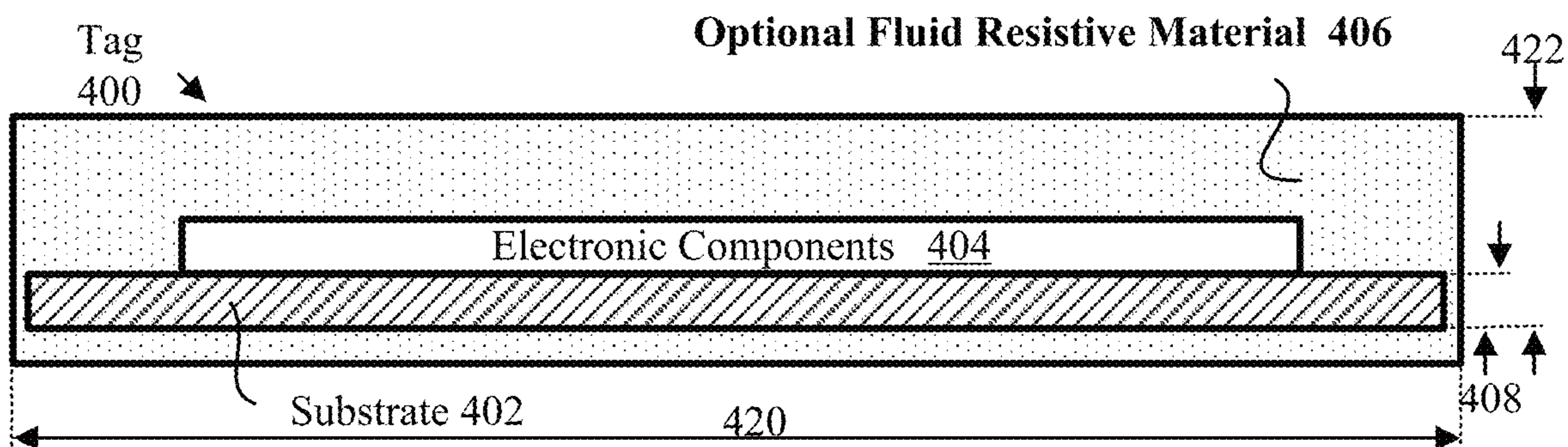
FIG. 4 (Side View)
