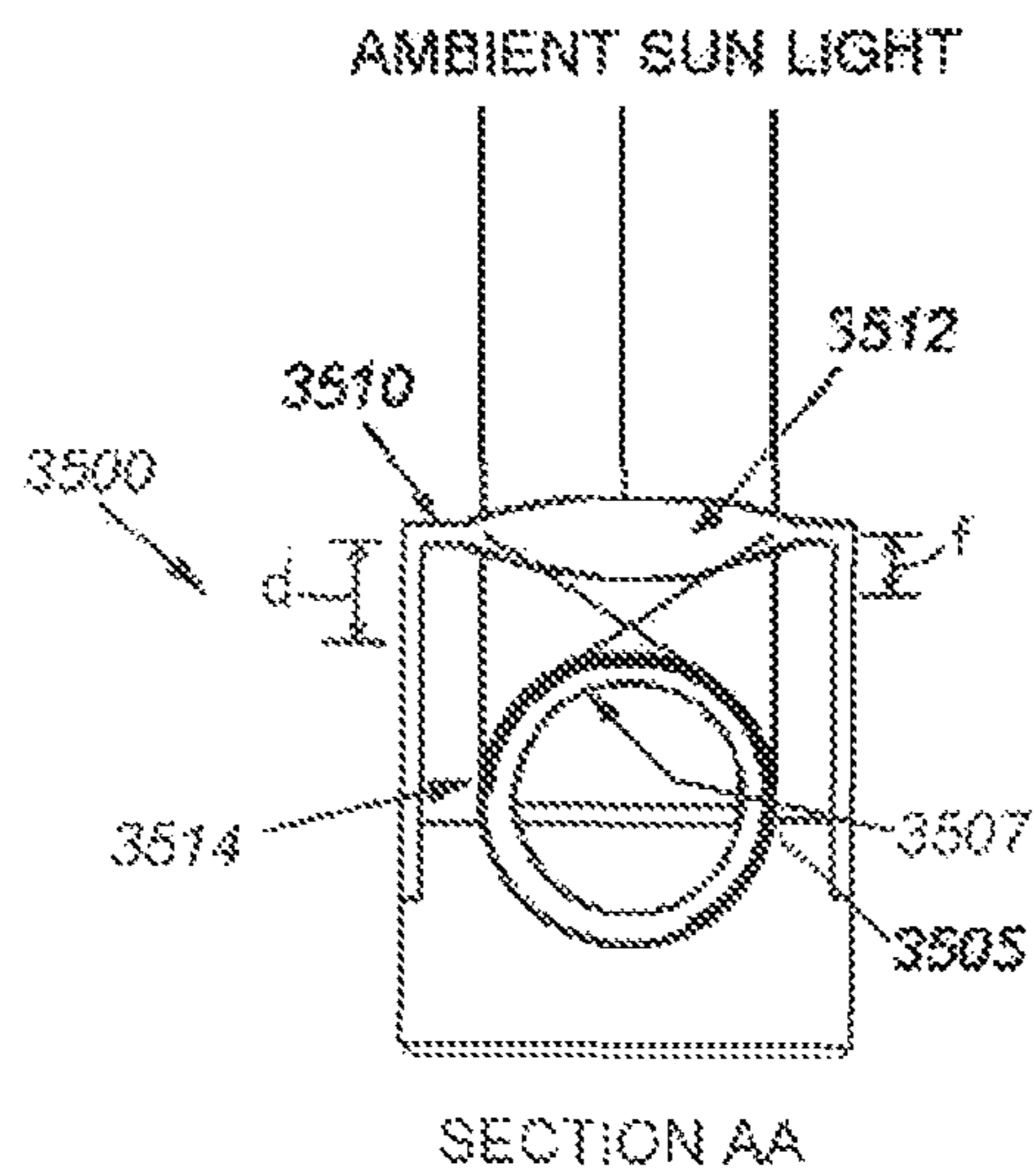
SECTION AA FIG. 35C
