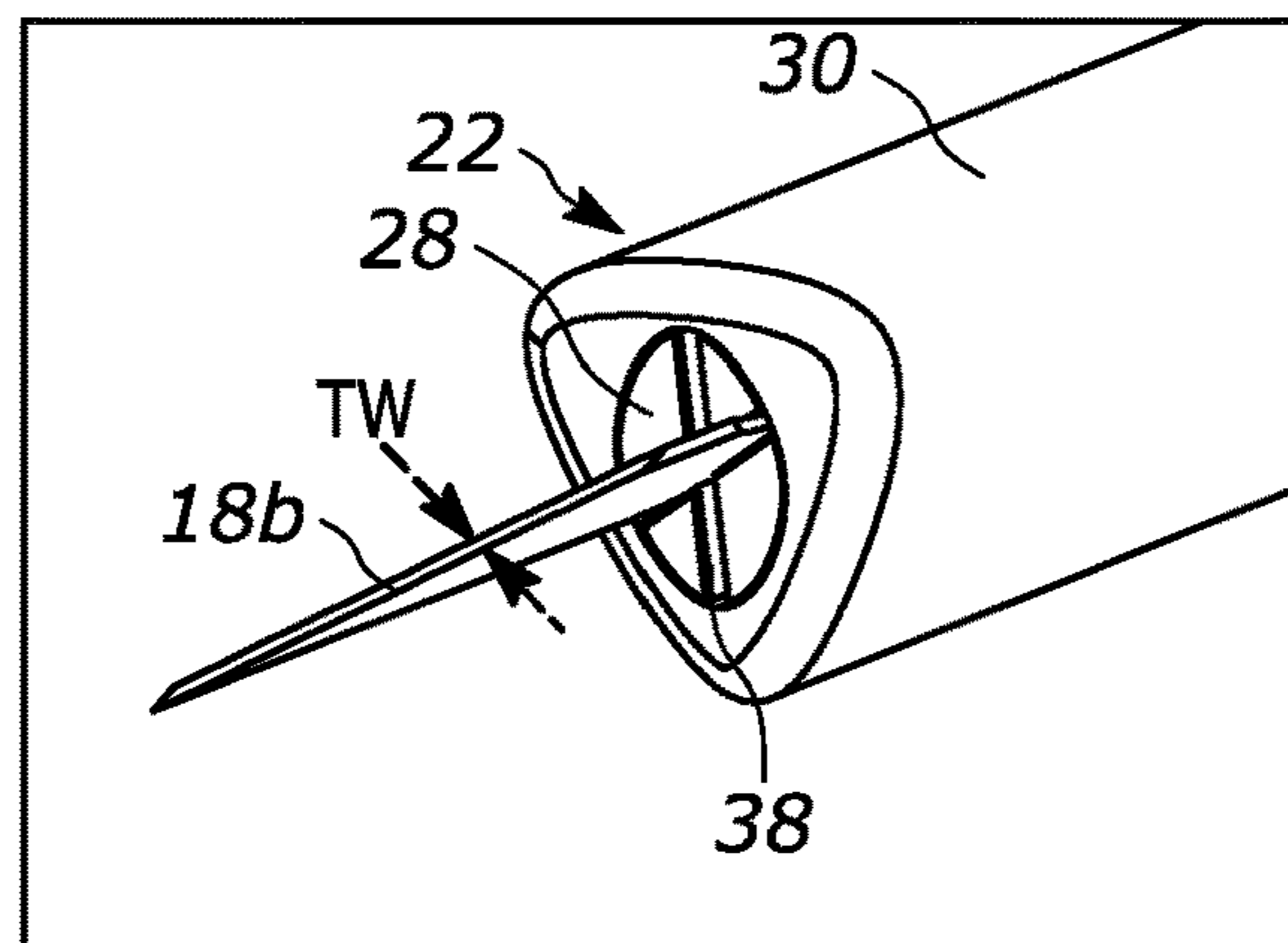
Collet With #11 Blade
