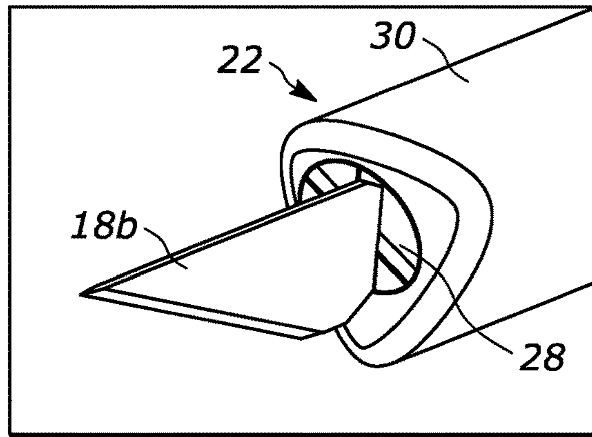
Collet With #11 Blade (View 2)
