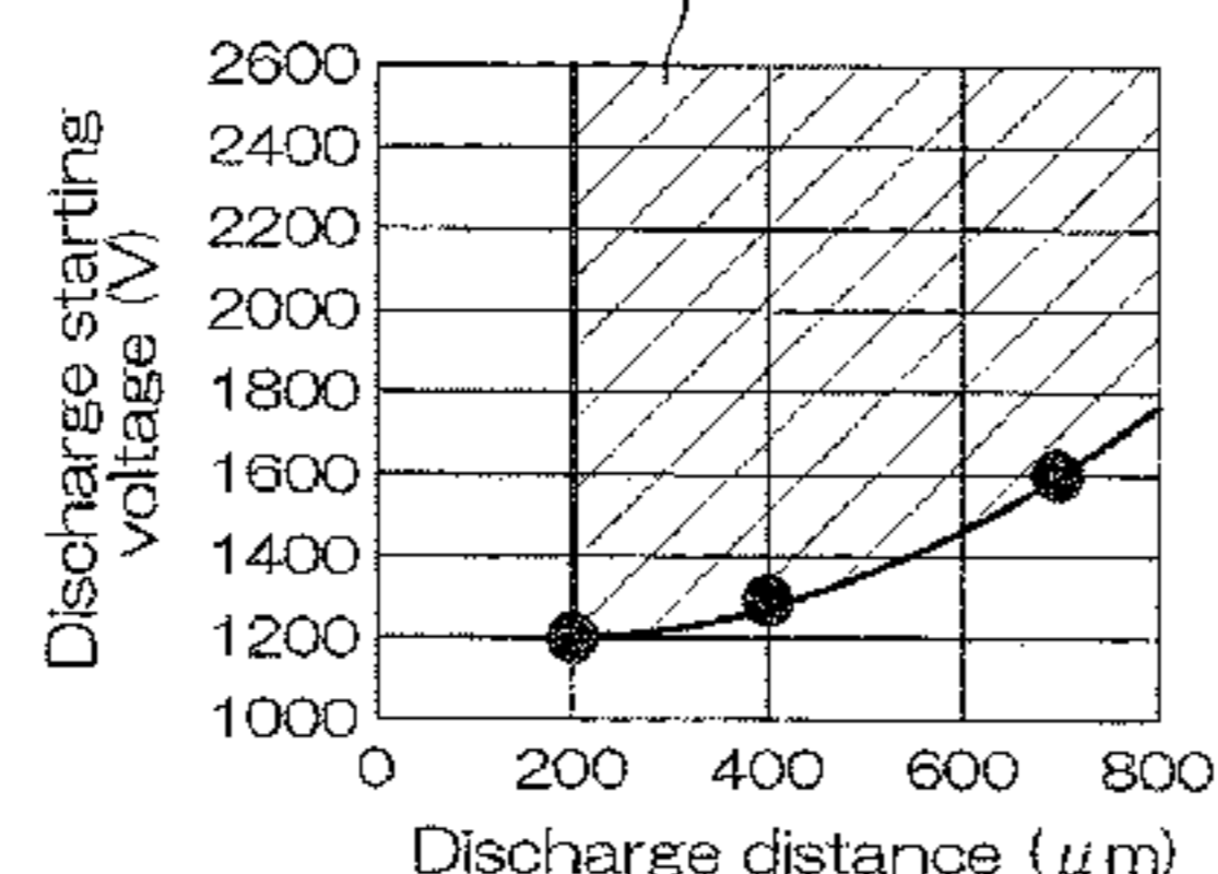
(a) Region with the possibility of occurrence of discharge
