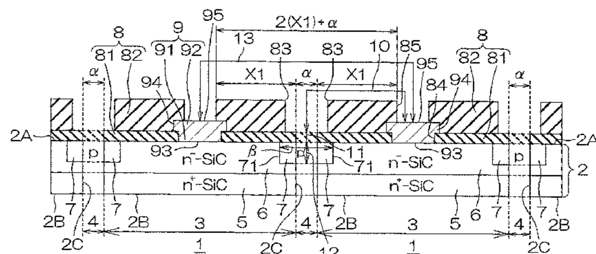
(a) Region with the possibility of occurrence of discharge
