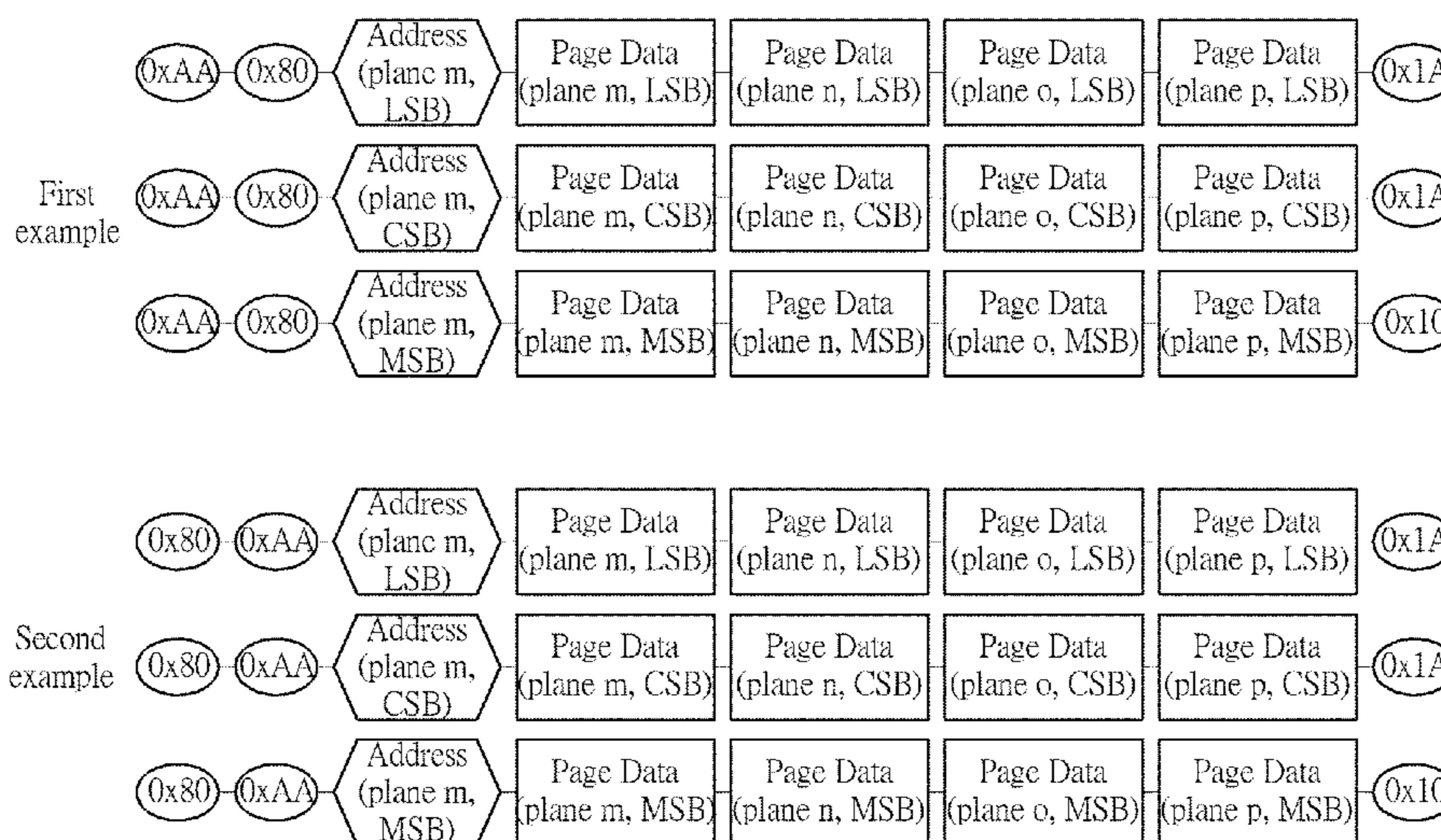
Flash memory controller send command for write operation
