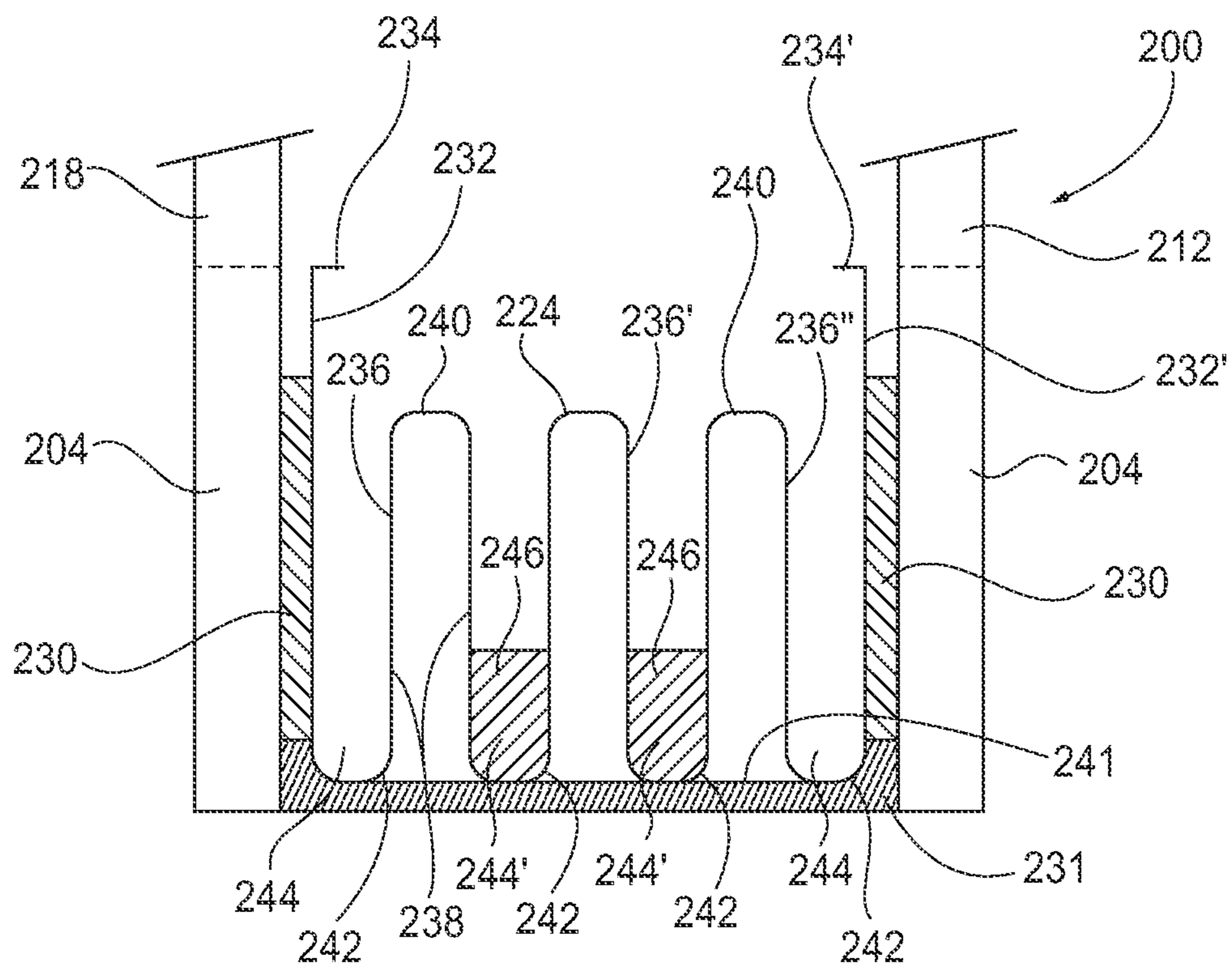
FIG. 3D
