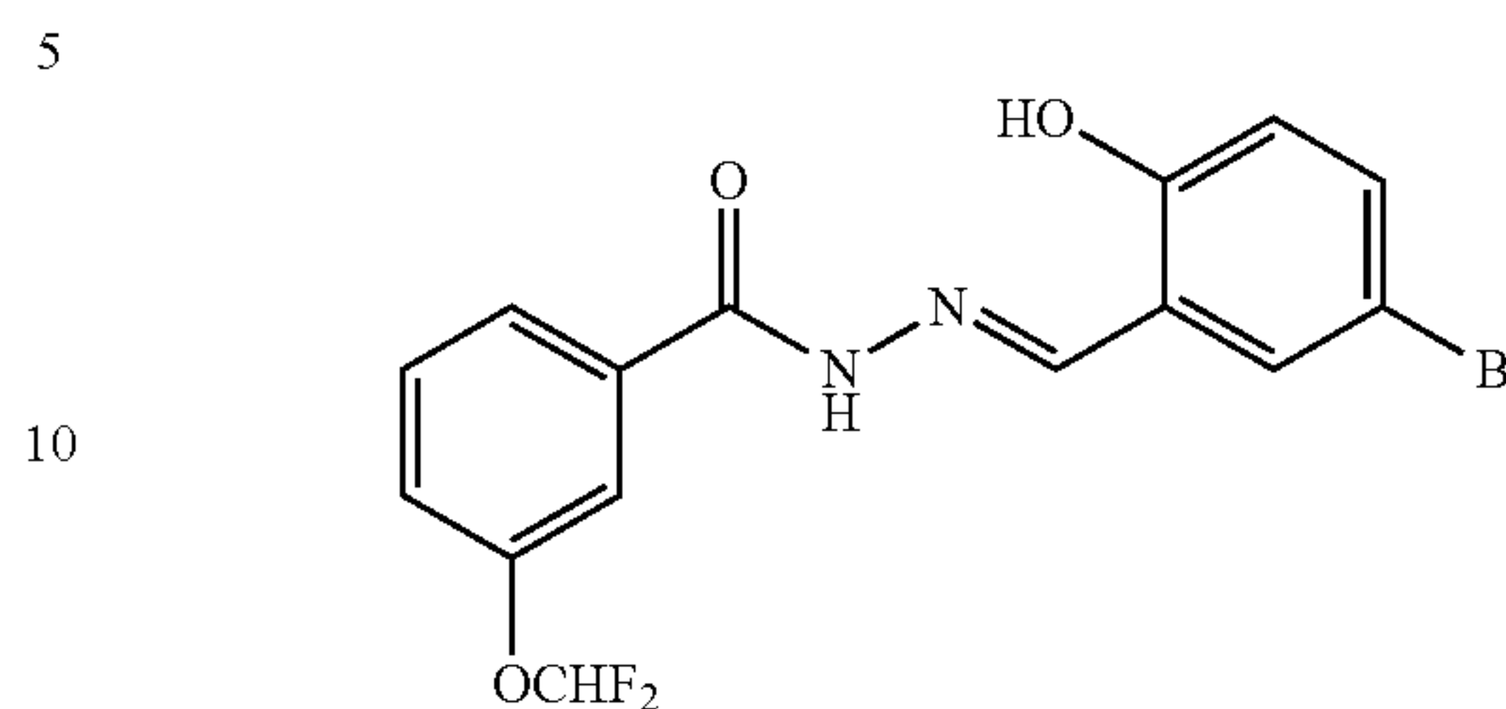
3-Difluoromethoxy-N'-(5-bromo-2-hydroxybenzylidene)benzohydrazide (A5)
