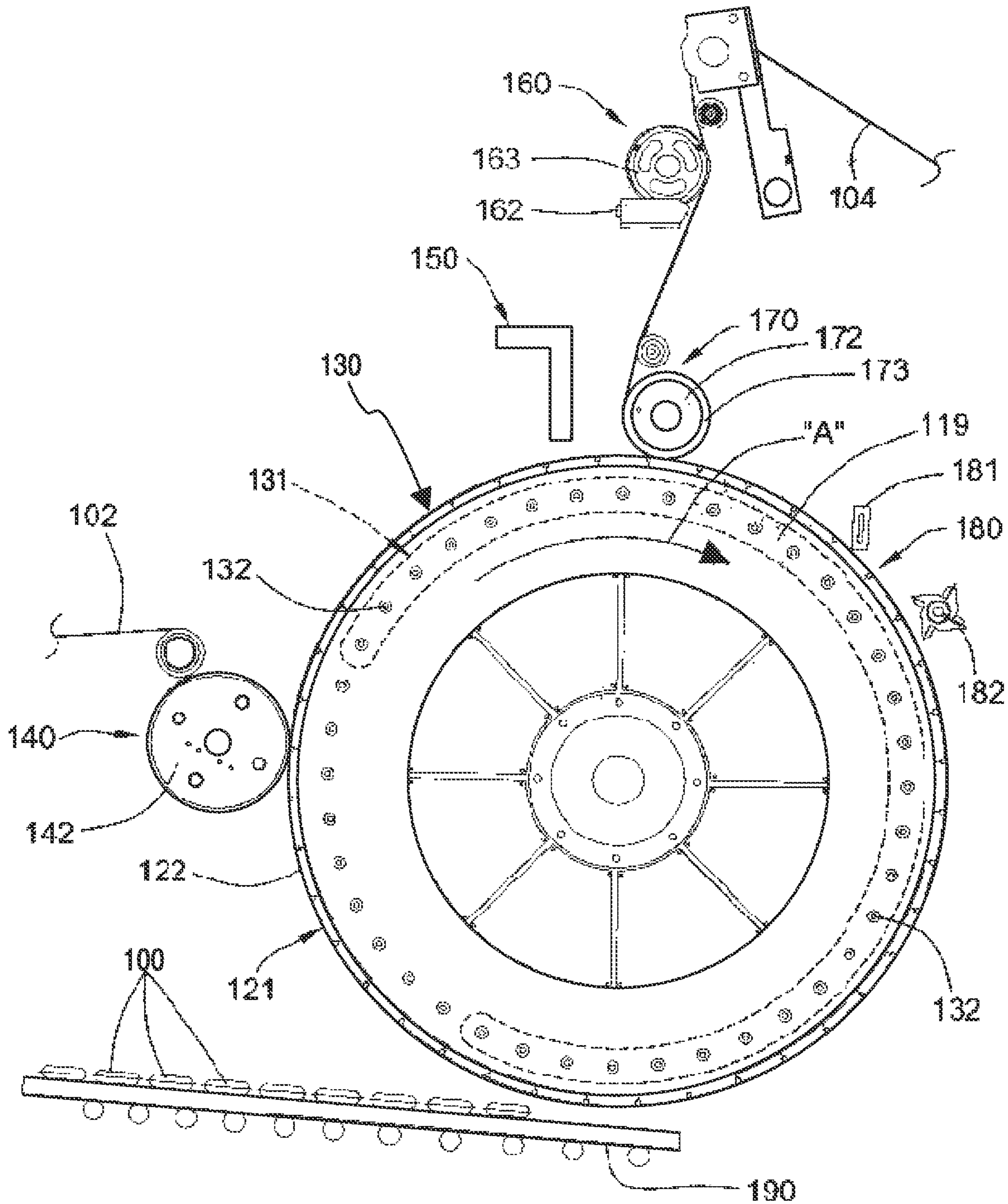
FIG. 5 PRIOR ART
